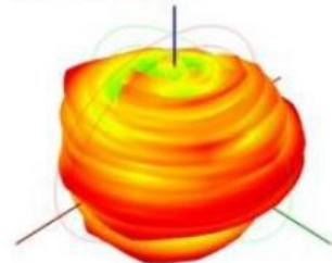
57400MH2 H+V,BT 65.4%
