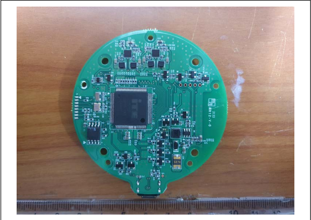
MainBoard-Rear
