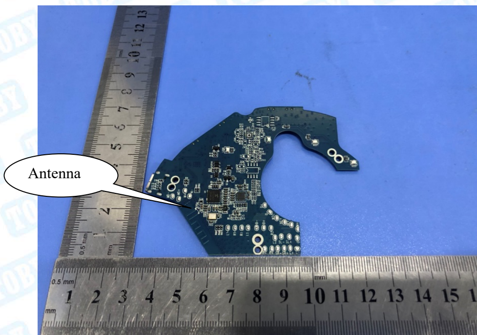
Photo 12 Internal of PCB
