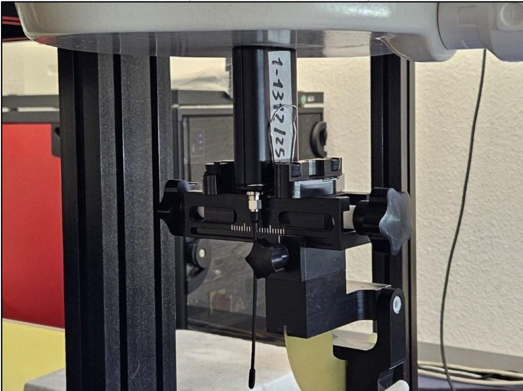
Photo 10: Test position bottom side without any distance
