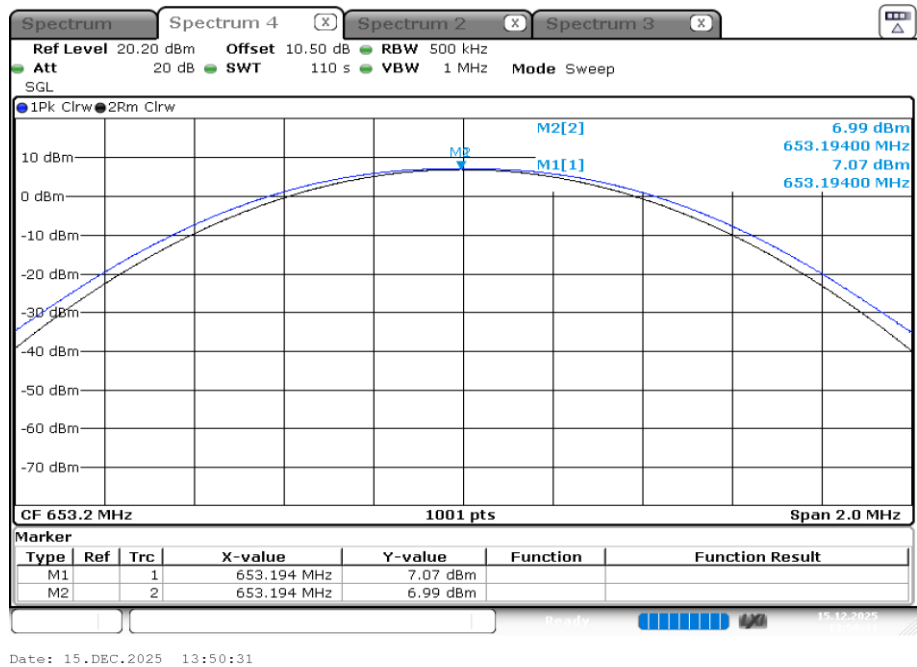
Plot 1: lowest channel, 653.2 MHz average (modulated carrier)
