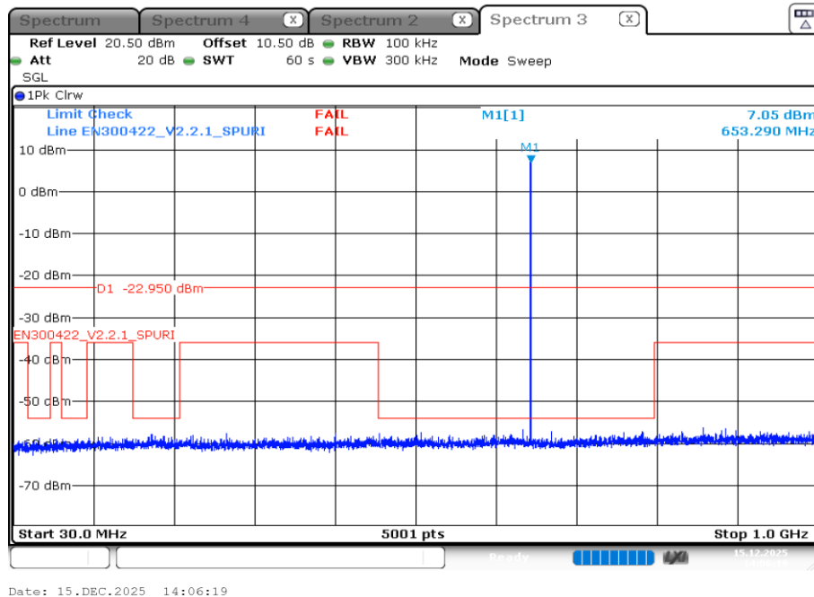
Plot 1: 653.2 MHz, 30MHz – 1 GHz
