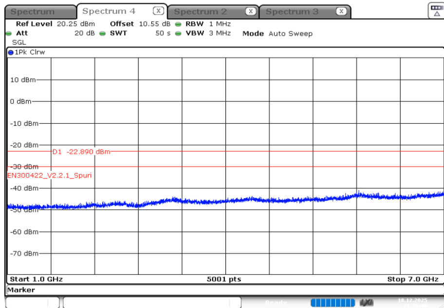
Plot 4: 656.8 MHz, 1 GHz – 7 GHz
