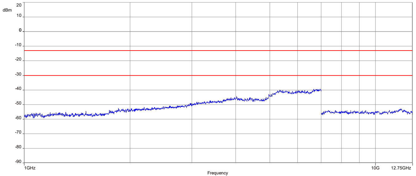
Plot 2: 656.8 MHz, spurious emissions, 1GHz - 12.75 GHz
