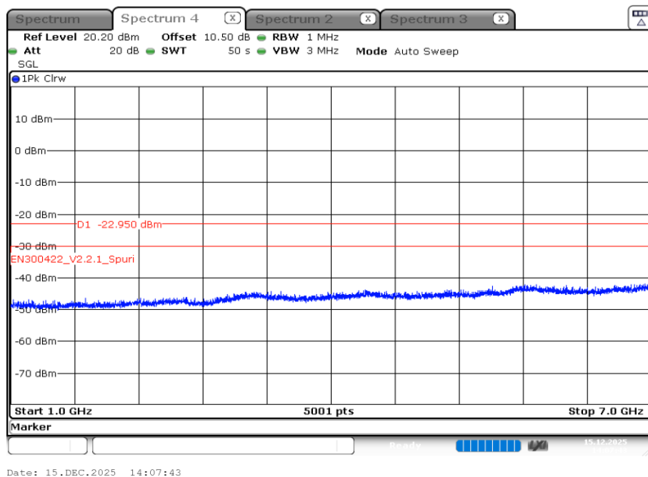
Plot 2: 653.2 MHz, 1 GHz – 7 GHz
