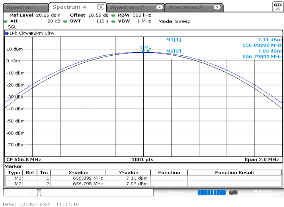
Plot 2: highest channel, 656.8 MHz, average (modulated carrier)
