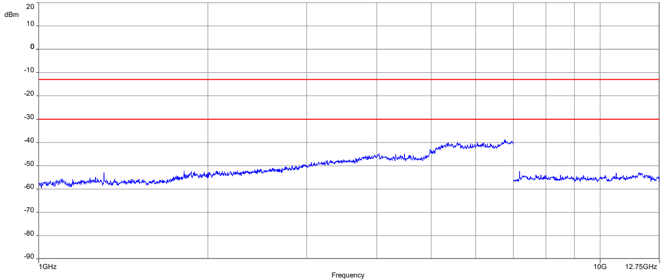
Plot 1: 653.2 MHz, spurious emissions, 1GHz - 12.75 GHz
