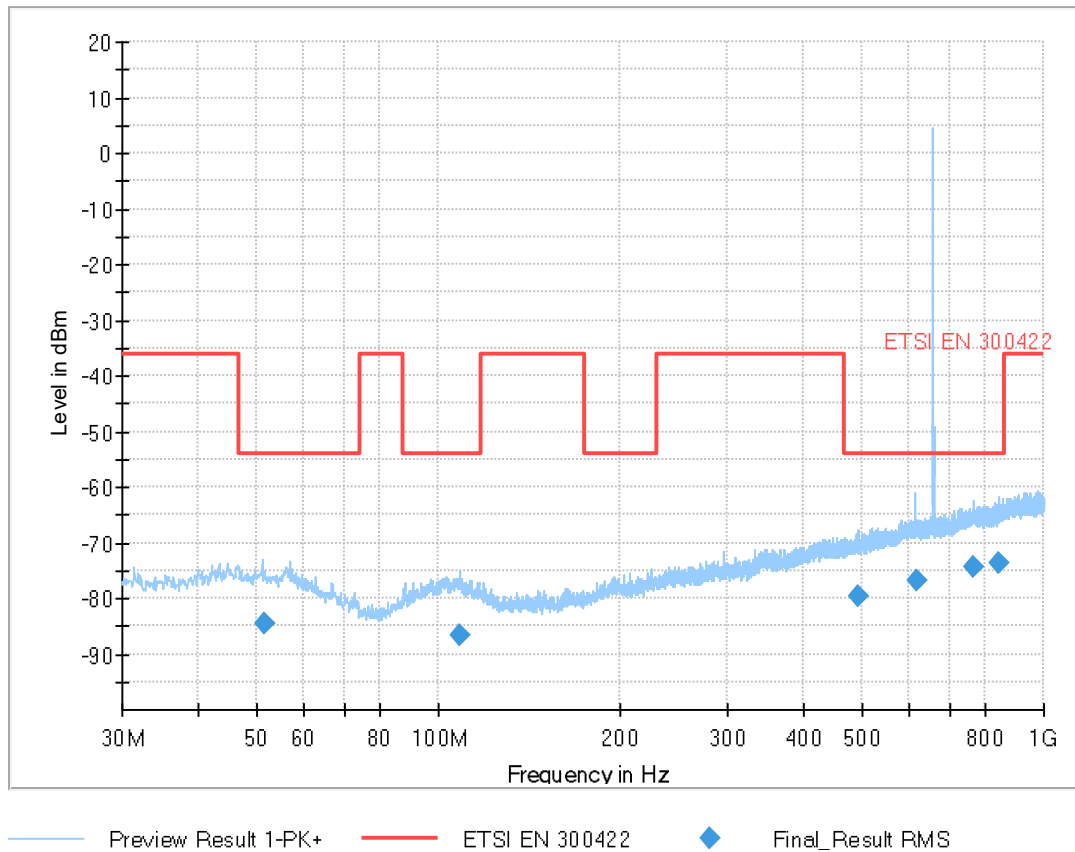
Plot 2: 656.8 MHz, spurious emissions, 30 MHz - 1GHz
