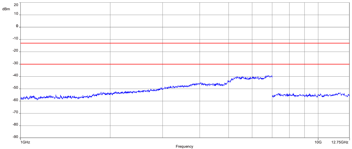
Plot 2: 656.8 MHz, spurious emissions, 1GHz - 12.75 GHz
