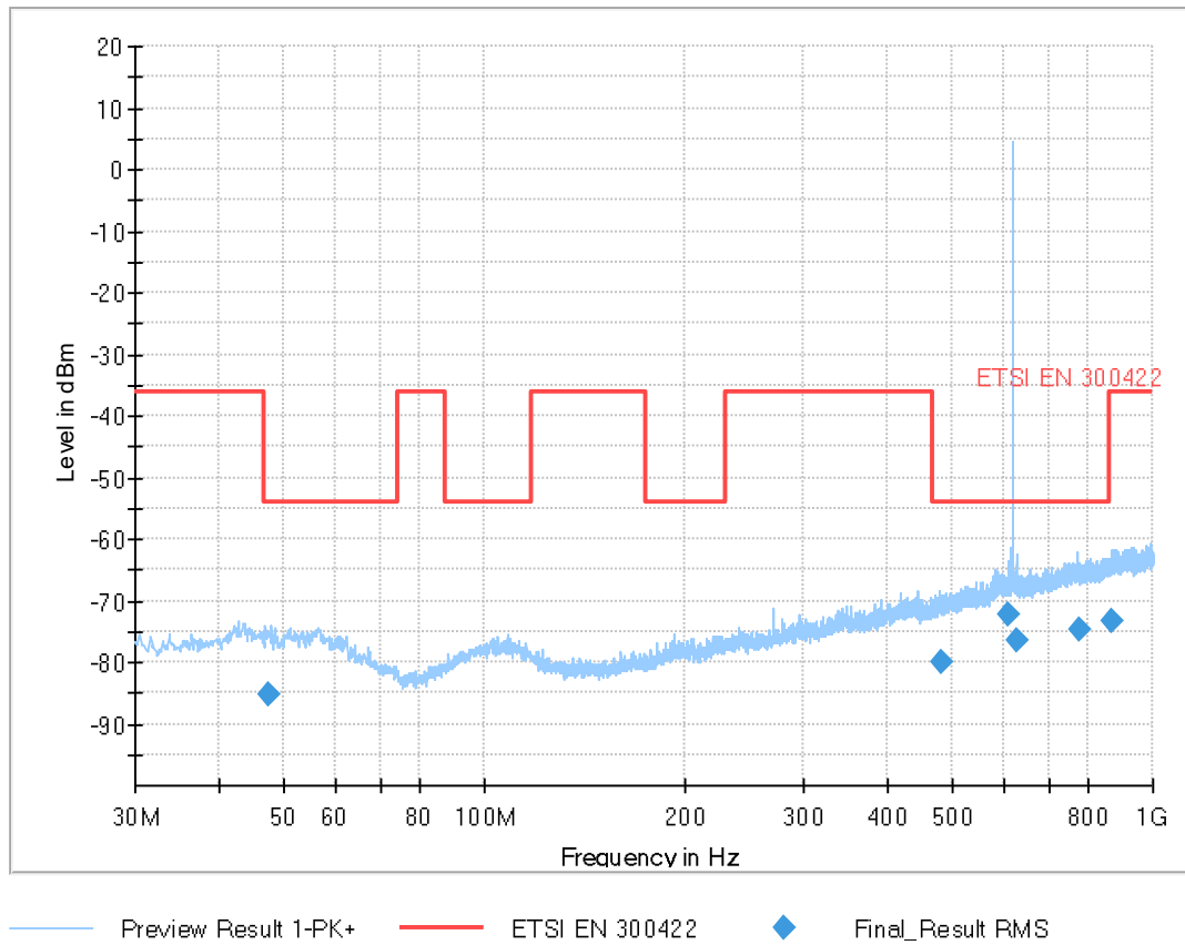
Plot 2: 615.8 MHz, spurious emissions, 30 MHz - 1 GHz
