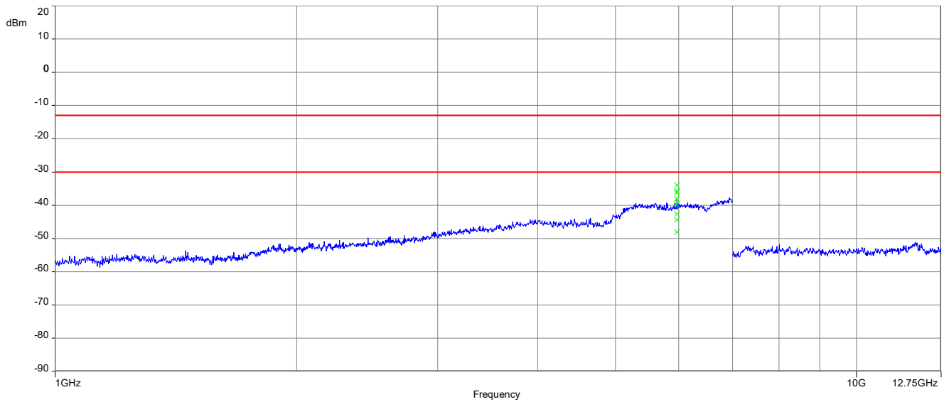
Plot 4: 662.8 MHz, spurious emissions, 1 GHz – 12.75 GHz
