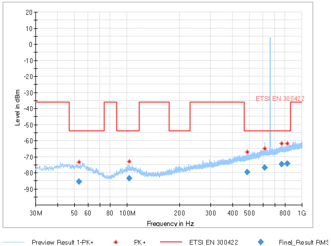
Plot 3: 657.2 MHz, spurious emissions, 30 MHz - 1 GHz
