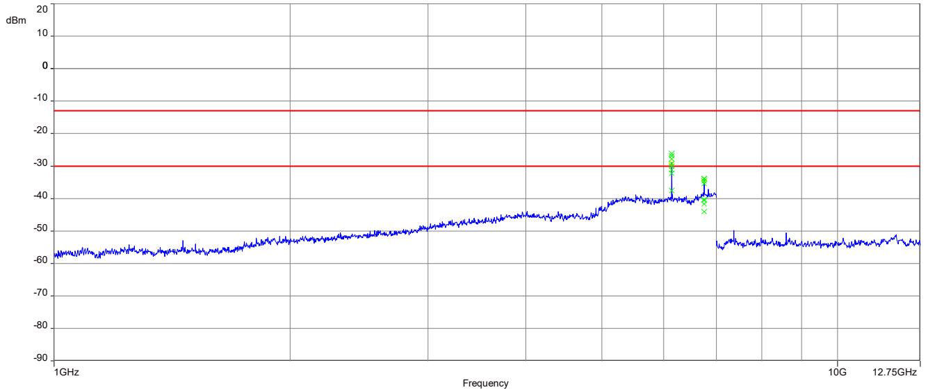
Plot 1: 614.2 MHz, spurious emissions, 1 GHz – 12.75 GHz
