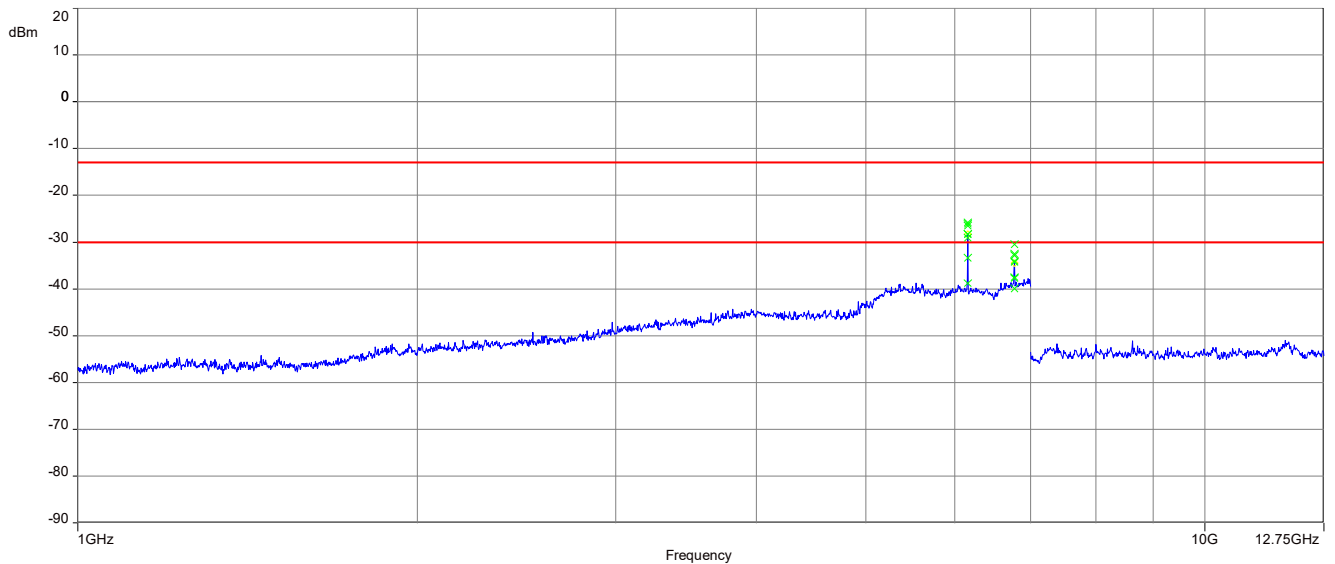
Plot 2: 615.8 MHz, spurious emissions, 1 GHz – 12.75 GHz
