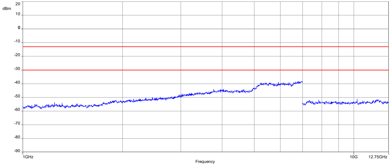
Plot 3: 657.2 MHz, spurious emissions, 1 GHz – 12.75 GHz
