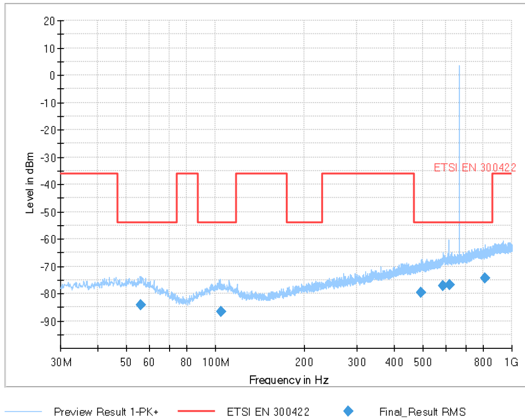
Plot 4: 662.8 MHz, spurious emissions, 30 MHz - 1 GHz
