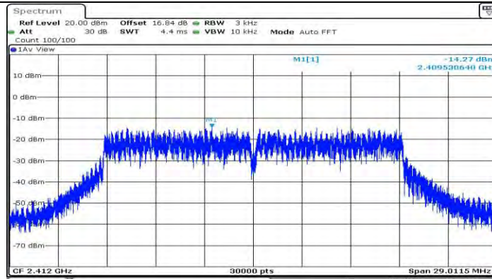
11N20SISO_Ant1_2412
