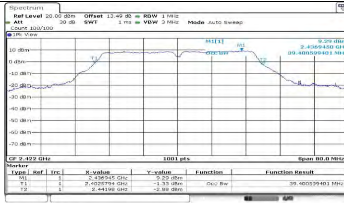
11N40SISO_Ant1_2422
