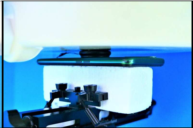
Front Face of EUT Tested at 0 mm_SKU 1 w/ Host
