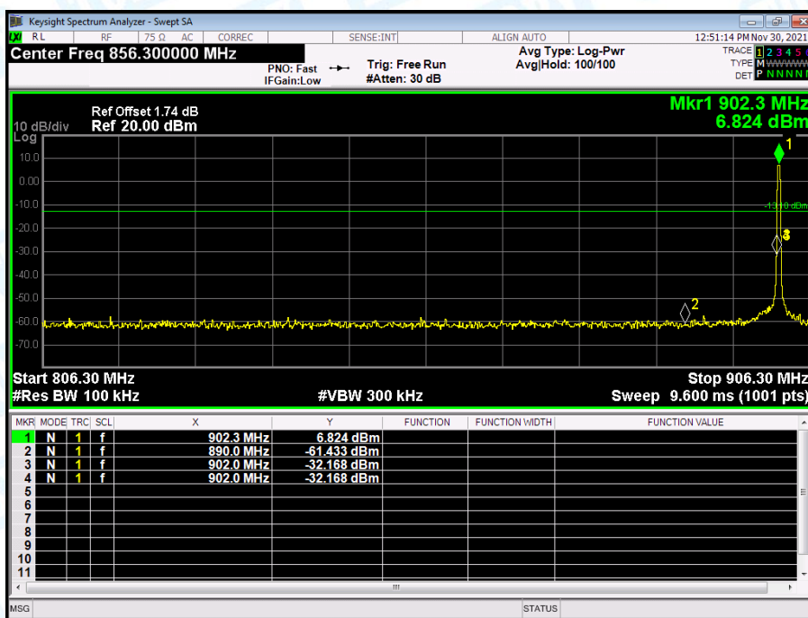
Band Edge NVNT LoRa 902.3MHz Ant1 Emission
