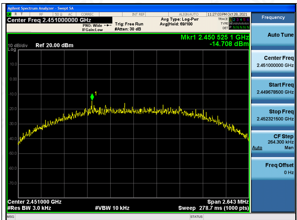
Test_Graph_LE2M_ANT1_2451_2Mbps_PSD
