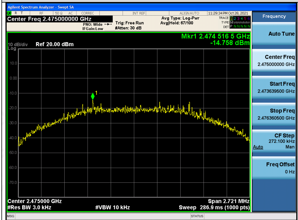
Test_Graph_LE2M_ANT1_2475_2Mbps_PSD
