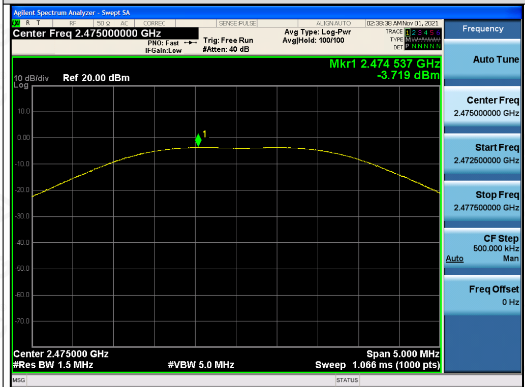
Test_Graph_LE2M_ANT1_2475_2Mbps_Peak Power
