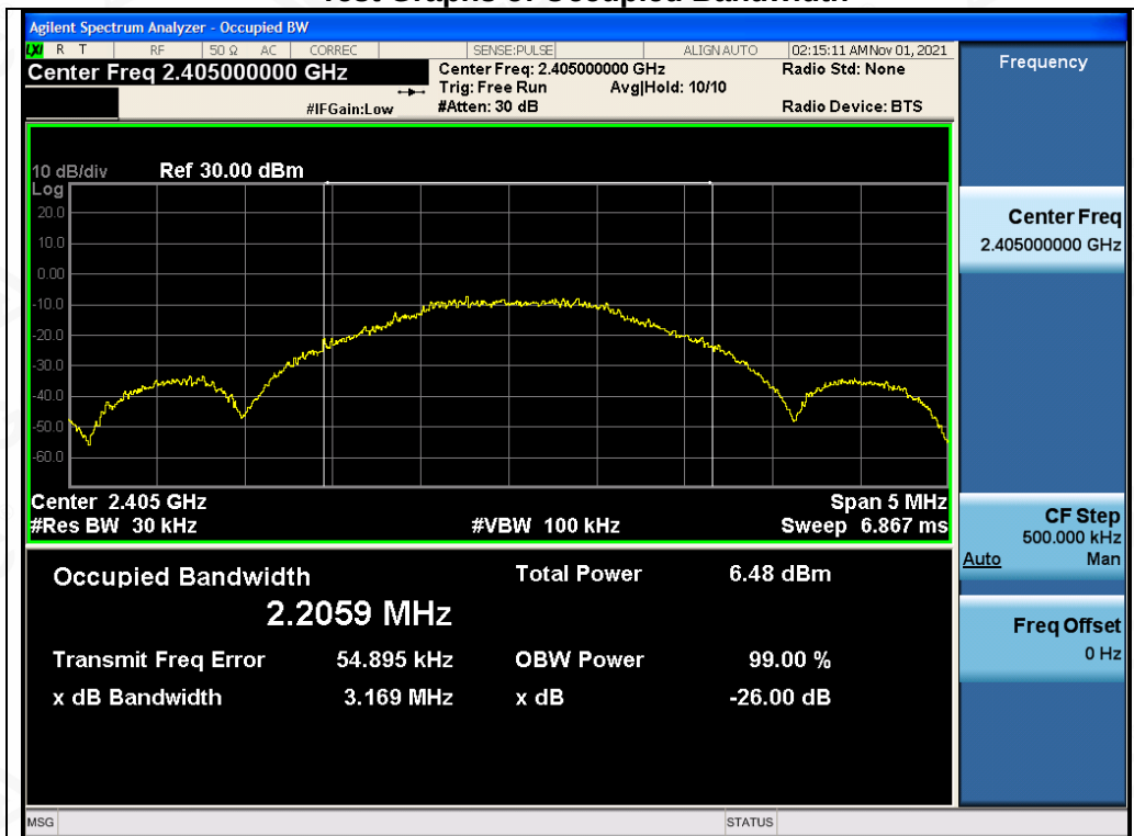
Test_Graph_LE2M_ANT1_2405_2Mbps_OBW
