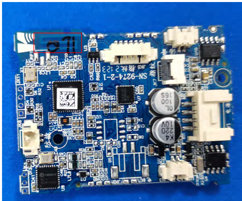
BT ANTENNA
