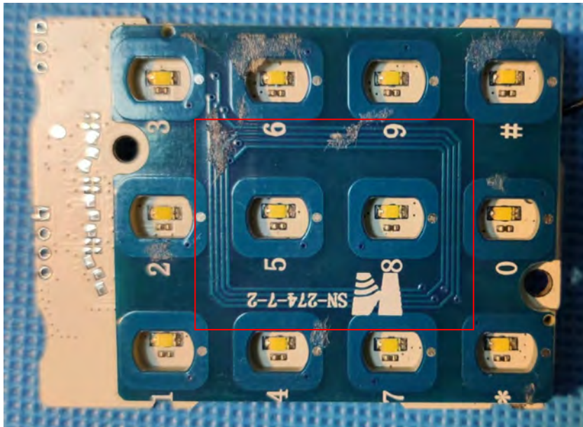
Loop antenna
