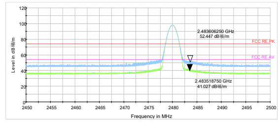
Bluetooth LE Channel 39 Peak & Average
