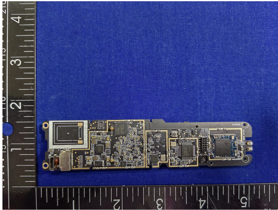
EUT View 11
