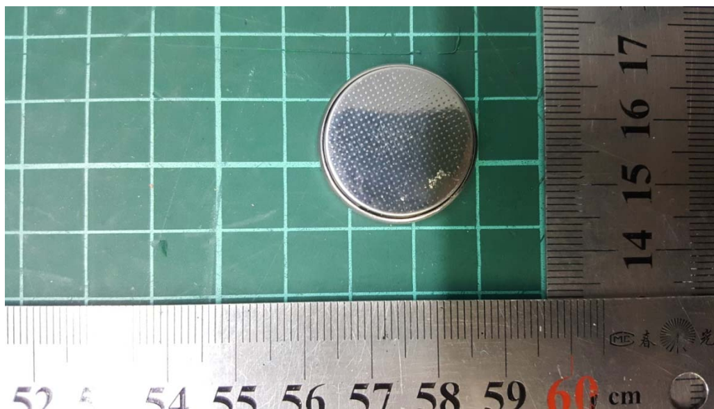
Battery Model:CR2450
