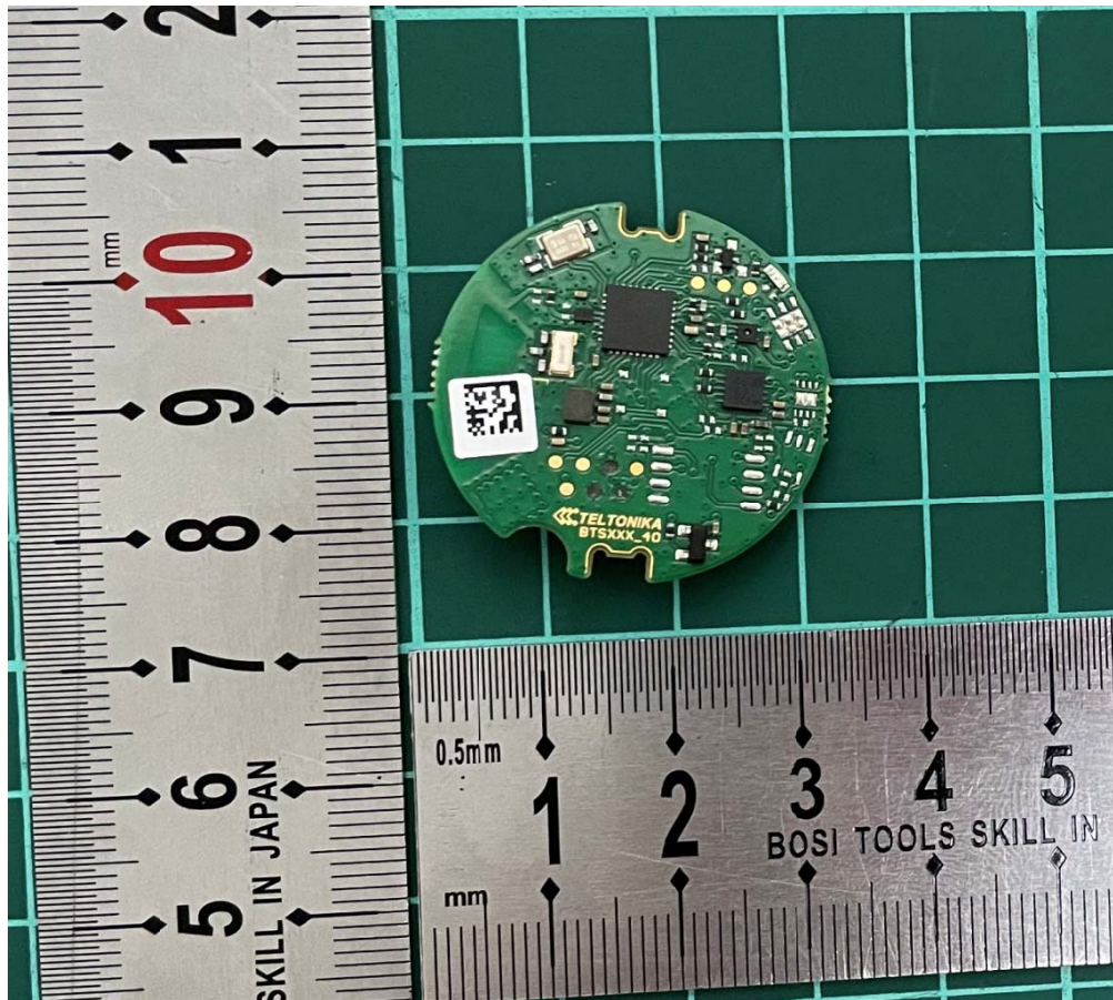
Mode: BTSMP1
