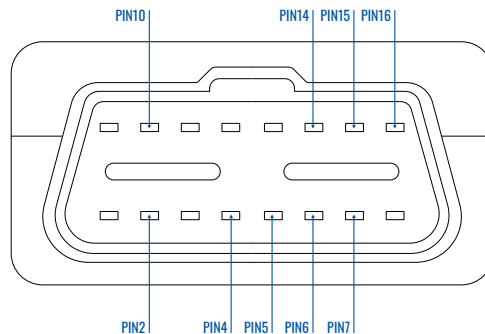
FMC00A OBDII socket pinout
