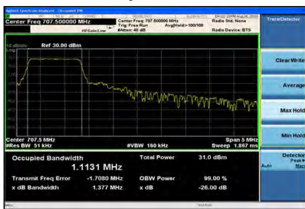
LTE Band 12 16QAM 1.4MHz CH-Middle
