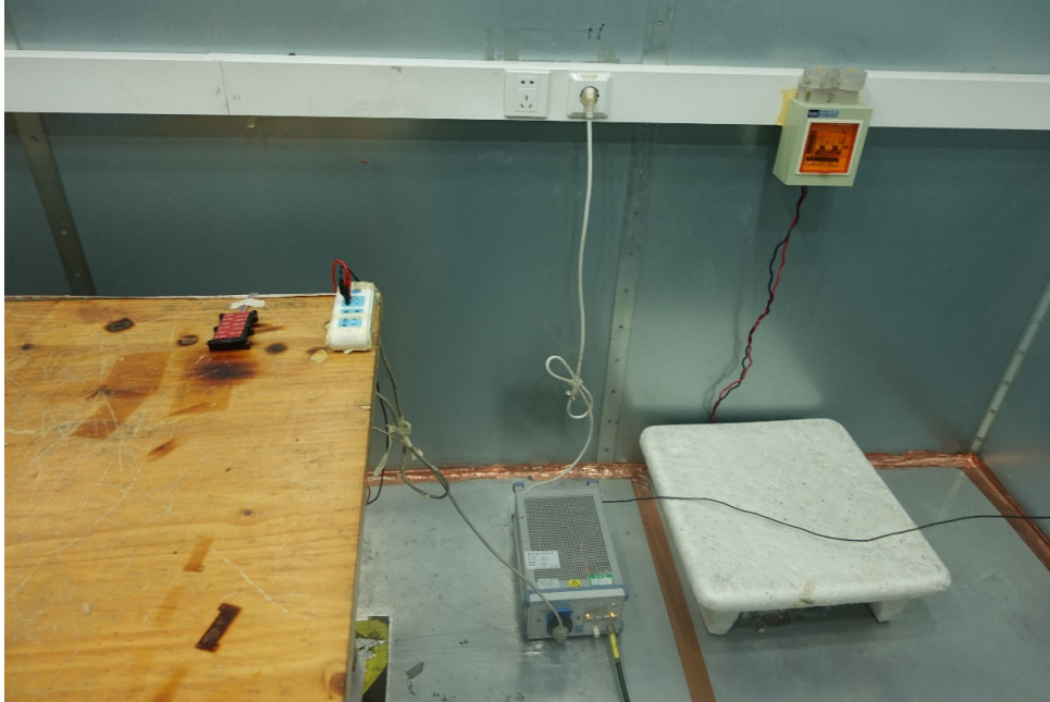
Picture 2 Conducted Emission Test Setup
