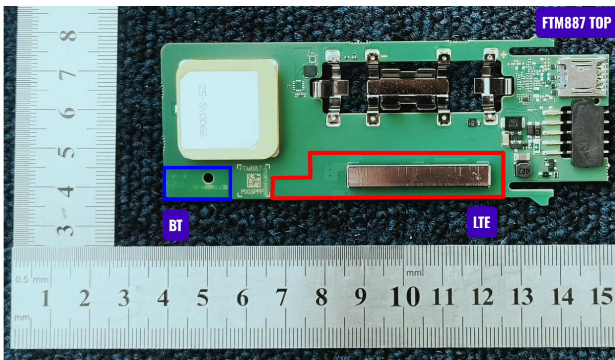
LTE BT antenna size diagram
