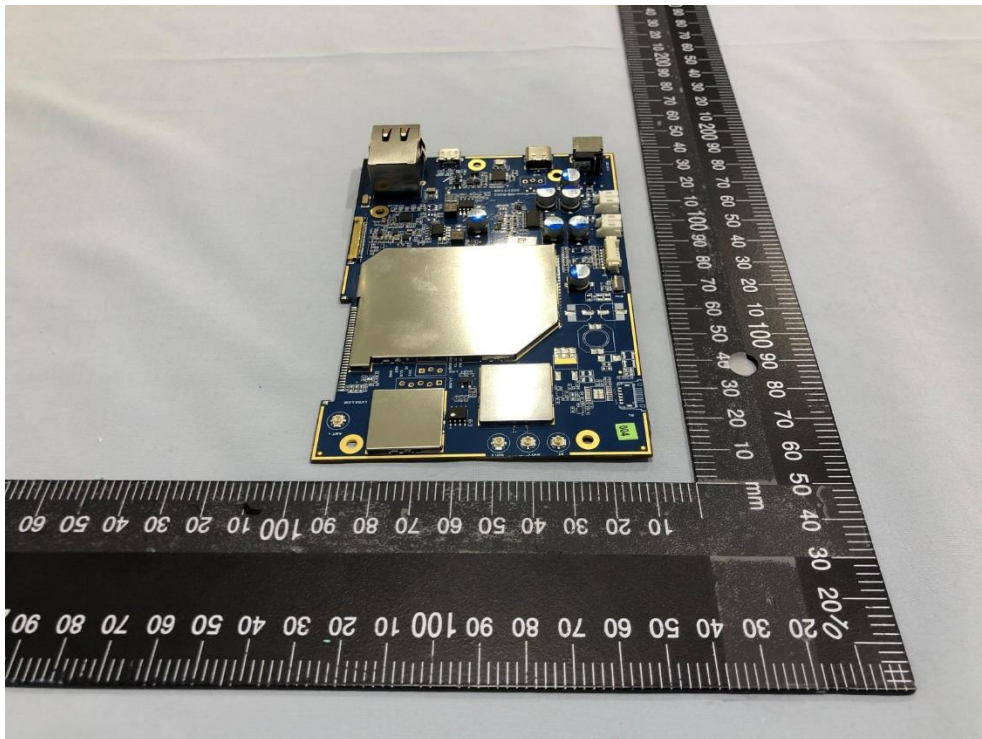
Outview: CIC15101 Pic 6
