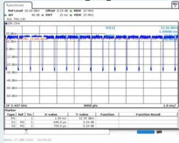
802.11n HT40_Ant1_2437MHz
