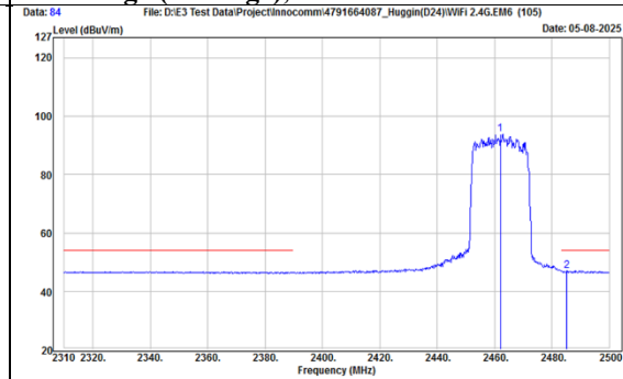
TX, 802.11ax(HE20) (Ch 11) Band Edge (Peak), Vertical
