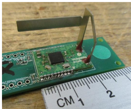
Figure 1: Picture of antenna assembled to RMG3_RCOM-B module.
