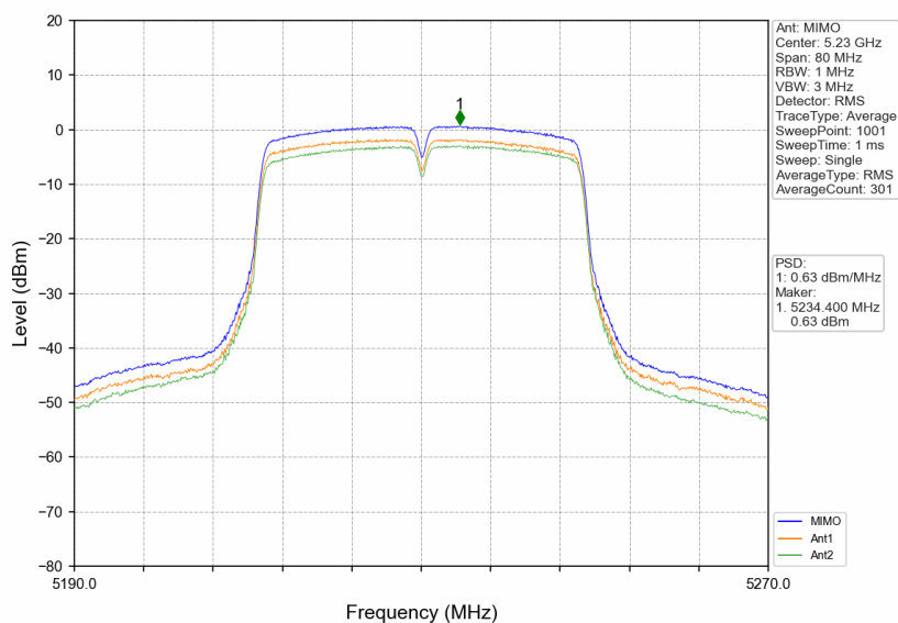
802.11ac(VHT40)_HCH_5230MHz_MIMO_NTNV
