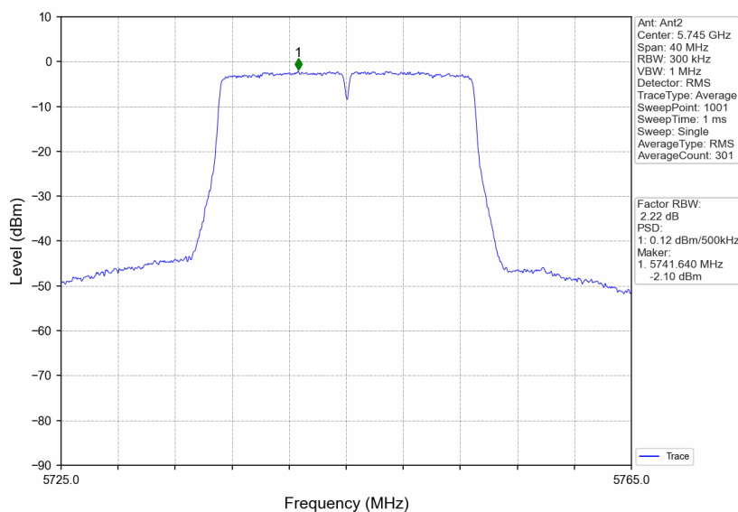
802.11n(HT20)_LCH_5745MHz_Ant2_NTNV
