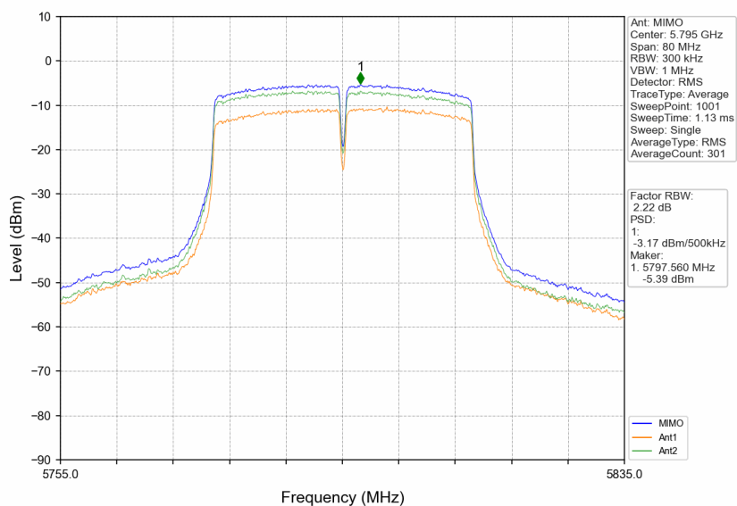
802.11ac(VHT40)_HCH_5795MHz_MIMO_NTNV
