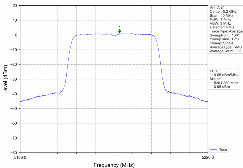
802.11n(HT20)_MCH_5200MHz_Ant1_NTNV
