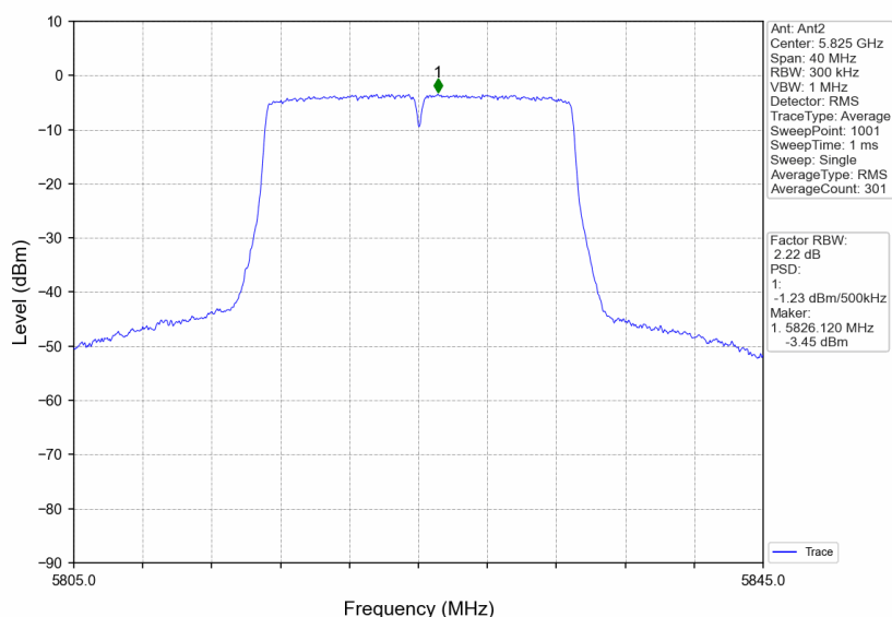
802.11ac(VHT20)_HCH_5825MHz_MIMO_NTNV
