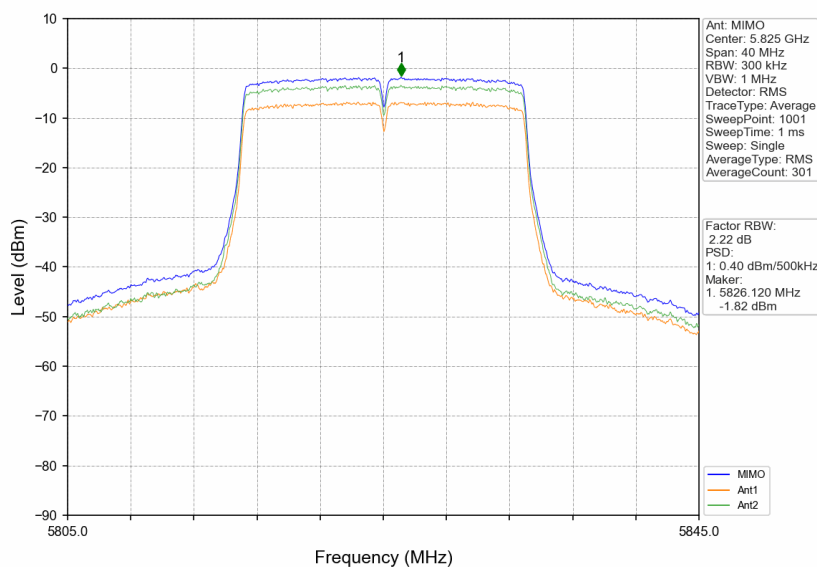
802.11ac(VHT20)_HCH_5825MHz_MIMO_NTNV
