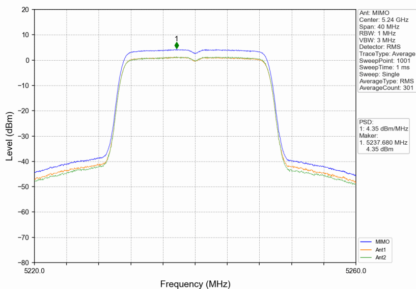
802.11ac(VHT20) HCH 5240MHz MIMO_NTNV
