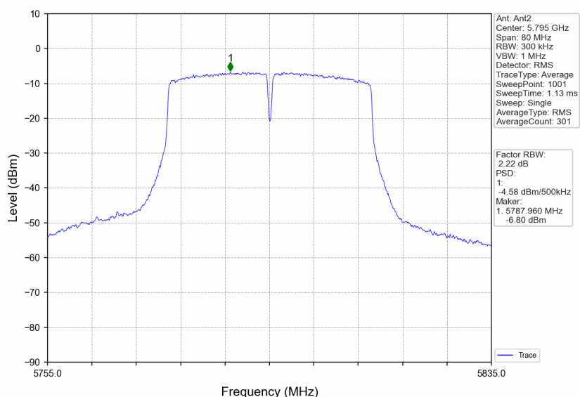
802.11ac(VHT40)_HCH_5795MHz_MIMO_NTNV
