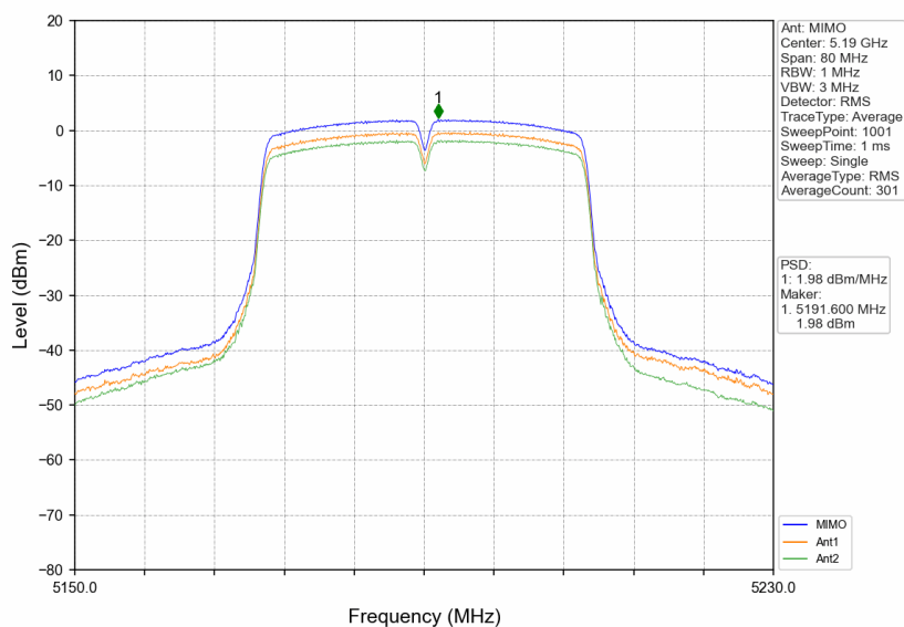
802.11n(HT40)_LCH_5190MHz_MIMO_NTNV
