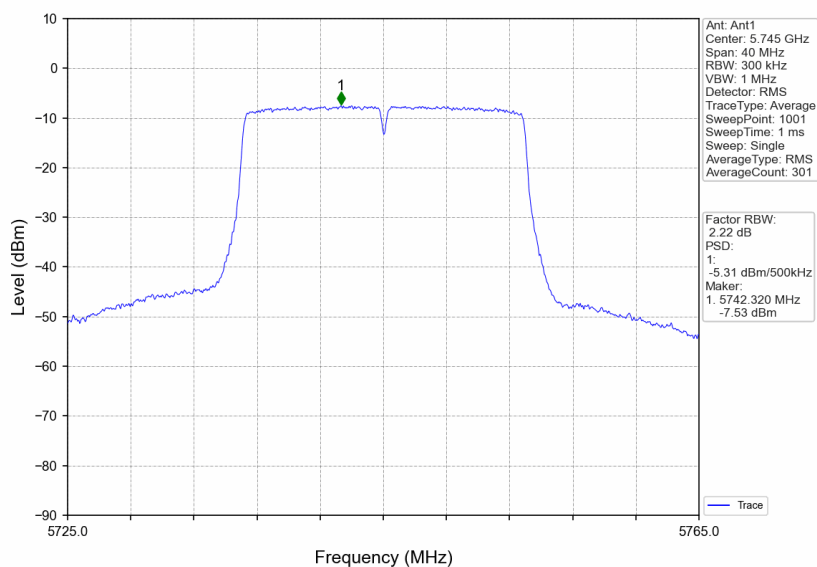
802.11ac(VHT20)_LCH_5745MHz_Ant1_NTNV
