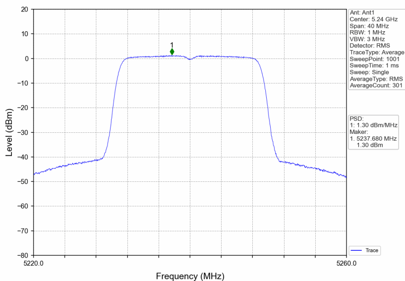
802.11ac(VHT20)_HCH_5240MHz_Ant1_NTNV
