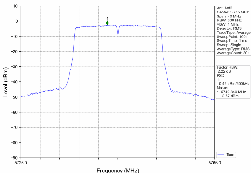
802.11ac(VHT20)_LCH_5745MHz_MIMO_NTNV
