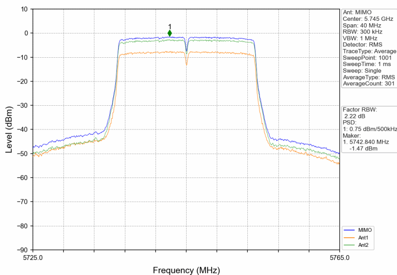
802.11ac(VHT20)_LCH_5745MHz_MIMO_NTNV
