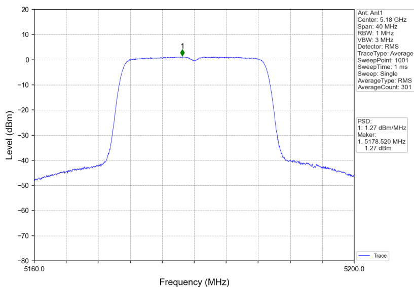
802.11ac(VHT20)_LCH_5180MHz_Ant1_NTNV
