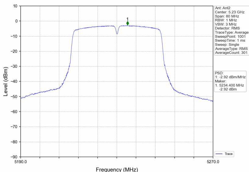
802.11ac(VHT40)_HCH_5230MHz_MIMO_NTNV
