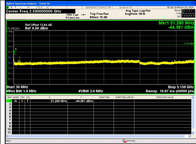
Spurious Emission:30.0~5150 MHz IEEE 802.11n_Channel 48_20MHz_Antenna 0
