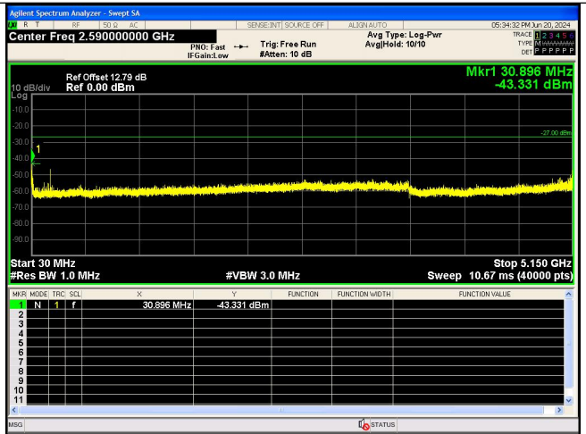
Spurious Emission:30.0~5150 MHz IEEE 802.11n_Channel 40_20MHz_Antenna 0
