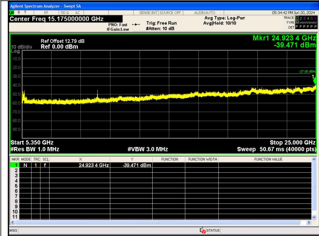
Spurious Emission:5350~25000.0 MHz IEEE 802.11n_Channel 40_20MHz_Antenna 0
