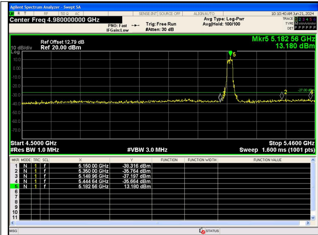
Out Of Band Emission IEEE 802.11a_Channel 36_20MHz_Antenna 0
