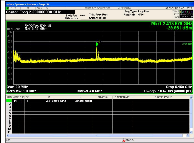
Spurious Emission:30.0~5150 MHz IEEE 802.11n_Channel 44_20MHz_Antenna 0
