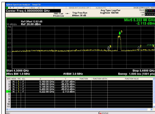
Out Of Band Emission IEEE 802.11ac_Channel 44_20MHz_Antenna 0
