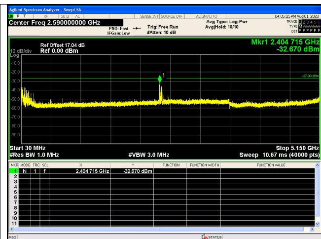
Spurious Emission:30.0~5150 MHz IEEE 802.11ac_Channel 44_20MHz_Antenna 0
