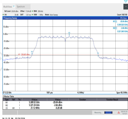
11N20SISO-Ant1-5320
