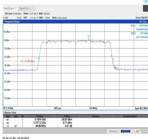
11AX40SISO-Ant1-5190
