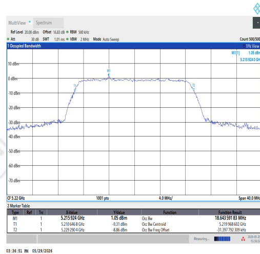
11N20SISO-Ant1-5220
