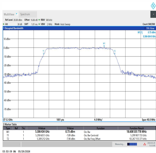
11N20SISO-Ant1-5300
