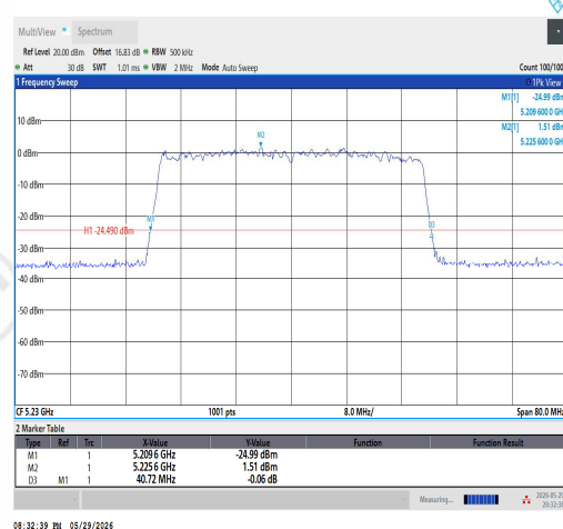
11AX40SISO-Ant1-5230
