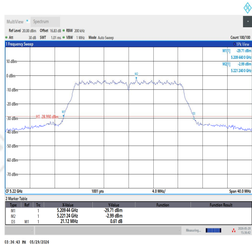
11N20SISO-Ant1-5220
