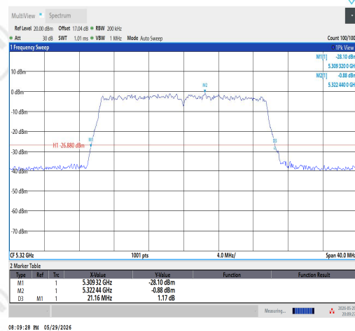
11AX20SISO-Ant1-5320
