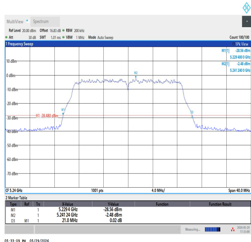
11AC20SISO-Ant1-5240
