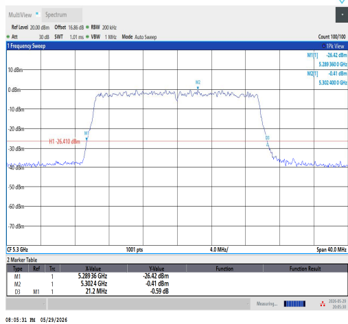
11AX20SISO-Ant1-5300
