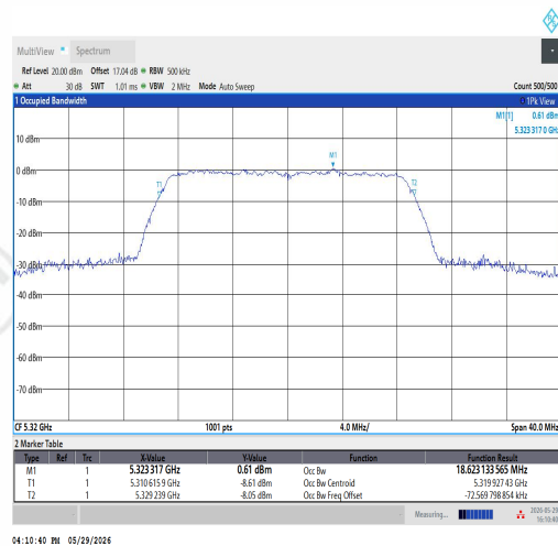
11N20SISO-Ant1-5320
