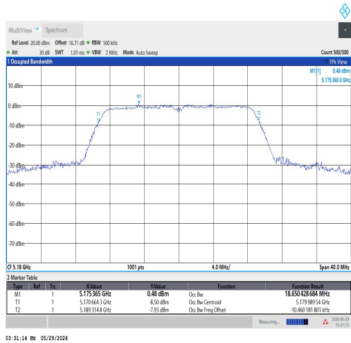
11N20SISO-Ant1-5180
