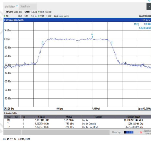
11N20SISO-Ant1-5260
