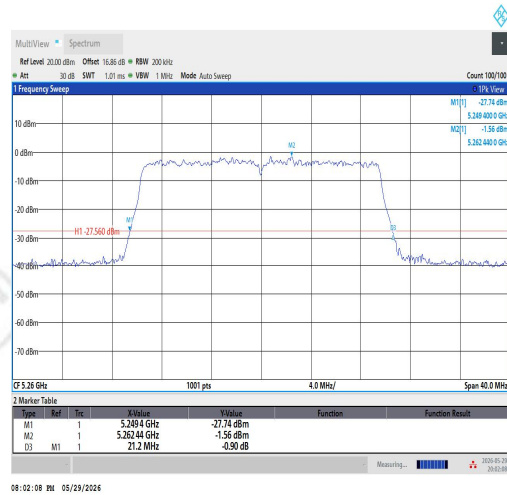
11AX20SISO-Ant1-5260
