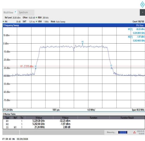
11AX20SISO-Ant1-5240
