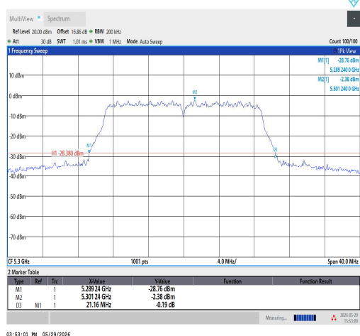
11N20SISO-Ant1-5300
