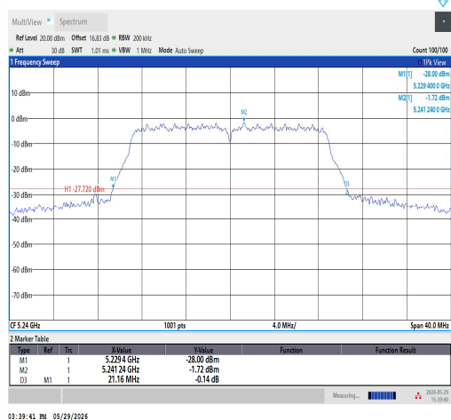
11N20SISO-Ant1-5240
