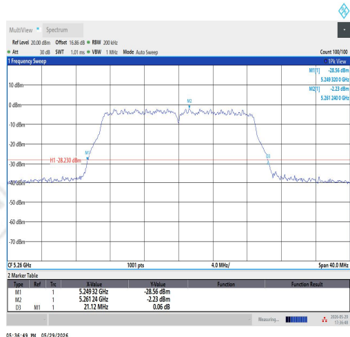
11AC20SISO-Ant1-5260
