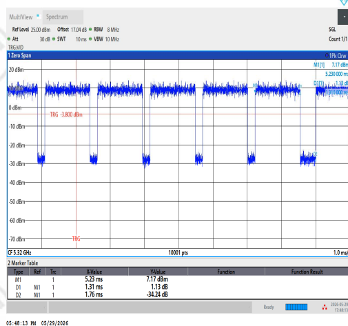
NTNV-11AC20SISO-Ant1-5320
