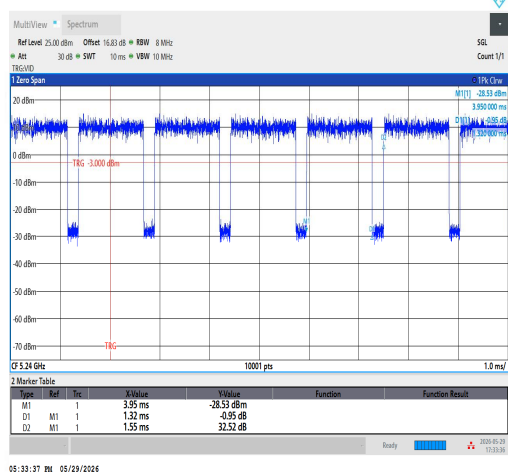
NTNV-11AC20SISO-Ant1-5240
