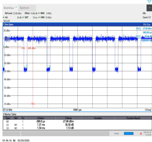
NTVN-11N20SISO-Ant1-5300
