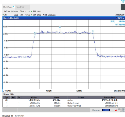
11AX40SISO-Ant1-5190
