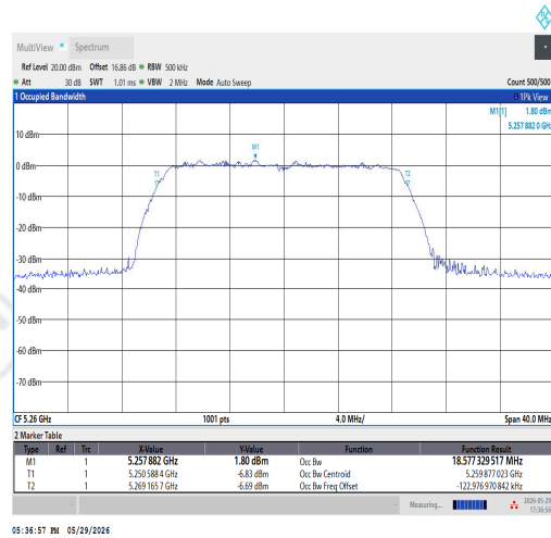
11AC20SISO-Ant1-5260
