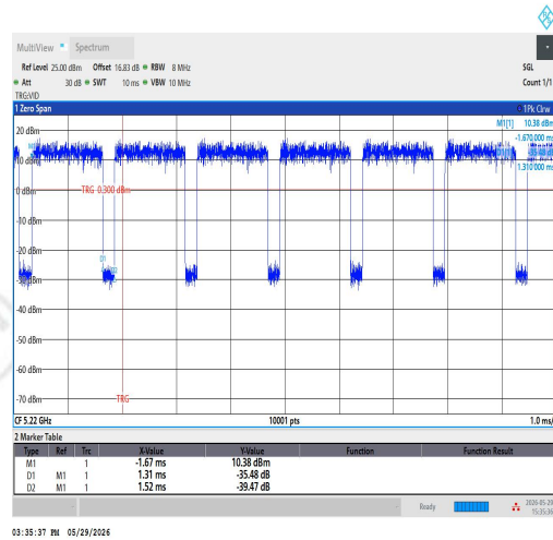
NTVN-11N20SISO-Ant1-5220
