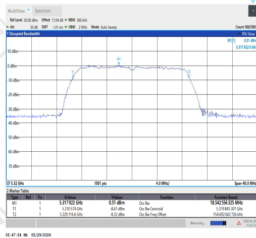
11AC20SISO-Ant1-5320
