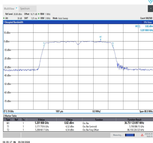
11AC40SISO-Ant1-5190
