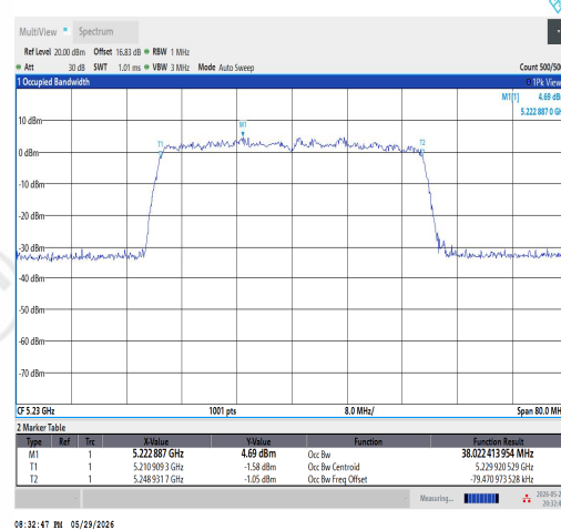
11AX40SISO-Ant1-5230
