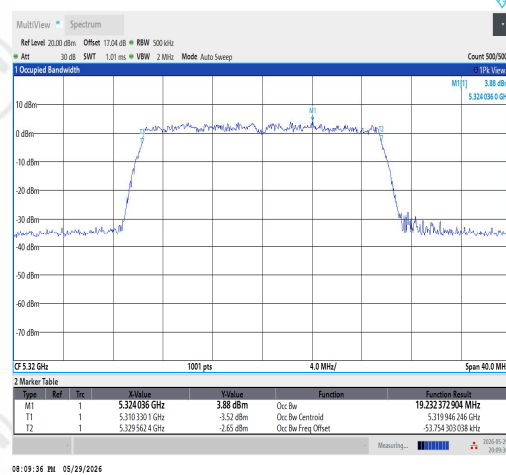
11AX20SISO-Ant1-5320
