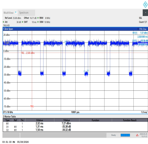
NTVN-11N20SISO-Ant1-5180
