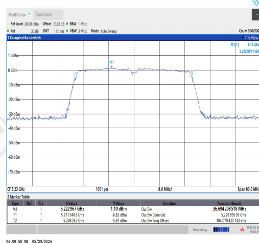
11AC40SISO-Ant1-5230
