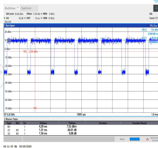
NTVN-11N20SISO-Ant1-5320
