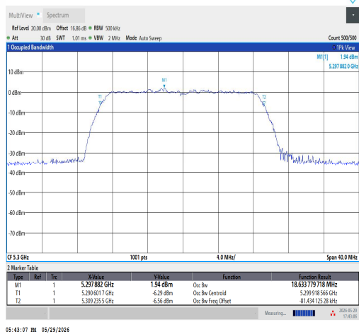
11AC20SISO-Ant1-5300
