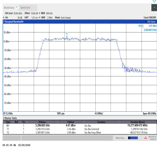
11AX20SISO-Ant1-5300
