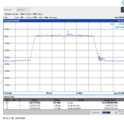
11AX20SISO-Ant1-5260
