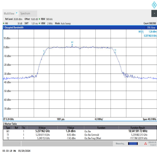
11AC20SISO-Ant1-5240
