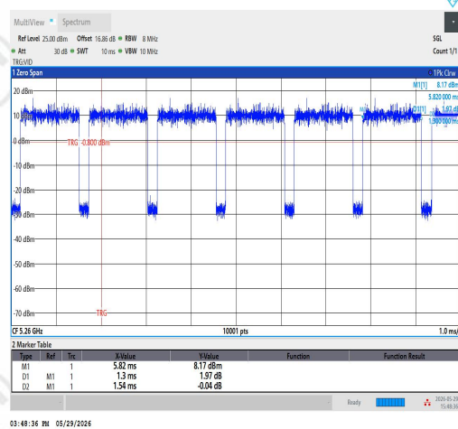
NTVN-11N20SISO-Ant1-5260
