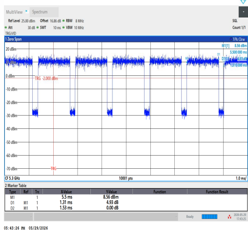
NTNV-11AC20SISO-Ant1-5300
