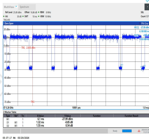
NTNV-11AC20SISO-Ant1-5260
