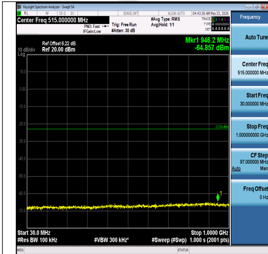
Band2-1.4MHz-16QAM-19193-1RB#5-30~1000- PASS
