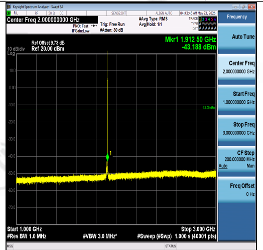
Band2-1.4MHz-16QAM-19193-1RB#5-1000~300 0-PASS
