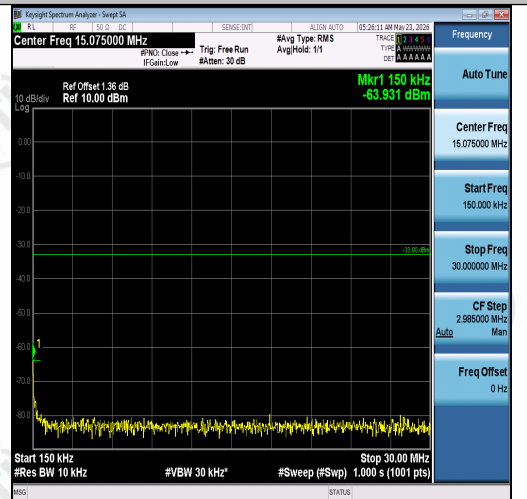
Band2-3MHz-QPSK-18900-1RB#0-0.15~30-PAS S
