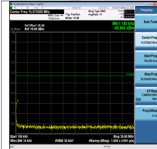
Band2-1.4MHz-16QAM-18900-1RB#0-0.15~30-P ASS
