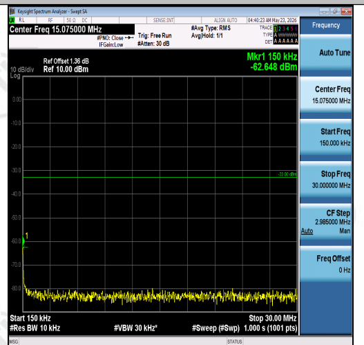
Band2-1.4MHz-QPSK-19193-1RB#0-0.15~30-P ASS
