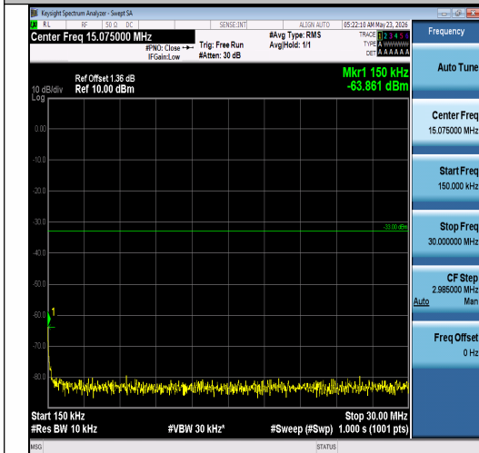
Band2-3MHz-QPSK-18615-1RB#14-0.15~30-PA-SS
