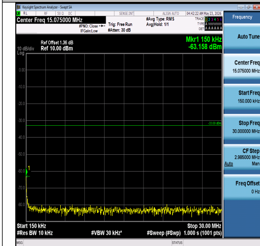
Band2-1.4MHz-QPSK-19193-1RB#5-0.15~30-P ASS
