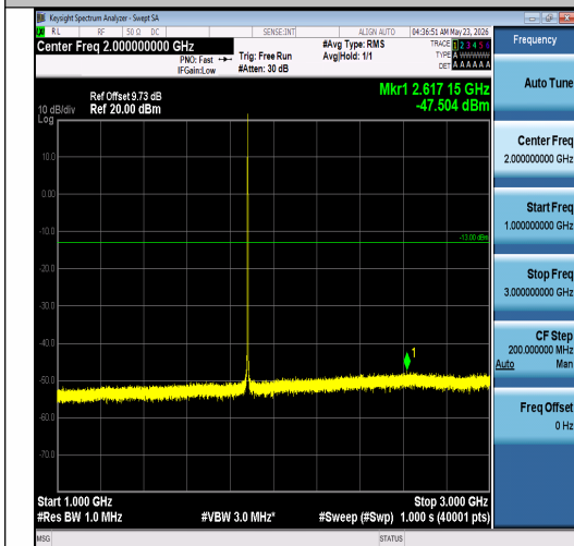
Band2-1.4MHz-QPSK-18900-1RB#5-1000~3000 -PASS
