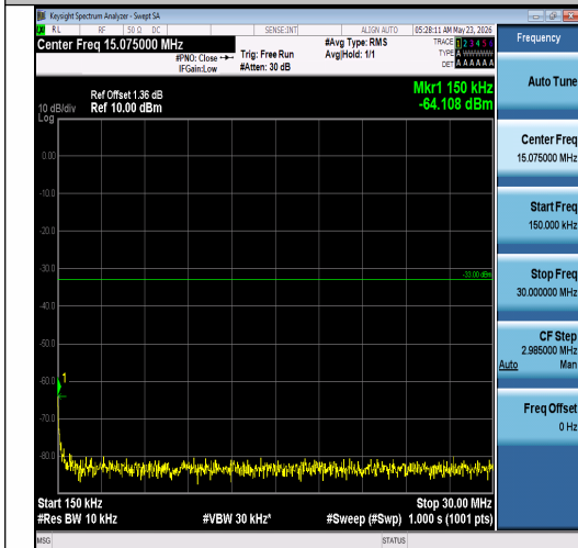
Band2-3MHz-QPSK-18900-1RB#14-0.15~30-PA SS
