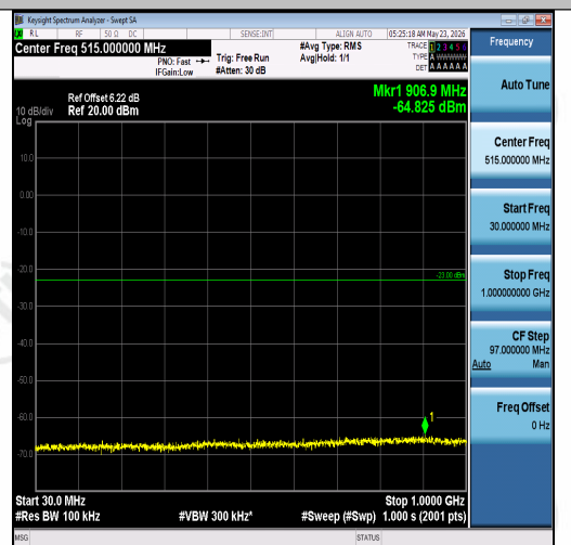
Band2-3MHz-16QAM-18615-15RB#0-30~1000-P ASS
