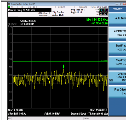
Band2-1.4MHz-16QAM-18900-1RB#5-0.009~0.1 5-PASS
