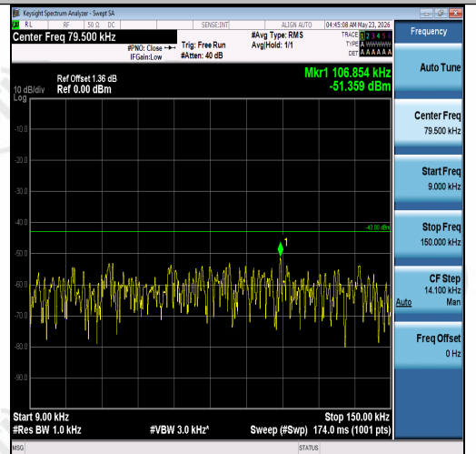
Band2-1.4MHz-16QAM-19193-6RB#0-0.009~0.1 5-PASS
