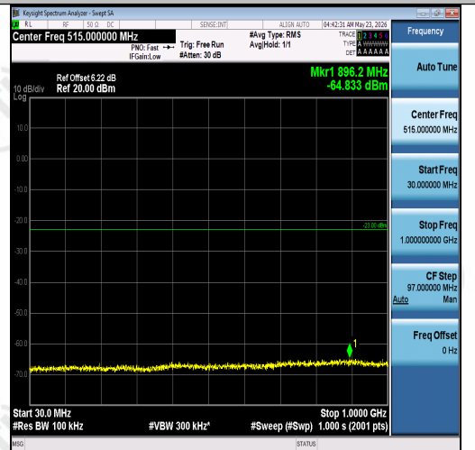
Band2-1.4MHz-QPSK-19193-1RB#5-30~1000-P ASS
