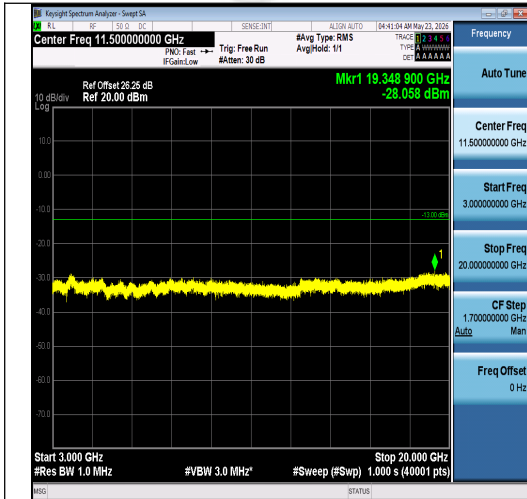
Band2-1.4MHz-QPSK-19193-1RB#0-3000~2000 0-PASS
