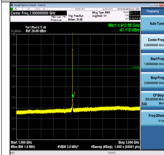
Band2-1.4MHz-QPSK-19193-1RB#5-1000~3000 -PASS
