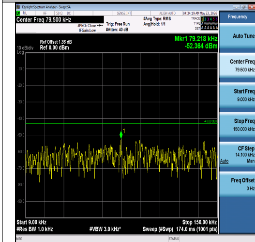
Band2-1.4MHz-QPSK-18900-1RB#0-0.009~0.15 -PASS
