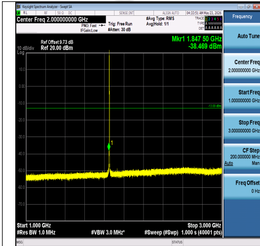
Band2-1.4MHz-16QAM-18607-6RB#0-1000~300 0-PASS
