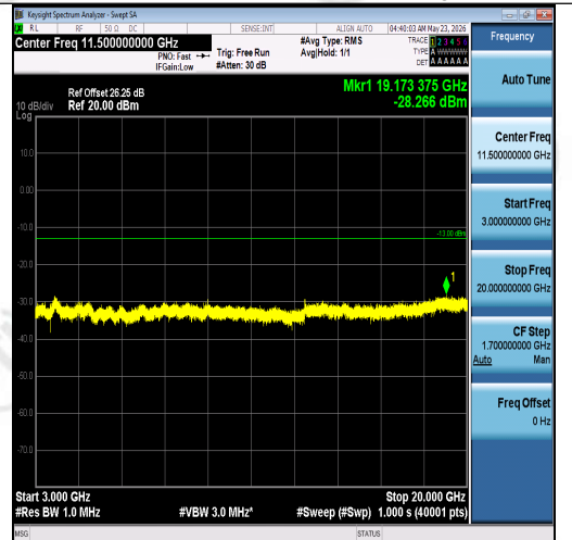
Band2-1.4MHz-16QAM-18900-6RB#0-3000~200 00-PASS
