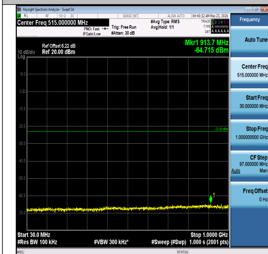
Band2-1.4MHz-QPSK-19193-1RB#0-30~1000-P ASS
