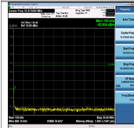
Band2-1.4MHz-16QAM-18900-6RB#0-0.15~30-P ASS
