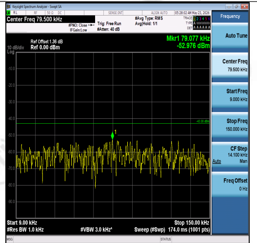
Band2-3MHz-QPSK-18900-1RB#14-0.009~0.15- PASS
