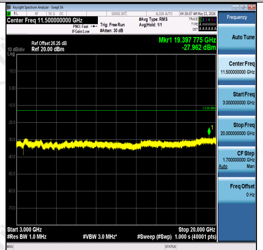
Band2-1.4MHz-16QAM-18900-1RB#0-3000~20000 00-PASS
