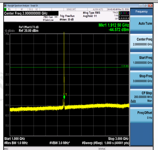
Band2-1.4MHz-QPSK-19193-1RB#0-1000~3000 -PASS
