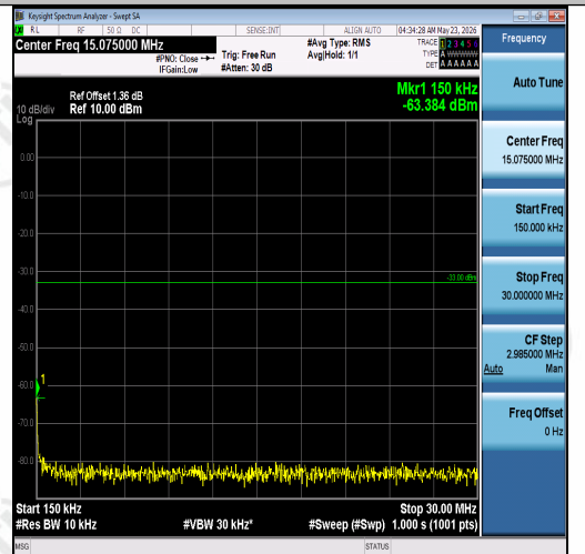
Band2-1.4MHz-QPSK-18900-1RB#0-0.15~30-P ASS
