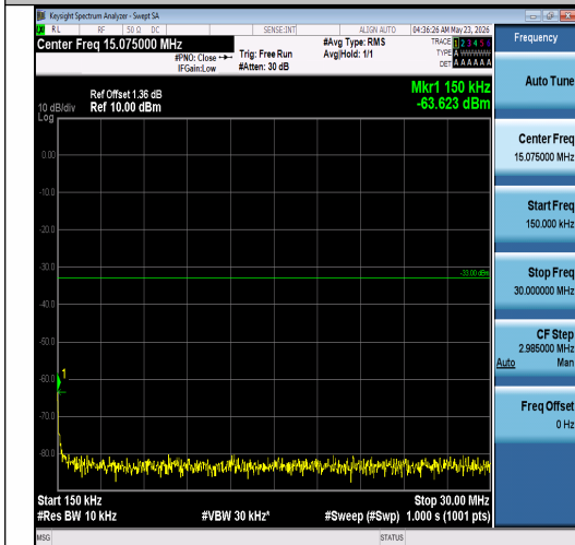
Band2-1.4MHz-QPSK-18900-1RB#5-0.15~30-P ASS
