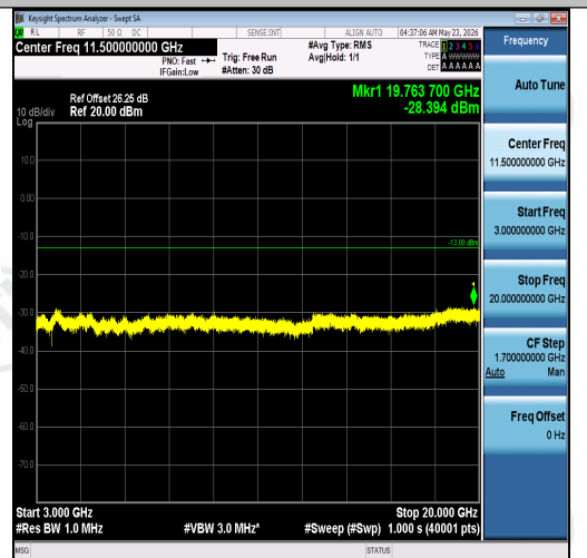
Band2-1.4MHz-QPSK-18900-1RB#5-3000~2000 0-PASS
