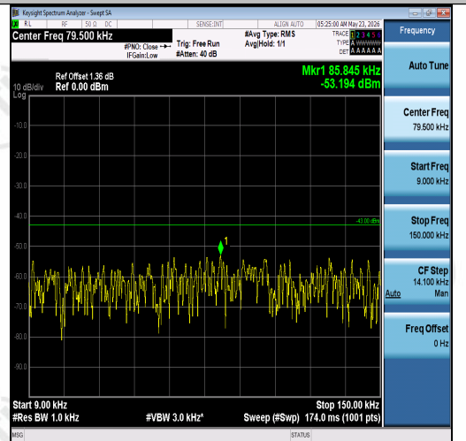
Band2-3MHz-16QAM-18615-15RB#0-0.009~0.1 5-PASS
