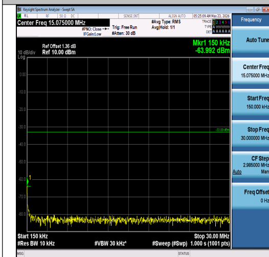
Band2-3MHz-16QAM-18615-15RB#0-0.15~30-P ASS
