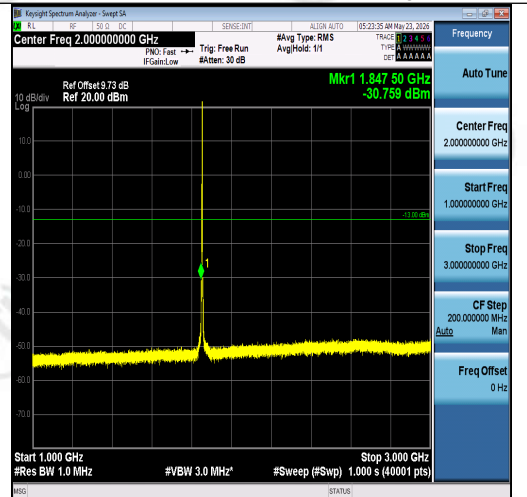
Band2-3MHz-16QAM-18615-1RB#14-1000~300 0-PASS
