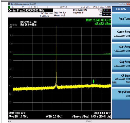
Band2-3MHz-QPSK-18900-1RB#14-1000~3000- PASS
