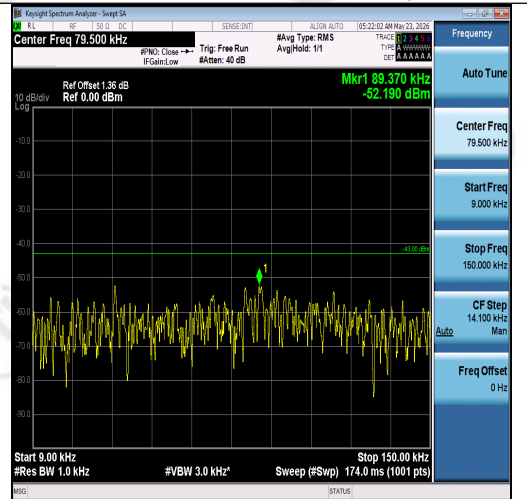
Band2-3MHz-QPSK-18615-1RB#14-0.009~0.15-PASS
