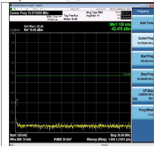
Band2-3MHz-16QAM-18900-1RB#0-0.15~30-PA SS
