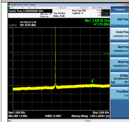
Band2-3MHz-16QAM-18900-1RB#0-1000~3000- PASS
