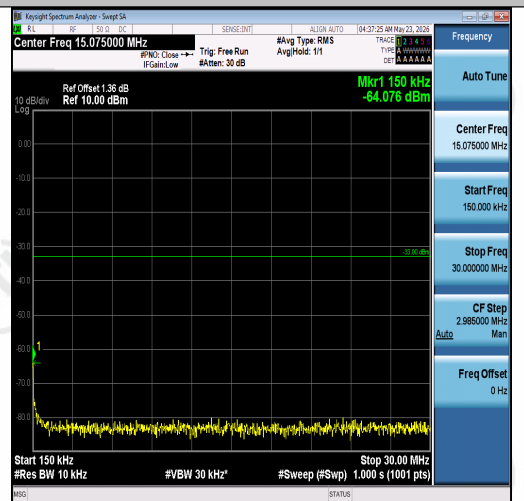
Band2-1.4MHz-16QAM-18900-1RB#5-0.15~30-P ASS
