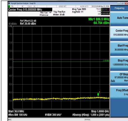
Band2-3MHz-16QAM-18615-1RB#14-30~1000-P ASS
