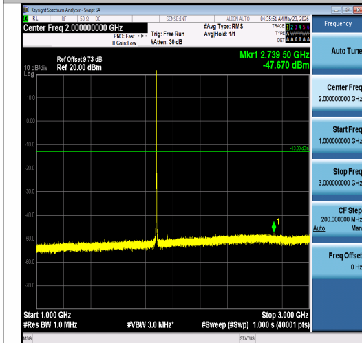
Band2-1.4MHz-16QAM-18900-1RB#0-1000~3000 0-PASS
