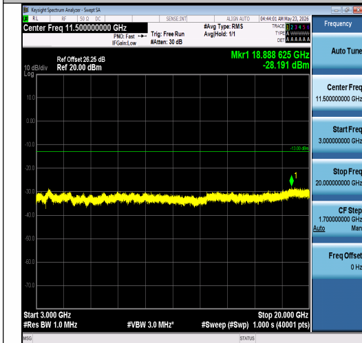
Band2-1.4MHz-16QAM-19193-1RB#5-3000~200 00-PASS
