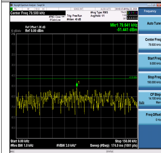
Band2-1.4MHz-QPSK-19193-1RB#0-0.009~0.15 -PASS
