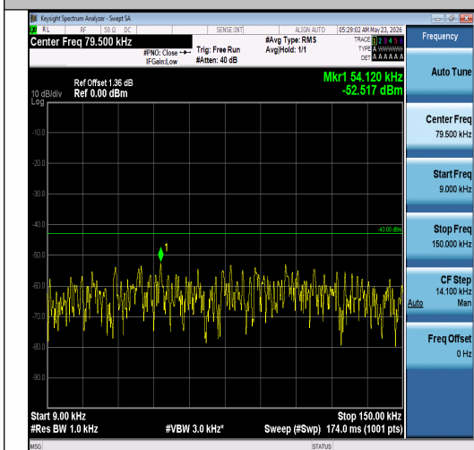
Band2-3MHz-16QAM-18900-1RB#14-0.009~0.1 5-PASS
