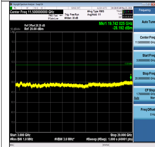
Band2-1.4MHz-16QAM-18900-1RB#5-3000~200 00-PASS
