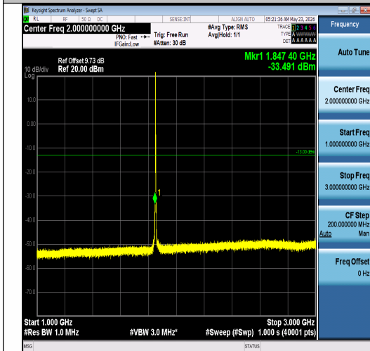
Band2-3MHz-16QAM-18615-1RB#0-1000~3000- PASS
