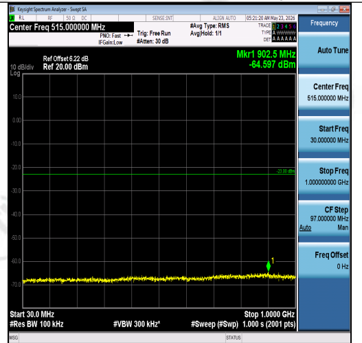
Band2-3MHz-16QAM-18615-1RB#0-30~1000-P ASS
