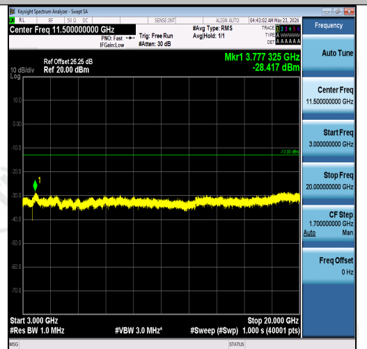
Band2-1.4MHz-QPSK-19193-1RB#5-3000~2000 0-PASS
