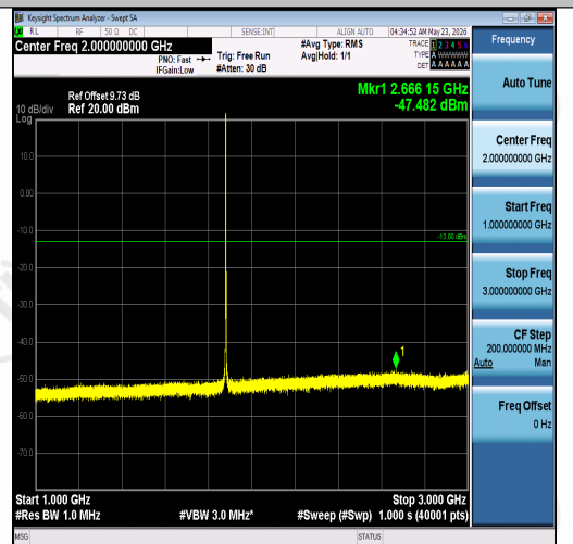
Band2-1.4MHz-QPSK-18900-1RB#0-1000~3000 -PASS
