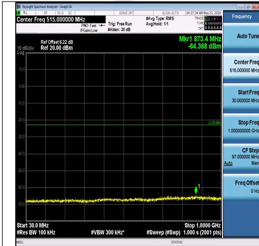
Band2-1.4MHz-16QAM-18900-1RB#5-30~1000- PASS
