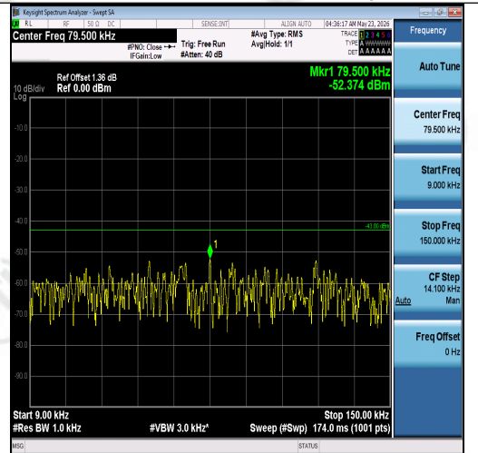
Band2-1.4MHz-QPSK-18900-1RB#5-0.009~0.15 -PASS
