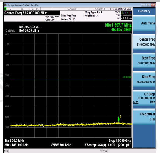
Band2-1.4MHz-16QAM-19193-6RB#0-30~1000- PASS
