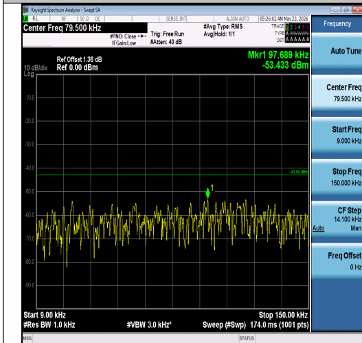
Band2-3MHz-QPSK-18900-1RB#0-0.009~0.15-P ASS
