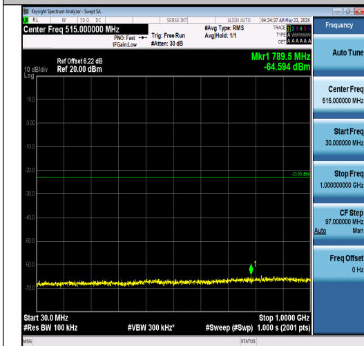
Band2-1.4MHz-QPSK-18900-1RB#0-30~1000-P ASS
