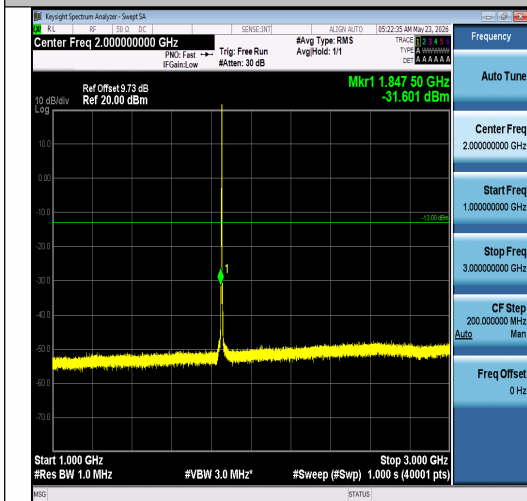
Band2-3MHz-QPSK-18615-1RB#14-1000~3000-PASS
