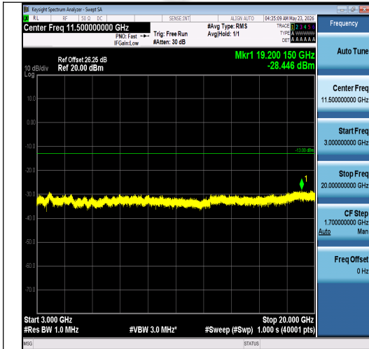
Band2-1.4MHz-QPSK-18900-1RB#0-3000~2000 0-PASS
