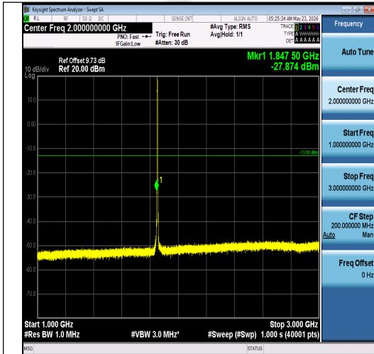
Band2-3MHz-16QAM-18615-15RB#0-1000~300 0-PASS
