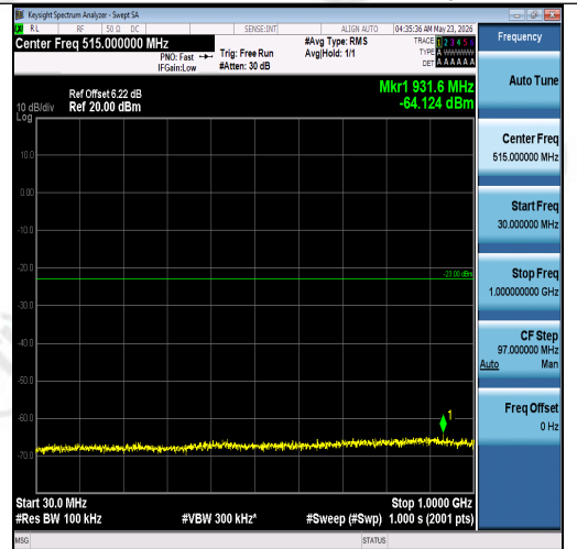
Band2-1.4MHz-16QAM-18900-1RB#0-30~1000- PASS
