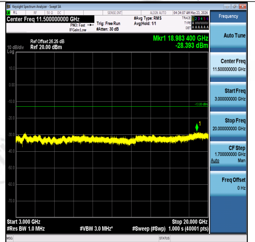
Band2-1.4MHz-16QAM-18607-6RB#0-3000~200 00-PASS
