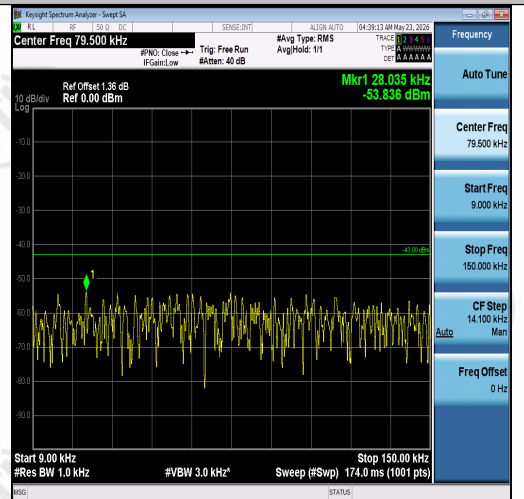
Band2-1.4MHz-16QAM-18900-6RB#0-0.009~0.1 5-PASS
