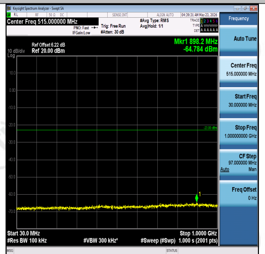
Band2-1.4MHz-16QAM-18900-6RB#0-30~1000- PASS
