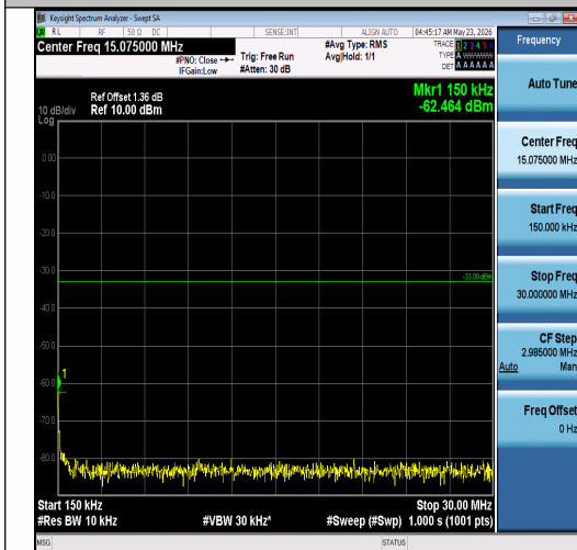
Band2-1.4MHz-16QAM-19193-6RB#0-0.15~30-P ASS
