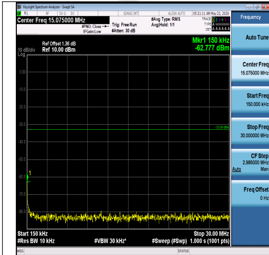
Band2-3MHz-16QAM-18615-1RB#0-0.15~30-PA SS
