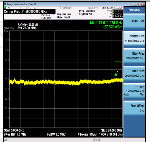
Band2-3MHz-16QAM-18615-1RB#0-3000~2000 0-PASS
