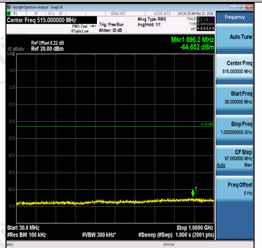
Band2-1.4MHz-QPSK-18900-1RB#5-30~1000-P ASS
