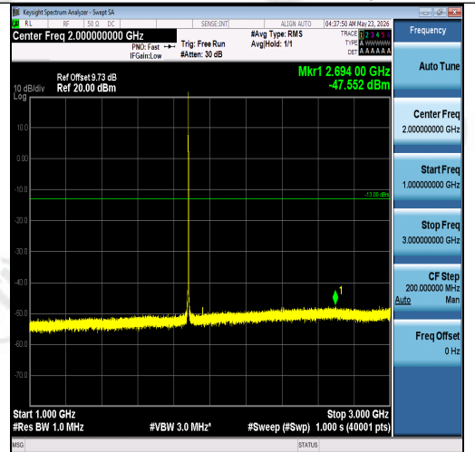
Band2-1.4MHz-16QAM-18900-1RB#5-1000~300 0-PASS
