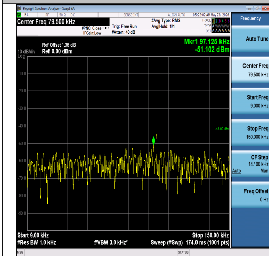
Band2-3MHz-16QAM-18615-1RB#14-0.009~0.1 5-PASS
