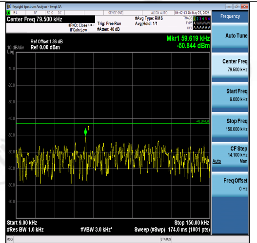
Band2-1.4MHz-QPSK-19193-1RB#5-0.009~0.15 -PASS
