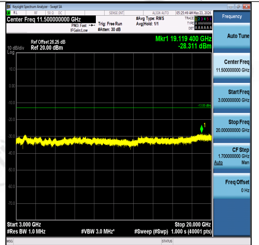
Band2-3MHz-16QAM-18615-15RB#0-3000~200 00-PASS
