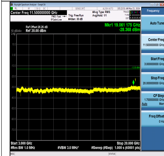
Band2-3MHz-16QAM-18615-1RB#14-3000~200 00-PASS
