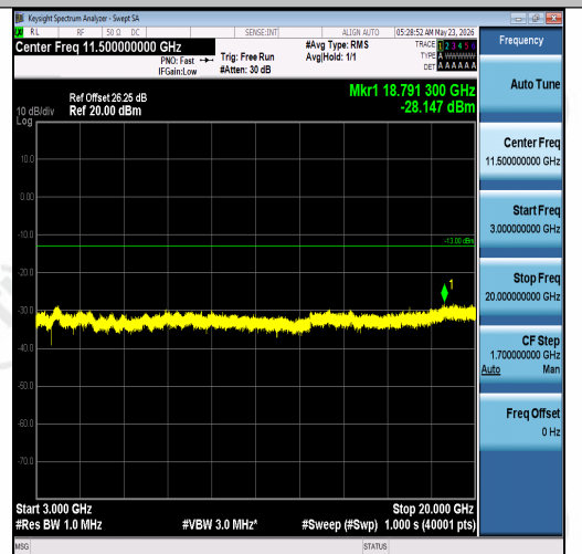
Band2-3MHz-QPSK-18900-1RB#14-3000~2000 0-PASS
