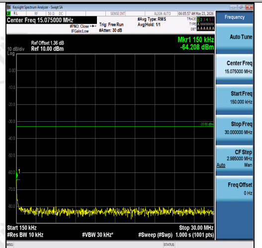
Band2-5MHz-QPSK-18900-1RB#0-0.15~30-PAS S
