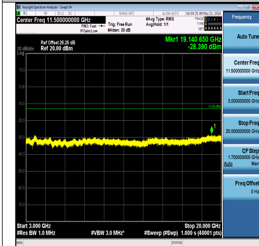
Band2-5MHz-16QAM-18900-1RB#24-3000~200 00-PASS
