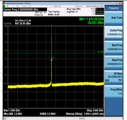
Band2-3MHz-16QAM-19185-1RB#14-1000~300 0-PASS
