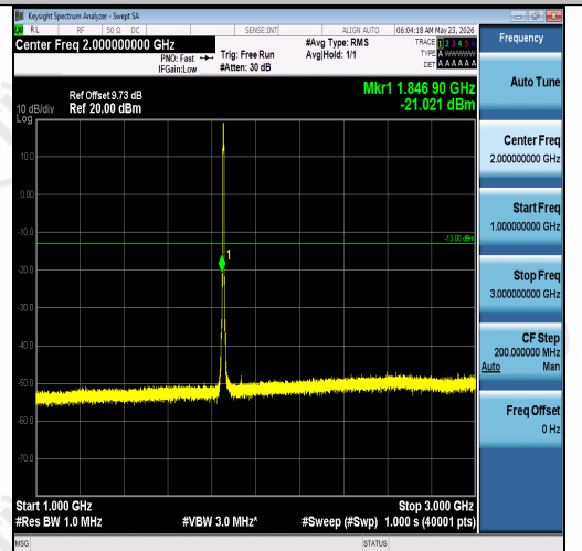
Band2-5MHz-QPSK-18625-25RB#0-1000~3000- PASS
