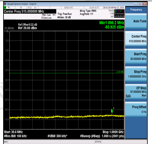
Band2-5MHz-16QAM-18625-1RB#0-30~1000-P ASS
