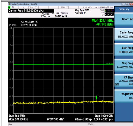
Band2-5MHz-QPSK-18900-1RB#0-30~1000-PA SS
