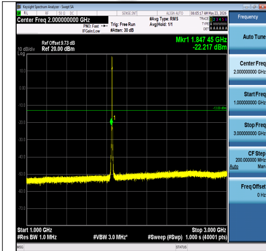
Band2-5MHz-16QAM-18625-25RB#0-1000~300 0-PASS
