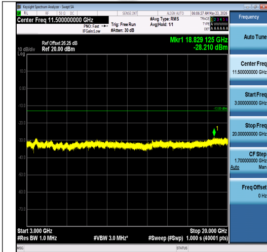
Band2-5MHz-QPSK-18900-1RB#0-3000~20000- PASS
