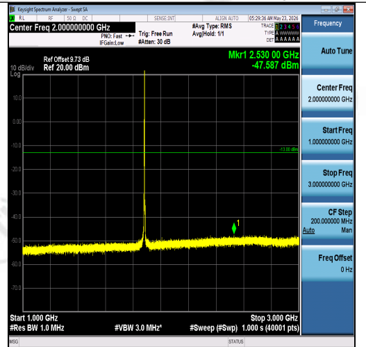
Band2-3MHz-16QAM-18900-1RB#14-1000~300 0-PASS
