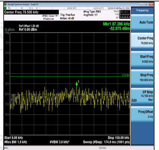
Band2-5MHz-16QAM-18625-25RB#0-0.009~0.1 5-PASS
