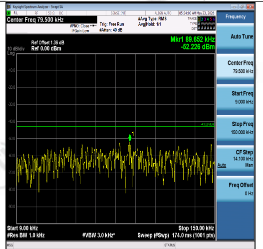
Band2-3MHz-QPSK-19185-1RB#14-0.009~0.15- PASS
