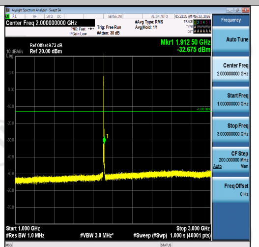
Band2-3MHz-QPSK-19185-1RB#0-1000~3000-P ASS
