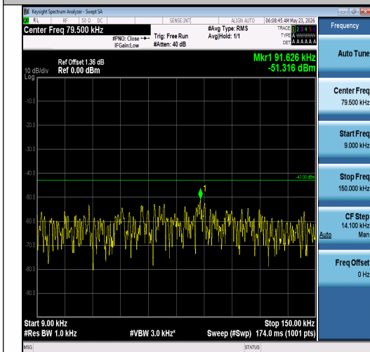
Band2-5MHz-16QAM-18900-1RB#24-0.009~0.1 5-PASS
