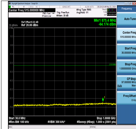
Band2-3MHz-16QAM-18900-1RB#14-30~1000-P ASS
