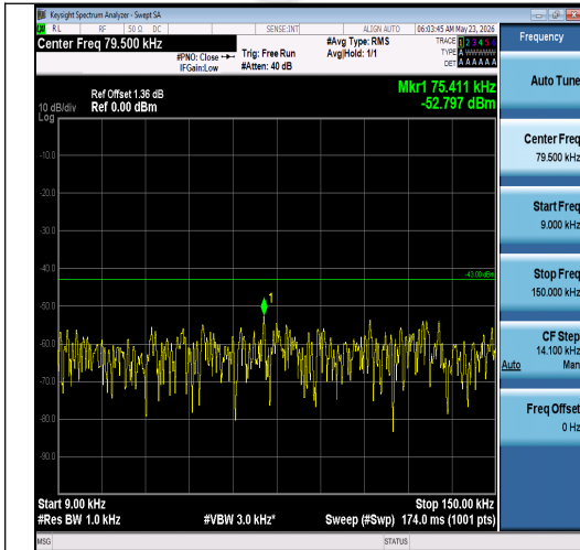
Band2-5MHz-QPSK-18625-25RB#0-0.009~0.15- PASS
