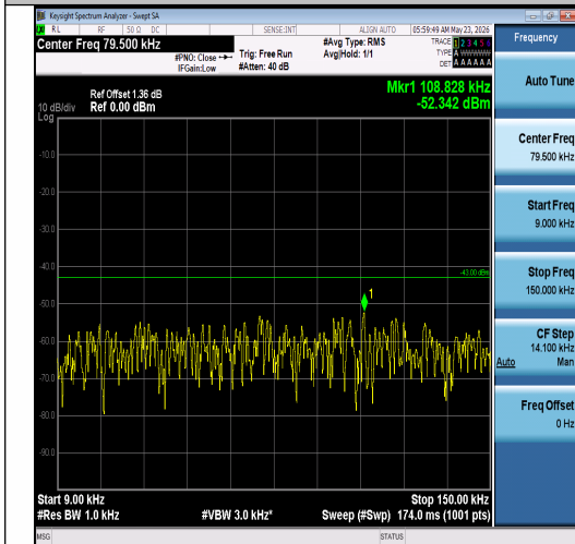
Band2-5MHz-QPSK-18625-1RB#0-0.009~0.15-P ASS
