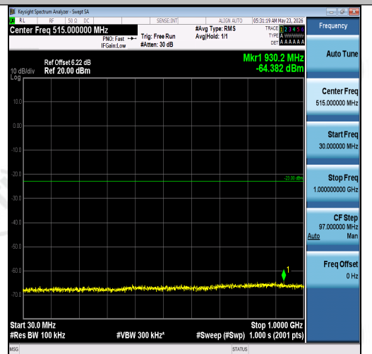
Band2-3MHz-16QAM-18900-15RB#0-30~1000-P ASS
