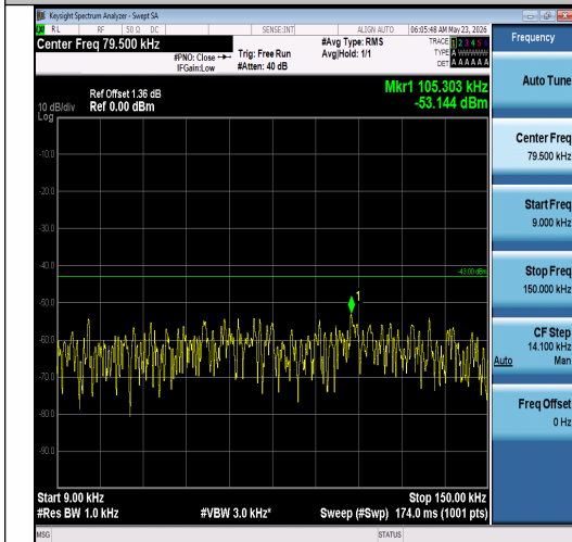
Band2-5MHz-QPSK-18900-1RB#0-0.009~0.15-P ASS
