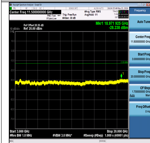
Band2-5MHz-QPSK-18625-25RB#0-3000~2000 0-PASS
