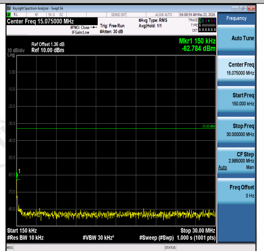
Band2-5MHz-16QAM-18900-1RB#24-0.15~30-P ASS
