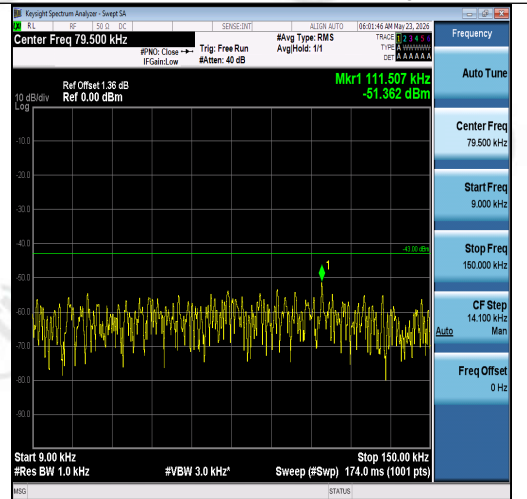
Band2-5MHz-QPSK-18625-1RB#24-0.009~0.15- PASS
