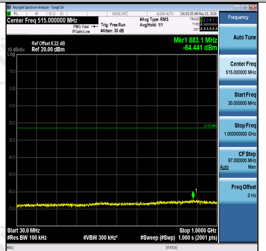
Band2-5MHz-QPSK-18625-1RB#24-30~1000-P ASS
