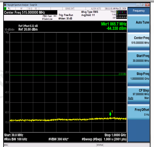
Band2-5MHz-16QAM-18900-25RB#0-30~1000-P ASS
