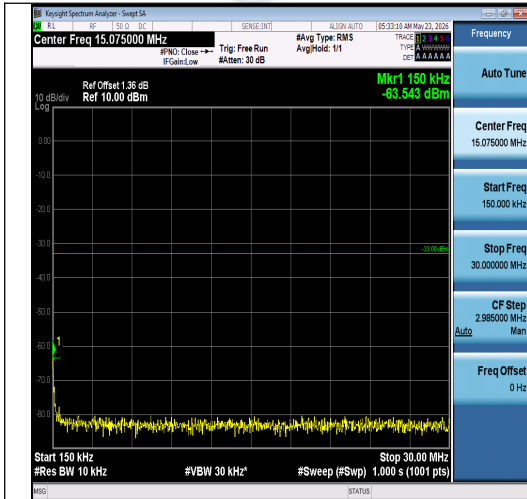
Band2-3MHz-16QAM-19185-1RB#0-0.15~30-PA SS
