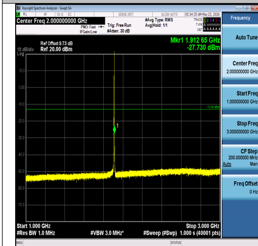
Band2-3MHz-QPSK-19185-1RB#14-1000~3000- PASS
