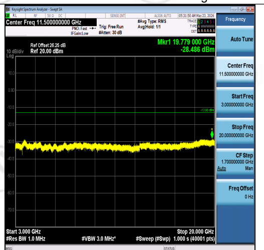
Band2-3MHz-16QAM-18900-15RB#0-3000~200 00-PASS
