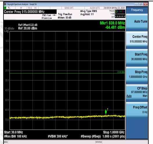
Band2-5MHz-QPSK-18900-1RB#24-30~1000-P ASS
