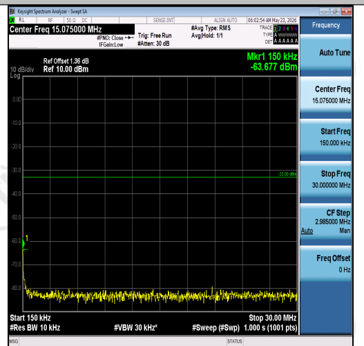
Band2-5MHz-16QAM-18625-1RB#24-0.15~30-P ASS
