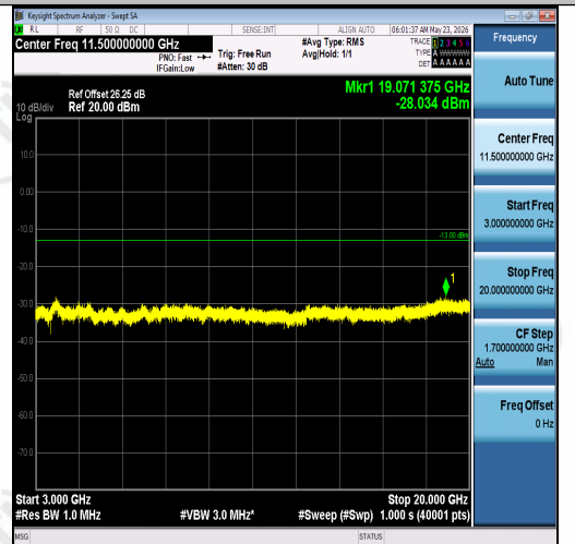
Band2-5MHz-16QAM-18625-1RB#0-3000~2000 0-PASS
