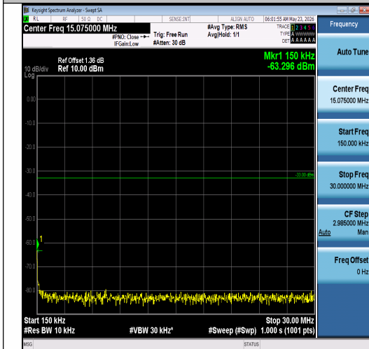
Band2-5MHz-QPSK-18625-1RB#24-0.15~30-PA SS
