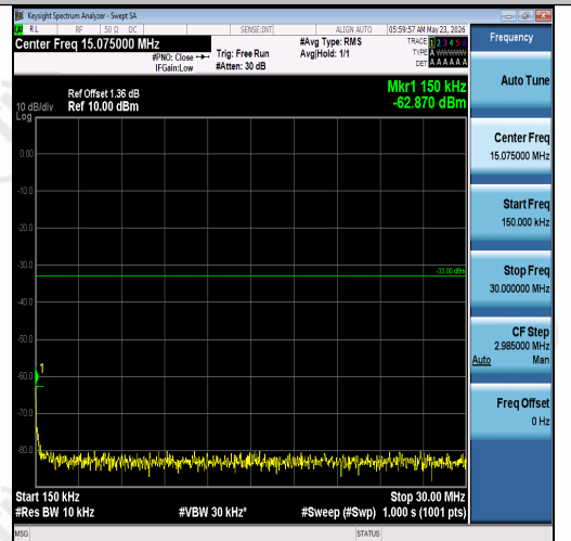
Band2-5MHz-QPSK-18625-1RB#0-0.15~30-PAS S
