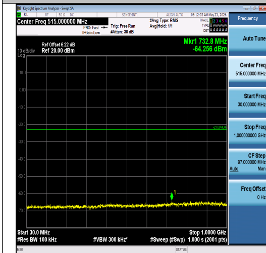
Band2-5MHz-QPSK-19175-1RB#0-30~1000-PA SS
