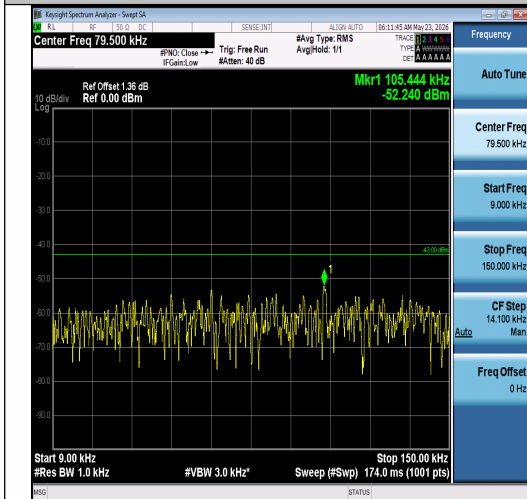
Band2-5MHz-QPSK-19175-1RB#0-0.009~0.15-P ASS
