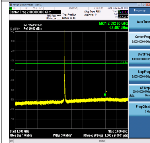
Band2-5MHz-QPSK-18900-1RB#24-1000~3000- PASS
