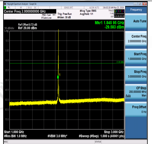
Band2-5MHz-16QAM-18625-1RB#24-1000~300 0-PASS
