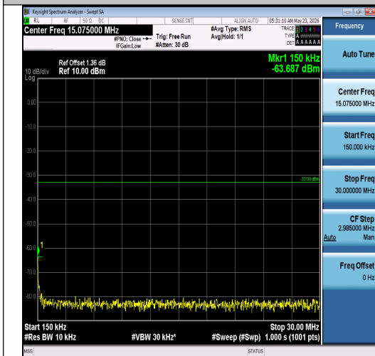
Band2-3MHz-16QAM-18900-15RB#0-0.15~30-P ASS
