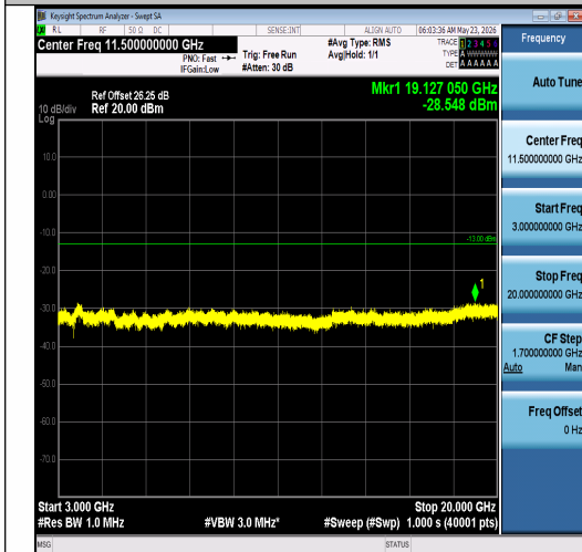
Band2-5MHz-16QAM-18625-1RB#24-3000~200 00-PASS
