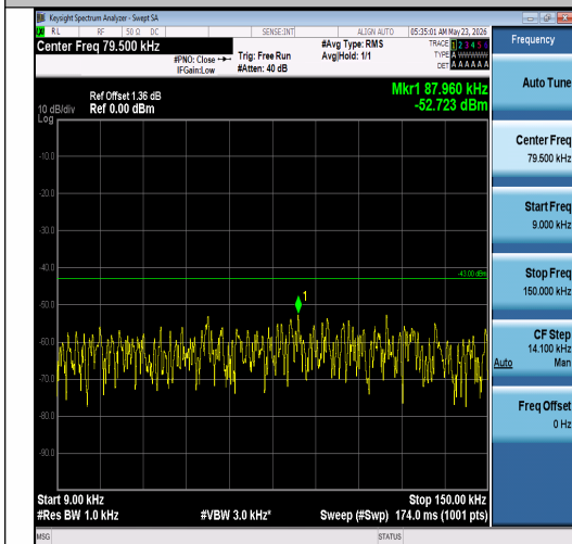
Band2-3MHz-16QAM-19185-1RB#14-0.009~0.1 5-PASS
