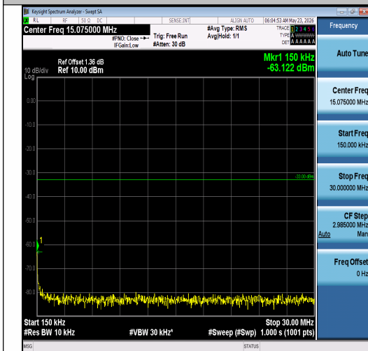
Band2-5MHz-16QAM-18625-25RB#0-0.15~30-P ASS
