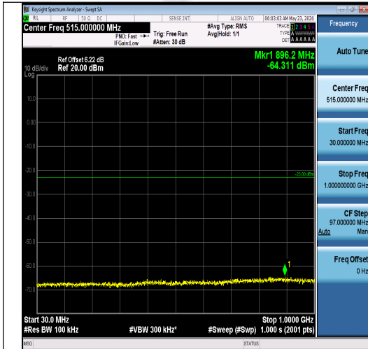
Band2-5MHz-16QAM-18625-1RB#24-30~1000-P ASS
