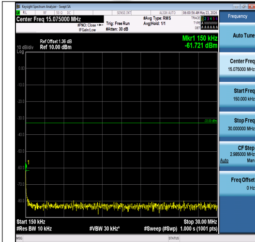
Band2-5MHz-16QAM-18625-1RB#0-0.15~30-PA SS
