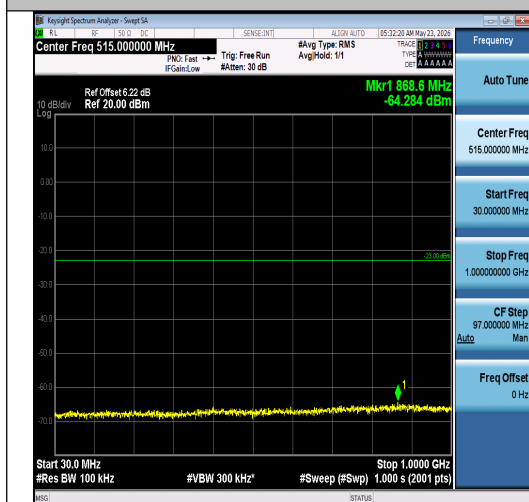
Band2-3MHz-QPSK-19185-1RB#0-30~1000-PA SS
