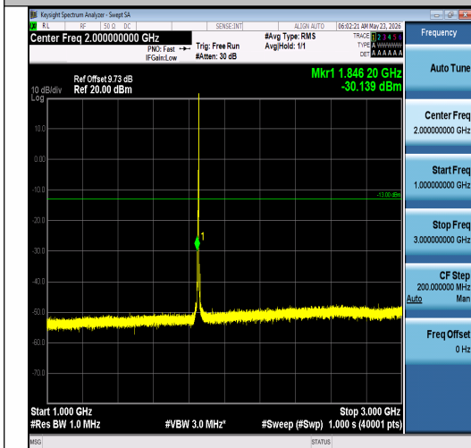
Band2-5MHz-QPSK-18625-1RB#24-1000~3000- PASS
