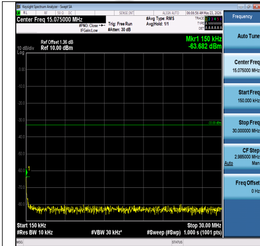
Band2-5MHz-16QAM-18900-1RB#0-0.15~30-PA SS
