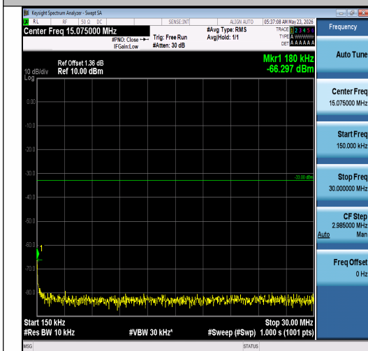
Band2-3MHz-16QAM-19185-15RB#0-0.15~30-P ASS
