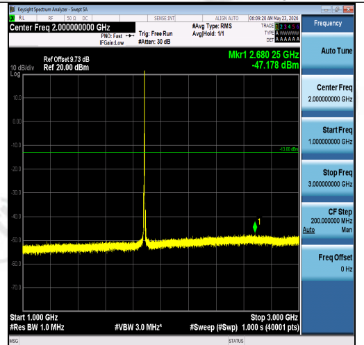
Band2-5MHz-16QAM-18900-1RB#24-1000~300 0-PASS
