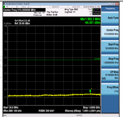
Band2-5MHz-16QAM-18625-25RB#0-30~1000-P ASS
