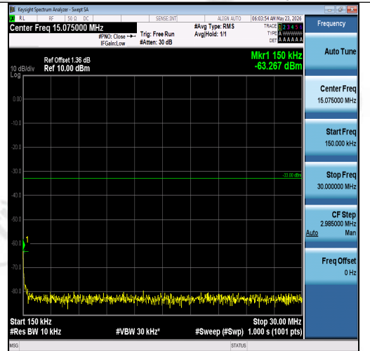
Band2-5MHz-QPSK-18625-25RB#0-0.15~30-PA SS
