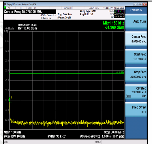
Band2-5MHz-QPSK-19175-1RB#0-0.15~30-PAS S
