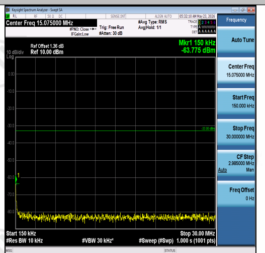
Band2-3MHz-QPSK-19185-1RB#0-0.15~30-PAS S
