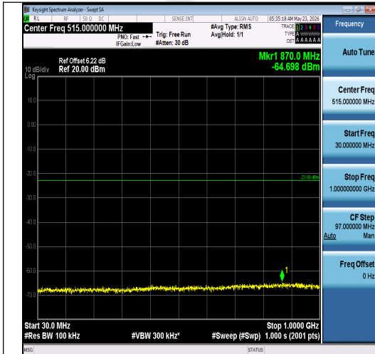
Band2-3MHz-16QAM-19185-1RB#14-30~1000-P ASS
