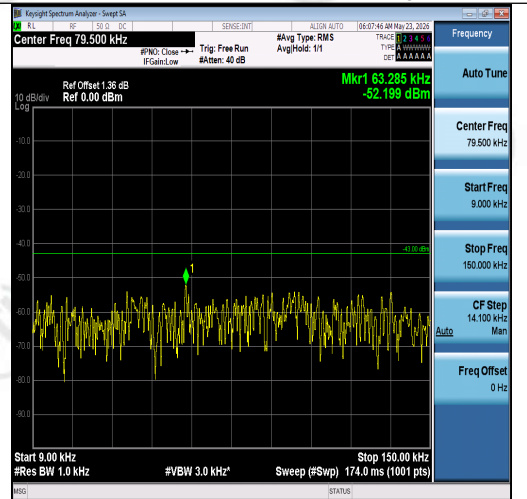
Band2-5MHz-QPSK-18900-1RB#24-0.009~0.15- PASS
