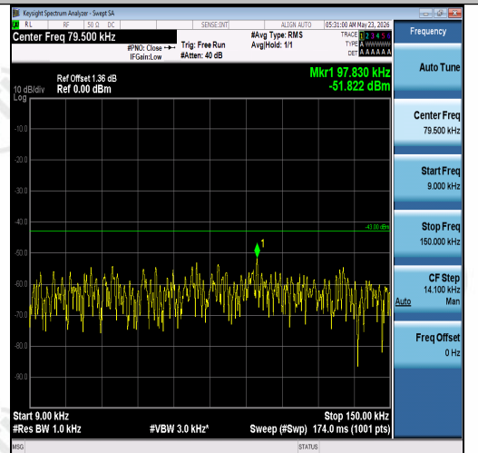
Band2-3MHz-16QAM-18900-15RB#0-0.009~0.1 5-PASS
