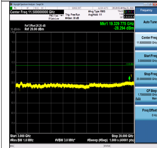
Band2-3MHz-16QAM-18900-1RB#14-3000~200 00-PASS
