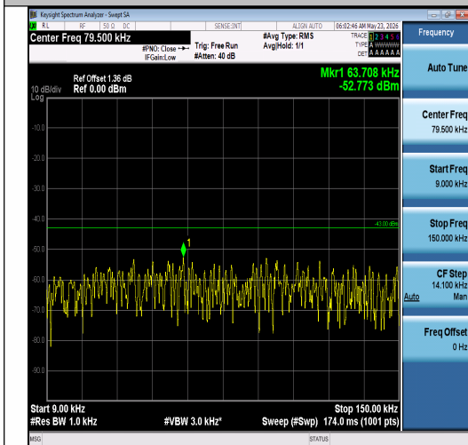
Band2-5MHz-16QAM-18625-1RB#24-0.009~0.1 5-PASS
