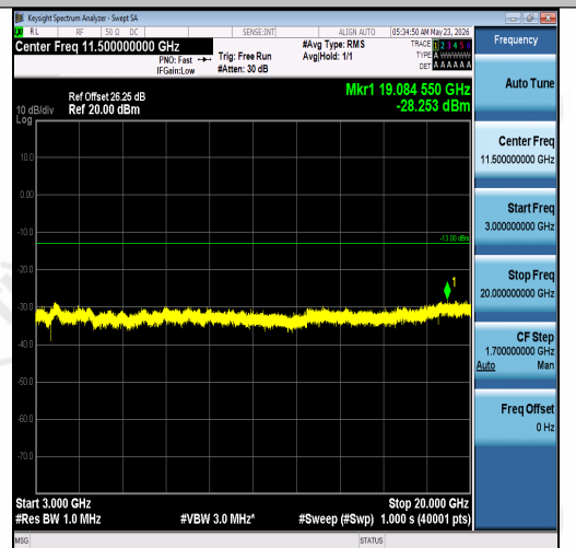
Band2-3MHz-QPSK-19185-1RB#14-3000~2000 0-PASS
