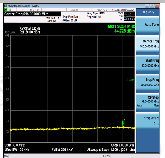
Band2-3MHz-16QAM-19185-15RB#0-30~1000-P ASS
