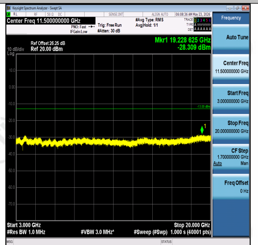
Band2-5MHz-QPSK-18900-1RB#24-3000~2000 0-PASS
