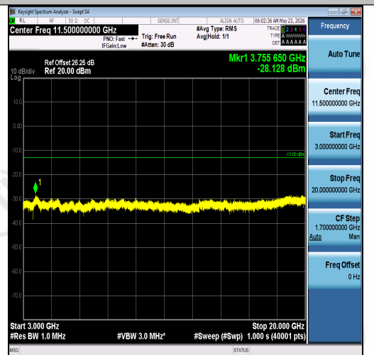
Band2-5MHz-QPSK-18625-1RB#24-3000~2000 0-PASS
