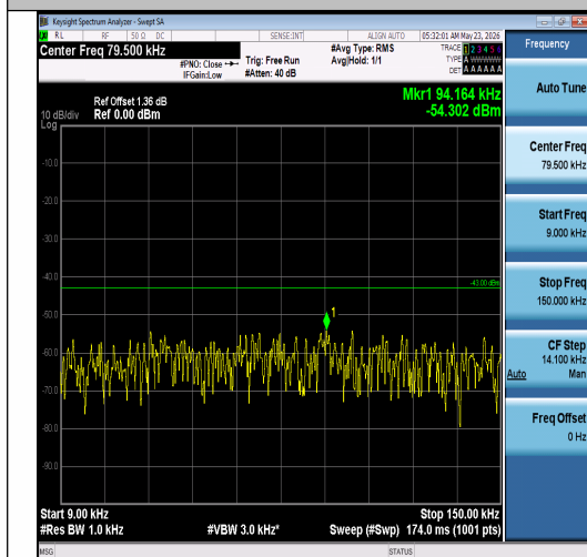
Band2-3MHz-QPSK-19185-1RB#0-0.009~0.15-P ASS
