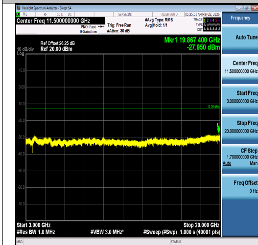
Band2-3MHz-16QAM-19185-1RB#14-3000~200 00-PASS
