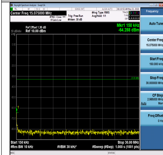
Band2-5MHz-16QAM-18900-25RB#0-0.15~30-P ASS
