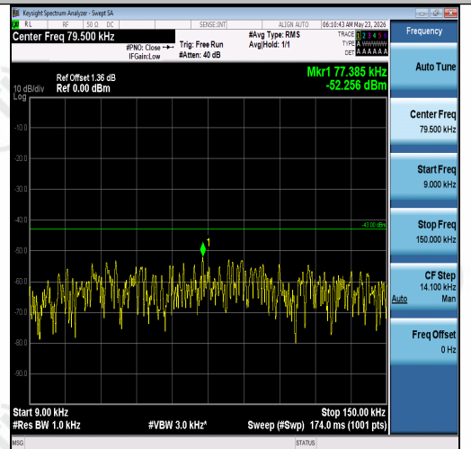
Band2-5MHz-16QAM-18900-25RB#0-0.009~0.1 5-PASS
