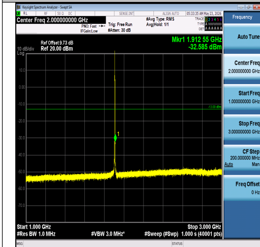
Band2-3MHz-16QAM-19185-1RB#0-1000~3000- PASS
