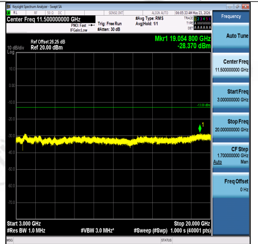
Band2-5MHz-16QAM-18625-25RB#0-3000~200 00-PASS
