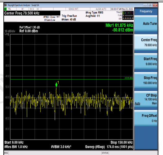
Band2-5MHz-16QAM-18625-1RB#0-0.009~0.15- PASS
