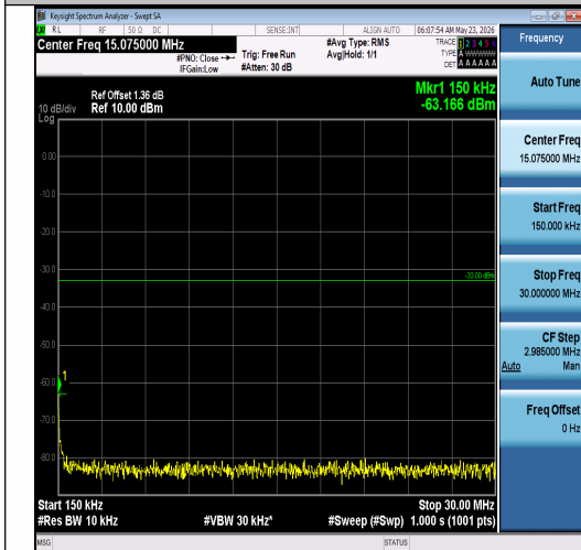
Band2-5MHz-QPSK-18900-1RB#24-0.15~30-PA SS
