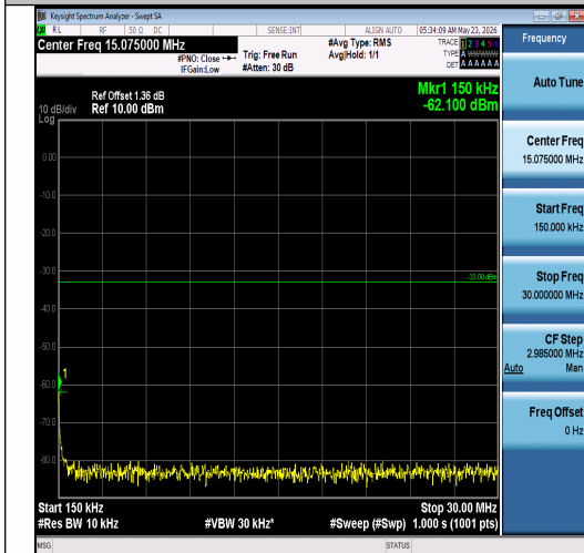
Band2-3MHz-QPSK-19185-1RB#14-0.15~30-PA SS
