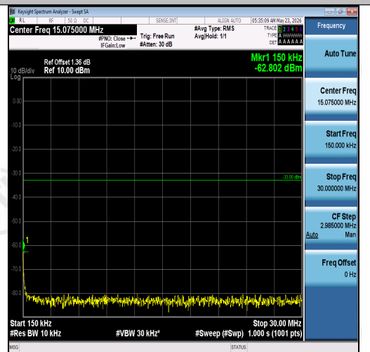
Band2-3MHz-16QAM-19185-1RB#14-0.15~30-P ASS
