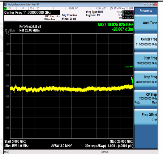
Band2-5MHz-16QAM-18900-1RB#0-3000~2000 0-PASS
