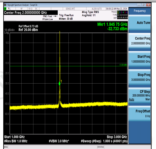
Band2-5MHz-QPSK-18625-1RB#0-1000~3000-P ASS
