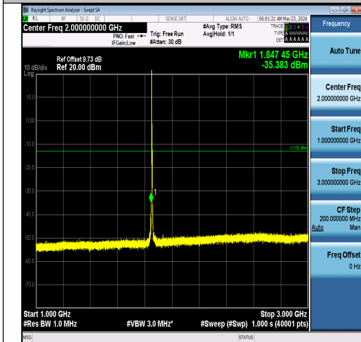
Band2-5MHz-16QAM-18625-1RB#0-1000~3000- PASS
