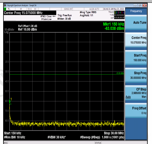
Band2-10MHz-16QAM-18900-1RB#49-0.15~30- PASS
