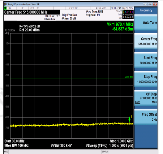
Band2-10MHz-16QAM-18900-1RB#0-30~1000-P ASS
