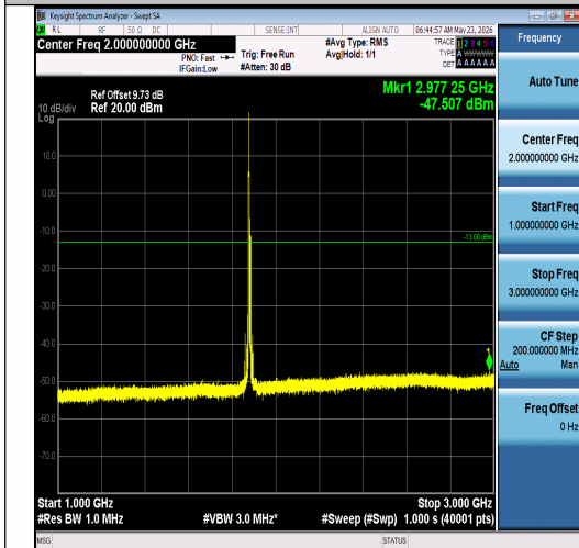
Band2-10MHz-16QAM-18900-1RB#0-1000~300 0-PASS
