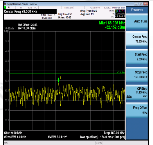
Band2-15MHz-QPSK-18675-1RB#74-0.009~0.1 5-PASS
