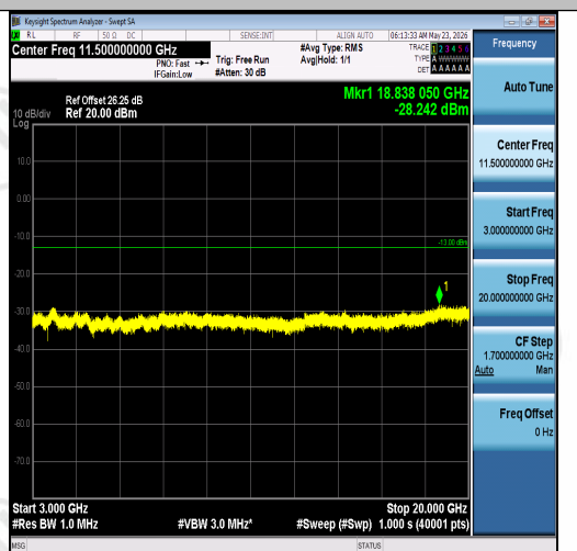
Band2-5MHz-16QAM-19175-1RB#0-3000~2000 0-PASS
