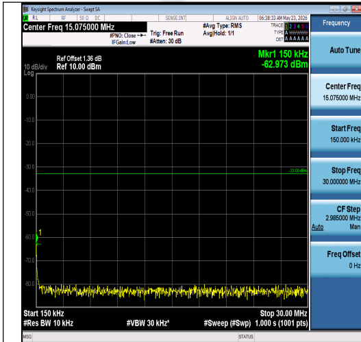
Band2-10MHz-16QAM-18650-1RB#0-0.15~30-P ASS
