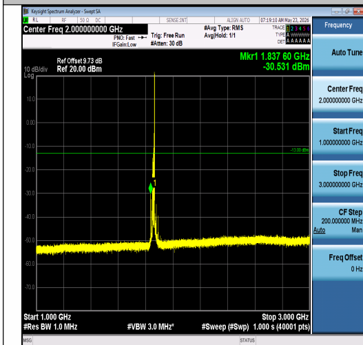
Band2-15MHz-QPSK-18675-1RB#74-1000~300 0-PASS
