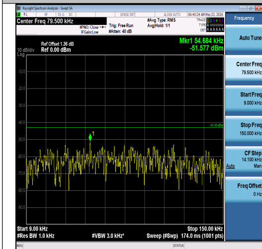
Band2-10MHz-16QAM-18650-1RB#49-0.009~0. 15-PASS
