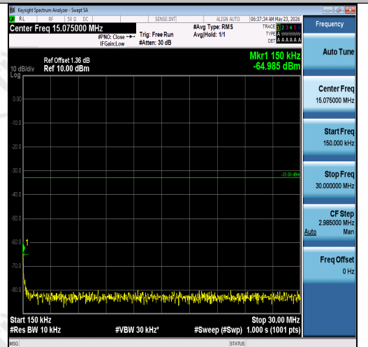
Band2-10MHz-QPSK-18650-1RB#0-0.15~30-PA SS
