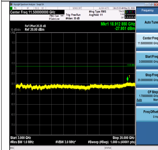
Band2-5MHz-16QAM-19175-1RB#24-3000~200 00-PASS
