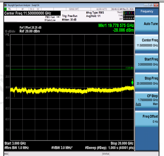
Band2-10MHz-QPSK-18900-1RB#49-3000~200 00-PASS
