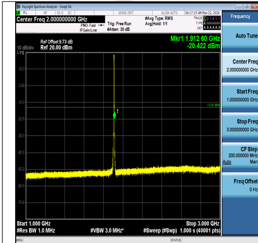
Band2-5MHz-16QAM-19175-25RB#0-1000~300 0-PASS
