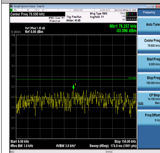
Band2-5MHz-16QAM-19175-1RB#24-0.009~0.1 5-PASS
