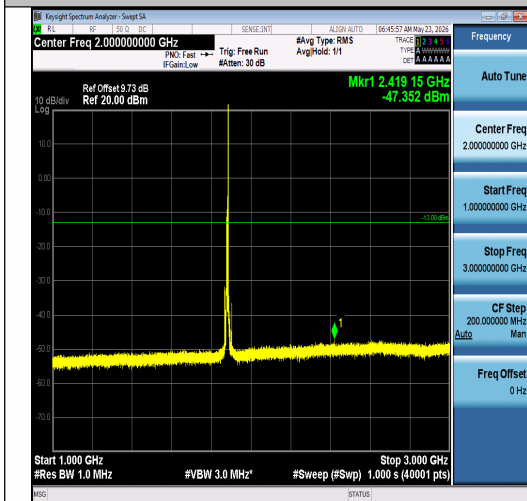
Band2-10MHz-QPSK-18900-1RB#49-1000~300 0-PASS
