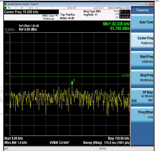
Band2-10MHz-QPSK-18900-1RB#49-0.009~0.1 5-PASS
