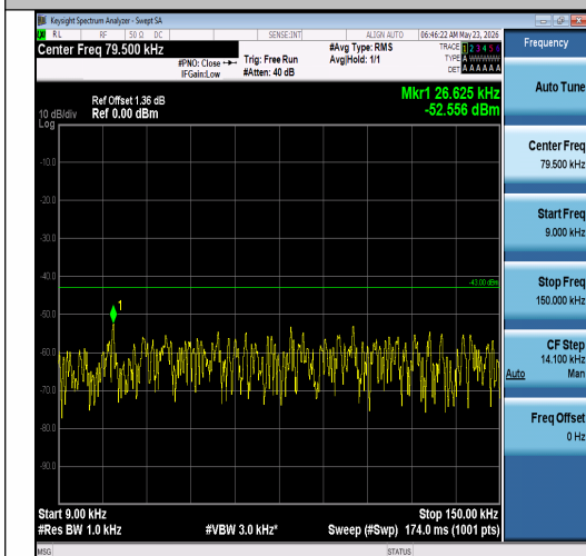
Band2-10MHz-16QAM-18900-1RB#49-0.009~0. 15-PASS
