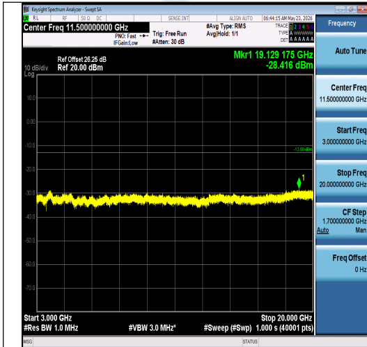
Band2-10MHz-QPSK-18900-1RB#0-3000~2000 0-PASS
