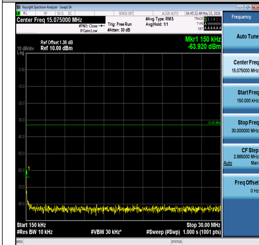
Band2-10MHz-QPSK-18900-1RB#49-0.15~30-P ASS
