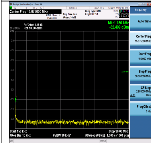
Band2-15MHz-QPSK-18675-1RB#74-0.15~30-P ASS
