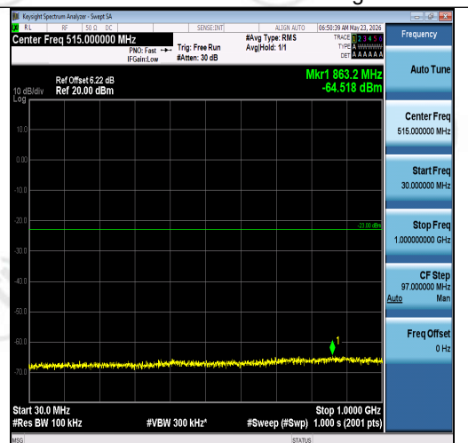
Band2-10MHz-16QAM-19150-1RB#0-30~1000-P ASS
