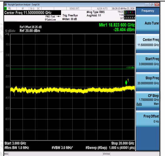
Band2-10MHz-16QAM-18650-1RB#0-3000~200 00-PASS
