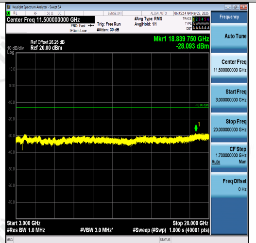
Band2-10MHz-16QAM-18900-1RB#0-3000~200 00-PASS
