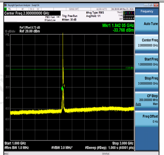
Band2-10MHz-QPSK-18650-1RB#0-1000~3000- PASS
