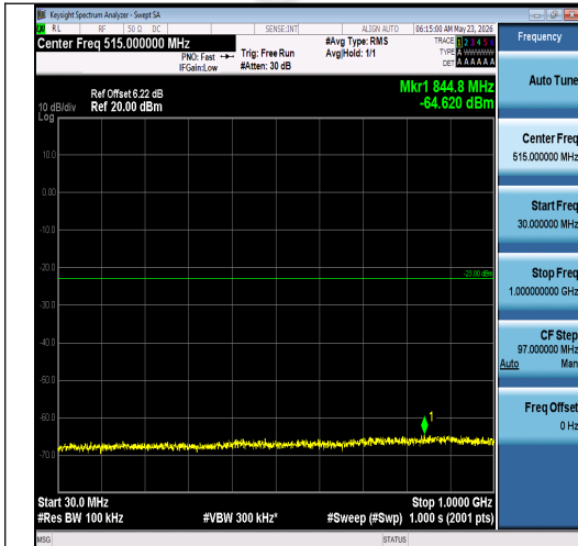
Band2-5MHz-16QAM-19175-1RB#24-30~1000-P ASS
