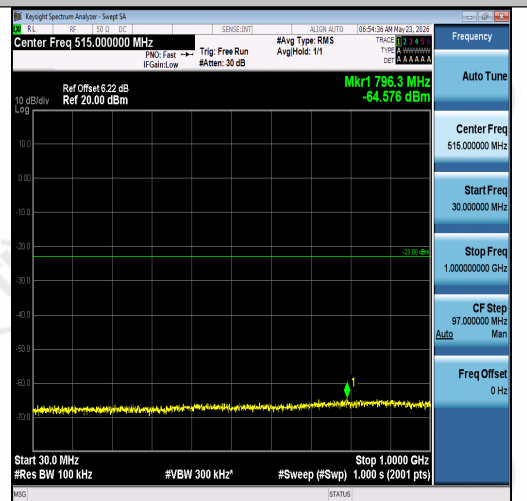
Band2-10MHz-16QAM-19150-50RB#0-30~1000-PASS
