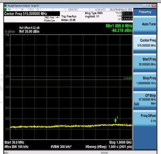
Band2-5MHz-16QAM-19175-25RB#0-30~1000-P ASS
