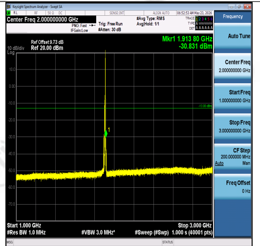
Band2-10MHz-16QAM-19150-1RB#49-1000~3000-PASS
