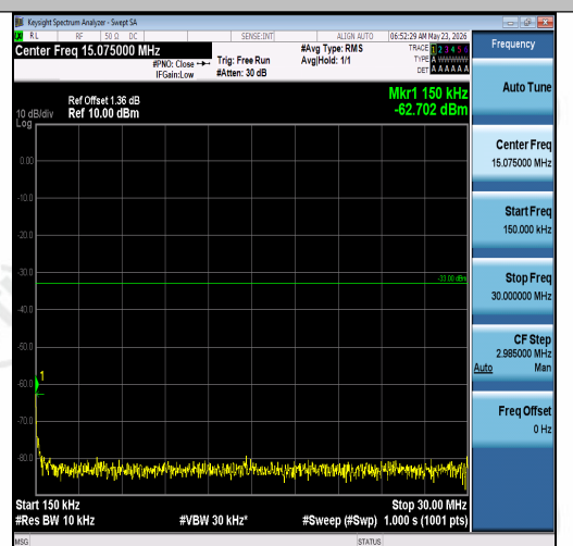
Band2-10MHz-16QAM-19150-1RB#49-0.15~30- PASS
