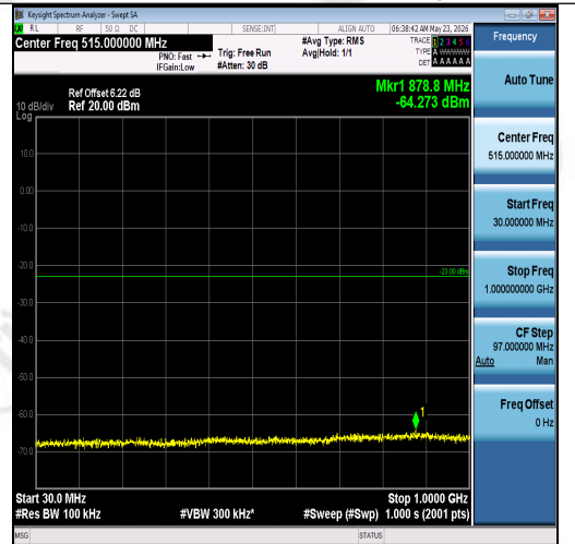
Band2-10MHz-16QAM-18650-1RB#0-30~1000-P ASS
