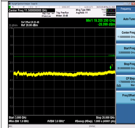
Band2-10MHz-16QAM-19150-1RB#49-3000~20000-PASS
