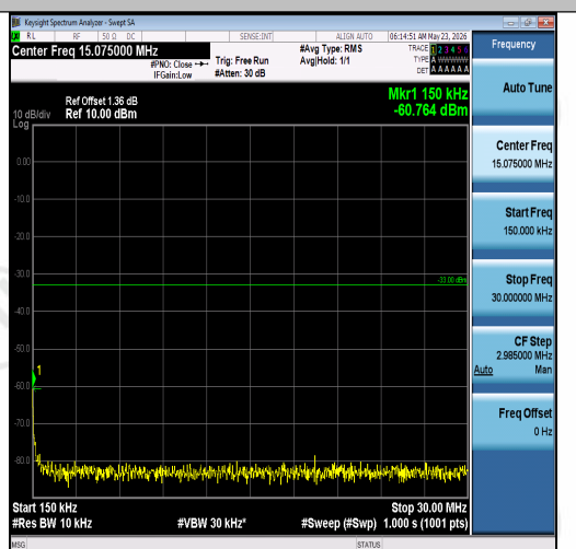
Band2-5MHz-16QAM-19175-1RB#24-0.15~30-P ASS
