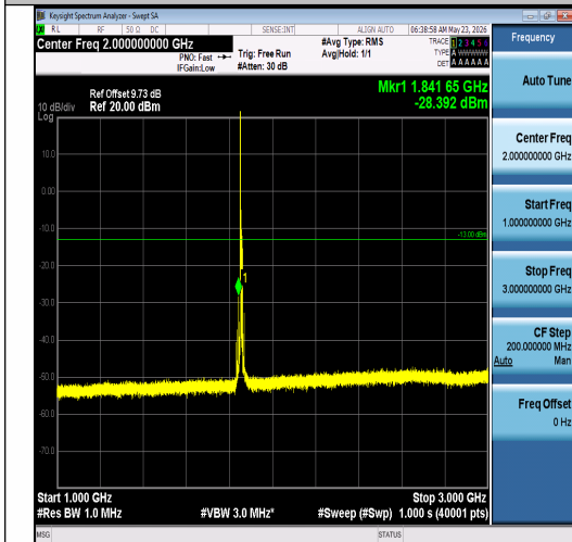
Band2-10MHz-16QAM-18650-1RB#0-1000~300 0-PASS
