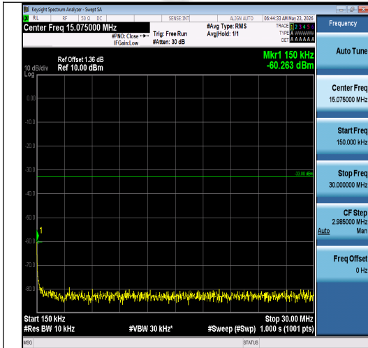
Band2-10MHz-16QAM-18900-1RB#0-0.15~30-P ASS
