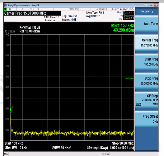
Band2-10MHz-16QAM-18650-1RB#49-0.15~30- PASS
