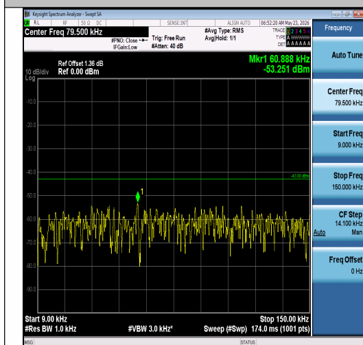
Band2-10MHz-16QAM-19150-1RB#49-0.009~0. 15-PASS
