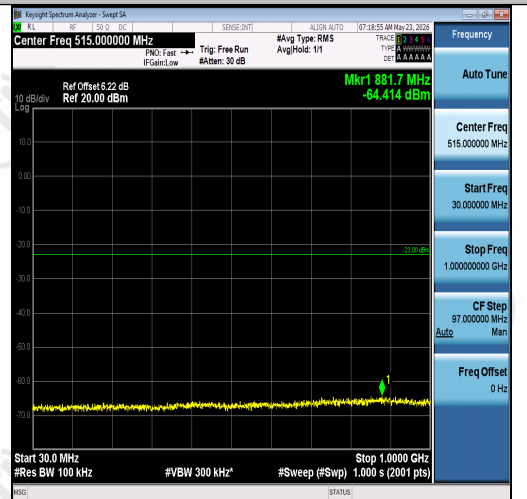
Band2-15MHz-QPSK-18675-1RB#74-30~1000-P ASS
