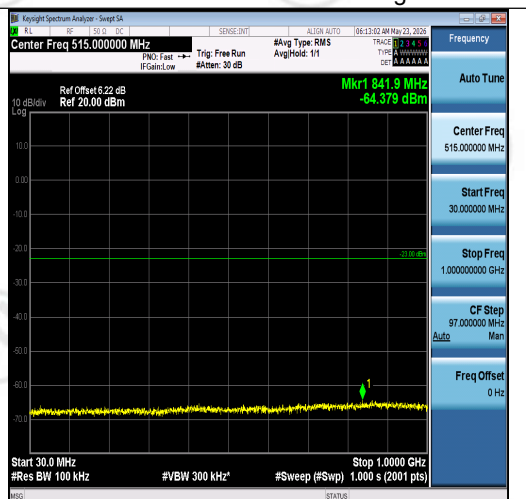
Band2-5MHz-16QAM-19175-1RB#0-30~1000-P ASS
