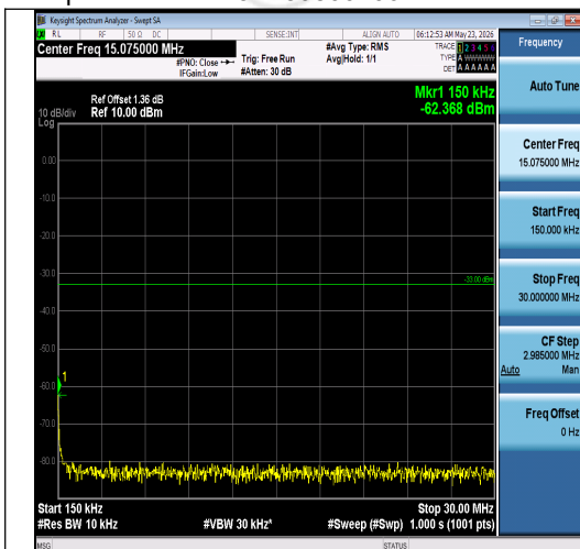
Band2-5MHz-16QAM-19175-1RB#0-0.15~30-PA SS
