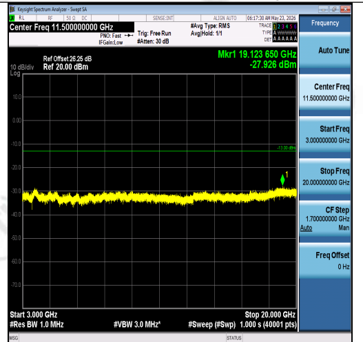
Band2-5MHz-16QAM-19175-25RB#0-3000~200 00-PASS
