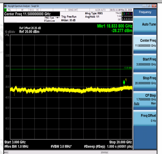
Band2-10MHz-16QAM-19150-1RB#0-3000~200 00-PASS
