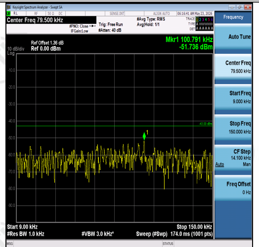
Band2-5MHz-16QAM-19175-25RB#0-0.009~0.1 5-PASS
