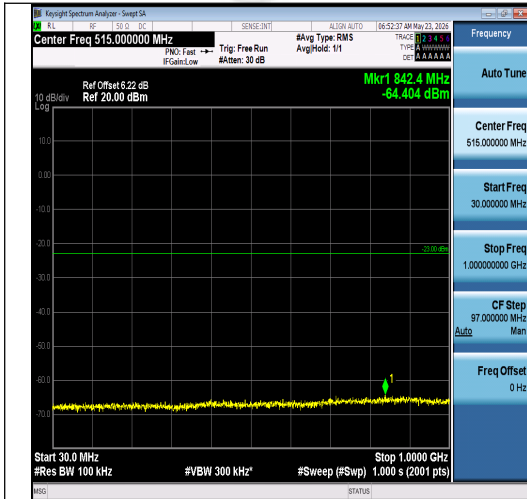
Band2-10MHz-16QAM-19150-1RB#49-30~1000-PASS
