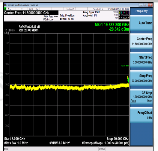
Band2-15MHz-QPSK-18675-1RB#74-3000~200 00-PASS
