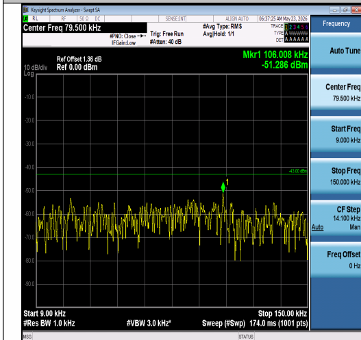
Band2-10MHz-QPSK-18650-1RB#0-0.009~0.15- PASS
