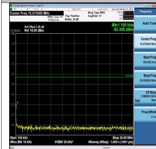
Band2-5MHz-16QAM-19175-25RB#0-0.15~30-P ASS
