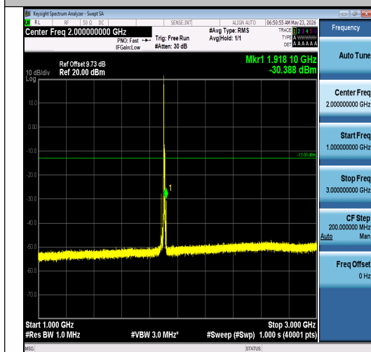
Band2-10MHz-16QAM-19150-1RB#0-1000~300 0-PASS
