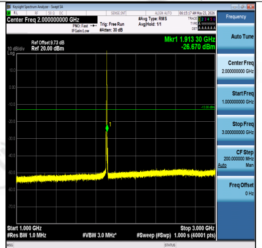
Band2-5MHz-16QAM-19175-1RB#24-1000~300 0-PASS
