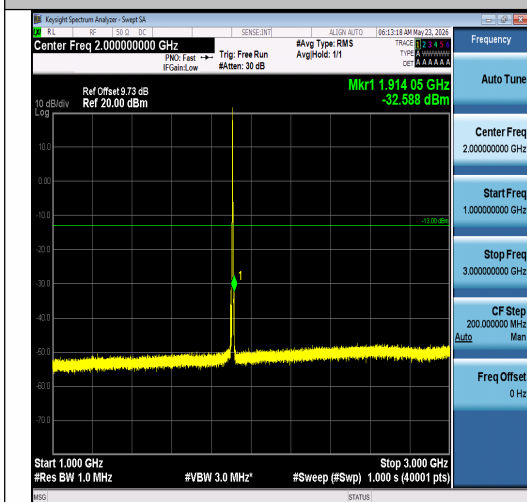
Band2-5MHz-16QAM-19175-1RB#0-1000~3000- PASS
