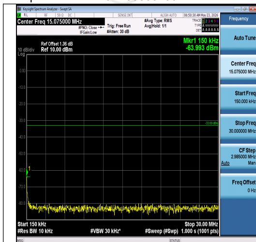
Band2-10MHz-16QAM-19150-1RB#0-0.15~30-P ASS
