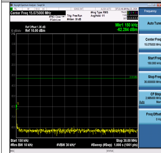
Band2-15MHz-16QAM-18675-75RB#0-0.15~30- PASS
