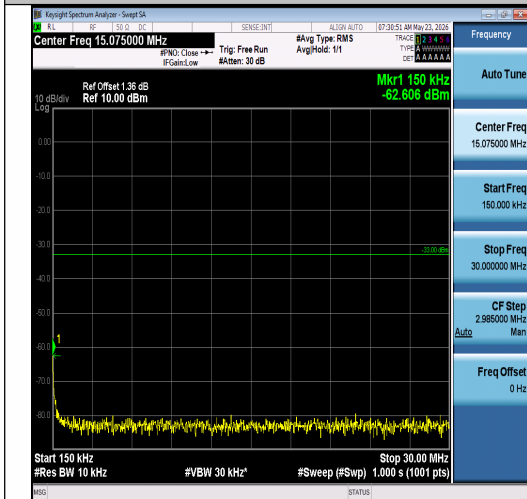
Band2-15MHz-QPSK-19125-1RB#74-0.15~30-P ASS
