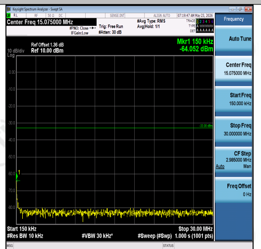
Band2-15MHz-16QAM-18675-1RB#74-0.15~30-PASS
