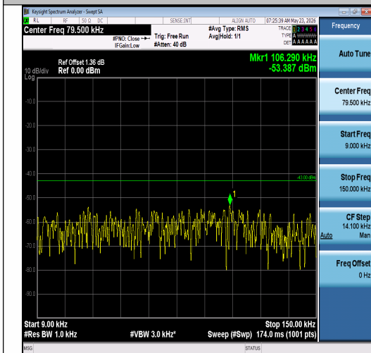
Band2-15MHz-16QAM-18900-1RB#74-0.009~0. 15-PASS
