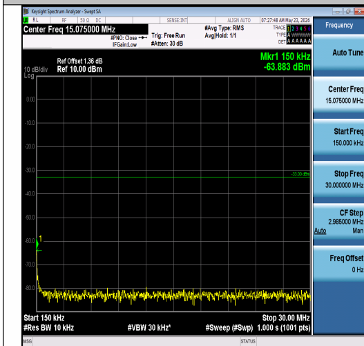
Band2-15MHz-16QAM-18900-75RB#0-0.15~30- PASS
