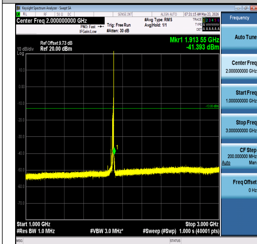
Band2-15MHz-QPSK-19125-1RB#74-1000~300 0-PASS
