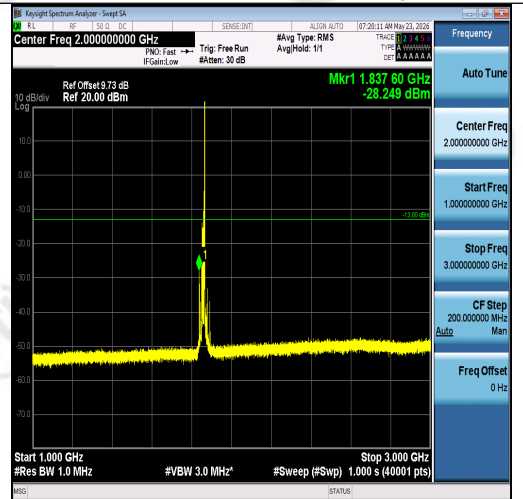
Band2-15MHz-16QAM-18675-1RB#74-1000~30 00-PASS
