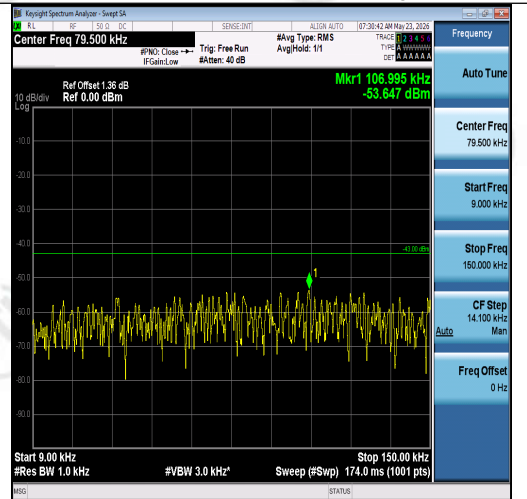
Band2-15MHz-QPSK-19125-1RB#74-0.009~0.1 5-PASS
