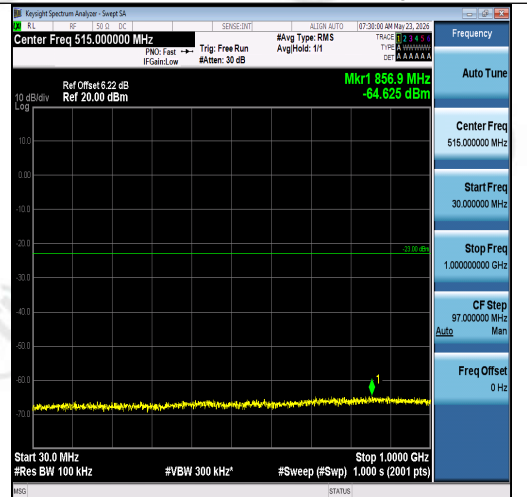
Band2-15MHz-16QAM-19125-1RB#0-30~1000-P ASS
