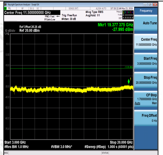
Band2-15MHz-16QAM-19125-1RB#0-3000~200 00-PASS
