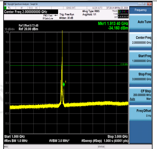
Band2-15MHz-16QAM-18900-1RB#74-1000~3000- 00-PASS
