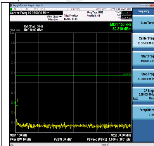
Band2-20MHz-16QAM-18700-1RB#0-0.15~30-P ASS
