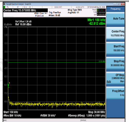
Band2-15MHz-16QAM-18900-1RB#74-0.15~30- PASS
