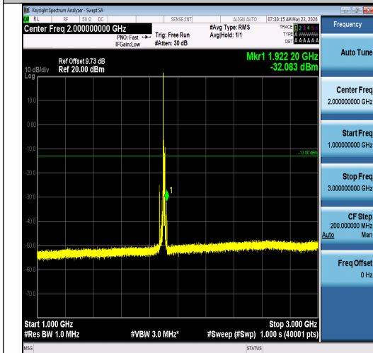
Band2-15MHz-16QAM-19125-1RB#0-1000~300 0-PASS
