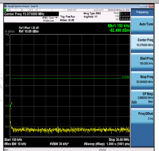
Band2-20MHz-16QAM-18700-1RB#99-0.15~30- PASS
