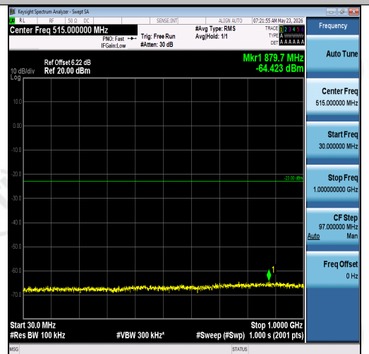
Band2-15MHz-16QAM-18675-75RB#0-30~1000- PASS
