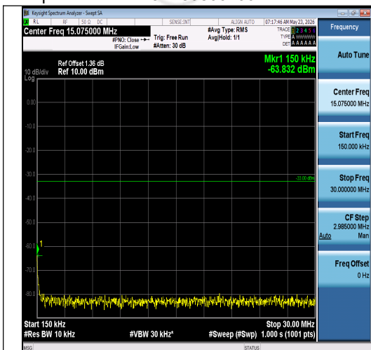
Band2-15MHz-16QAM-18675-1RB#0-0.15~30-P ASS
