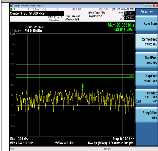
Band2-15MHz-16QAM-18675-1RB#74-0.009~0. 15-PASS
