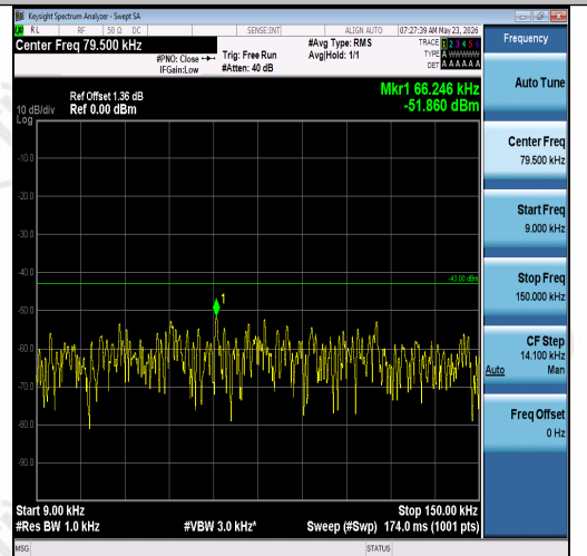
Band2-15MHz-16QAM-18900-75RB#0-0.009~0.15- 15-PASS
