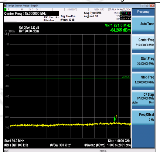
Band2-20MHz-16QAM-18700-1RB#0-30~1000-P ASS
