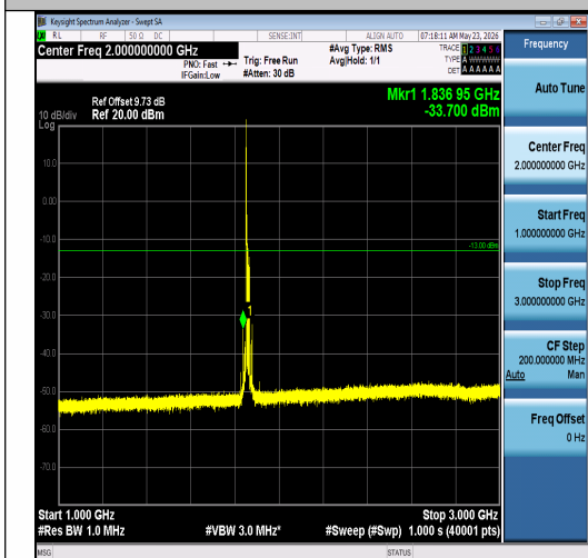
Band2-15MHz-16QAM-18675-1RB#0-1000~300 0-PASS
