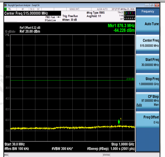
Band2-15MHz-16QAM-18900-75RB#0-30~1000- PASS
