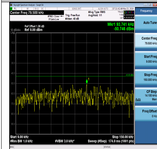
Band2-15MHz-16QAM-19125-1RB#74-0.009~0. 15-PASS
