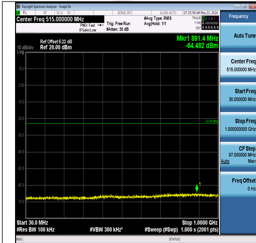
Band2-15MHz-16QAM-18900-1RB#74-30~1000- PASS
