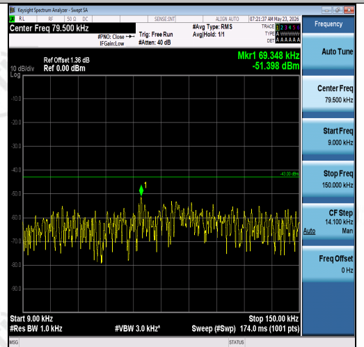
Band2-15MHz-16QAM-18675-75RB#0-0.009~0. 15-PASS
