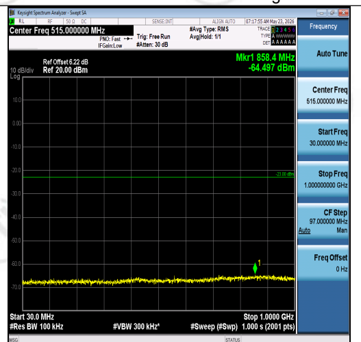
Band2-15MHz-16QAM-18675-1RB#0-30~1000-P ASS
