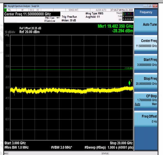
Band2-15MHz-16QAM-18675-1RB#0-3000~200 00-PASS
