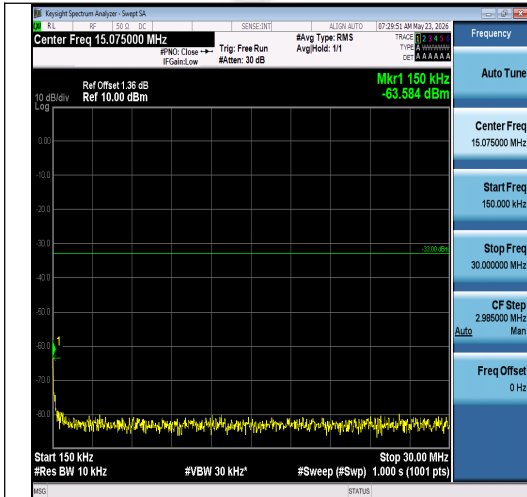
Band2-15MHz-16QAM-19125-1RB#0-0.15~30-P ASS
