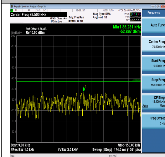
Band2-20MHz-16QAM-18700-1RB#99-0.009~0. 15-PASS
