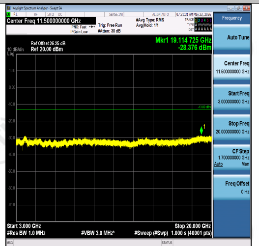
Band2-15MHz-QPSK-19125-1RB#74-3000~200 00-PASS
