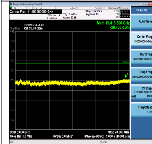
Band2-15MHz-16QAM-18900-1RB#74-3000~20000- 000-PASS
