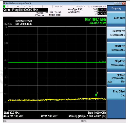
Band2-15MHz-16QAM-18900-1RB#0-30~1000-P ASS
