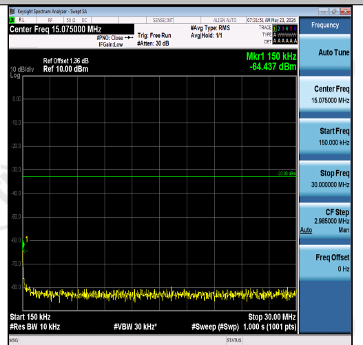
Band2-15MHz-16QAM-19125-1RB#74-0.15~30- PASS
