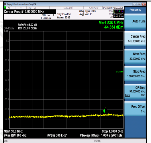
Band2-15MHz-QPSK-19125-1RB#74-30~1000-P ASS
