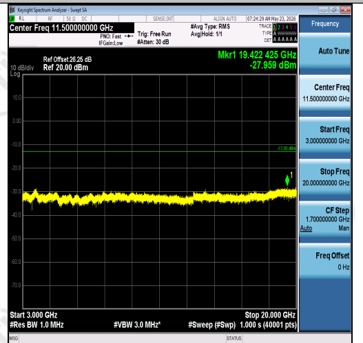
Band2-15MHz-16QAM-18900-1RB#0-3000~200 00-PASS
