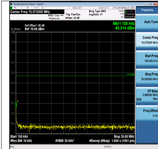
Band2-15MHz-16QAM-18900-1RB#0-0.15~30-P ASS
