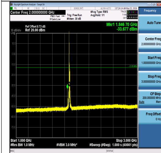
Band2-15MHz-16QAM-18900-1RB#0-1000~300 0-PASS
