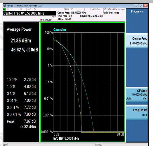
Band26(814-824)-5MHz-16QAM-26715-25RB#0 -PASS
