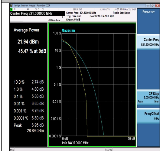
Band26(814-824)-5MHz-16QAM-26765-1RB#0- PASS
