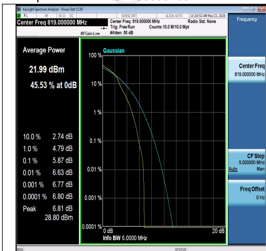
Band26(814-824)-5MHz-16QAM-26740-1RB#0- PASS
