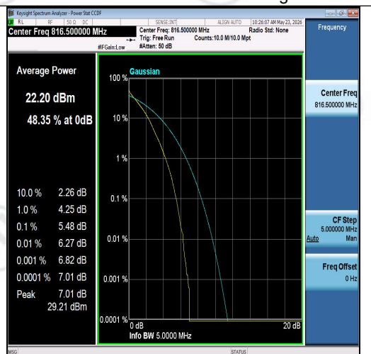
Band26(814-824)-5MHz-QPSK-26715-25RB#0-P ASS
