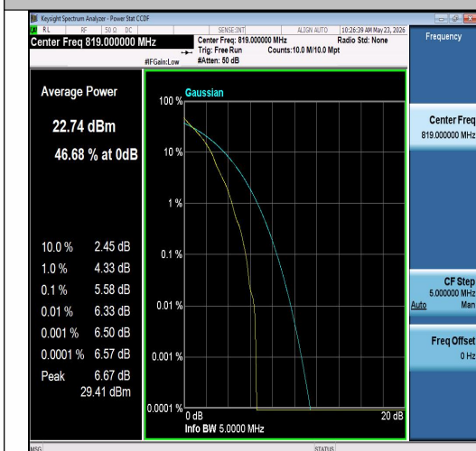
Band26(814-824)-5MHz-QPSK-26740-1RB#0-P ASS
