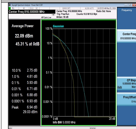
Band26(814-824)-5MHz-16QAM-26715-1RB#0-0 PASS
