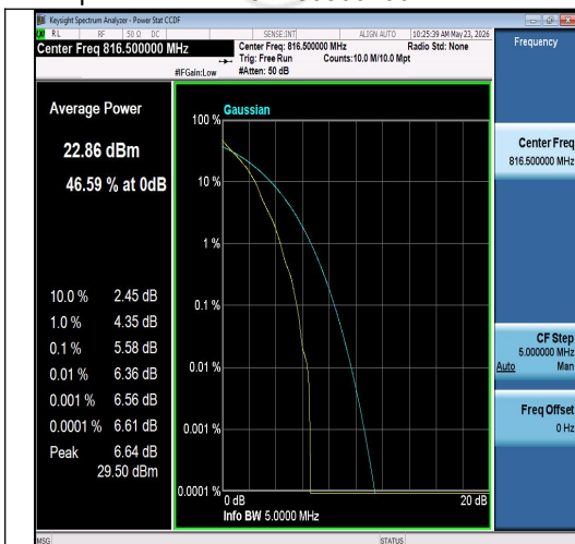
Band26(814-824)-5MHz-QPSK-26715-1RB#0-P ASS
