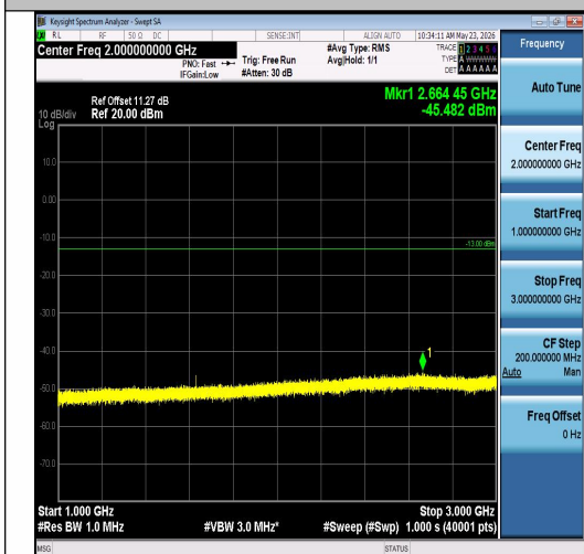
Band26(814-824)-10MHz-16QAM-26740-1RB#0 -1000~3000-PASS
