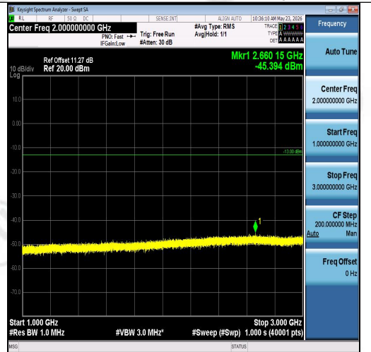
Band26(814-824)-10MHz-16QAM-26740-1RB#4 9-1000~3000-PASS
