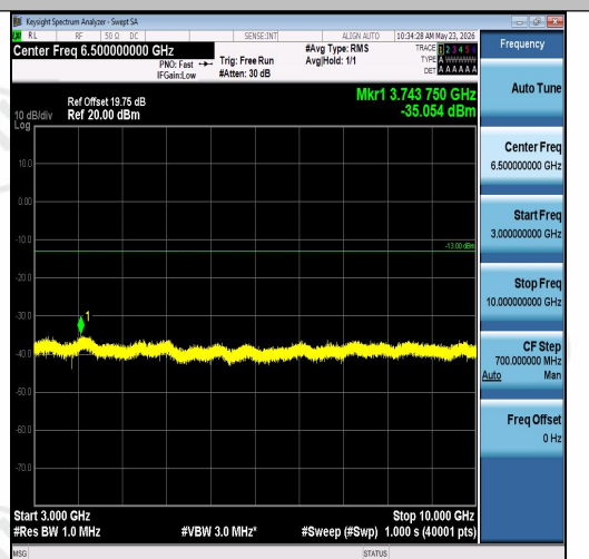
Band26(814-824)-10MHz-16QAM-26740-1RB#0 -3000~10000-PASS
