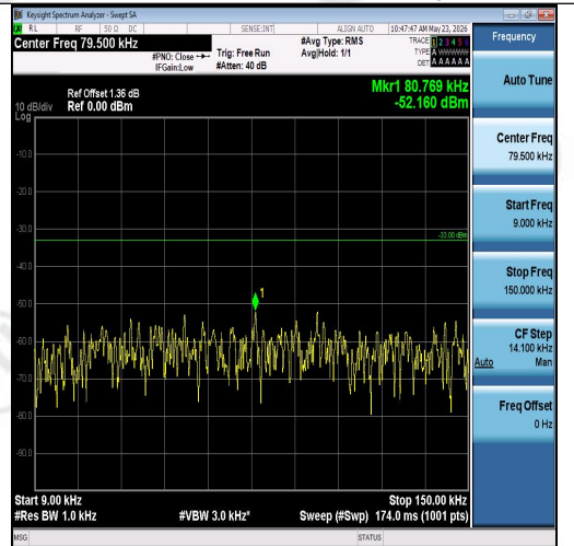
Band26(814-824)-15MHz-QPSK-26765-1RB#74- 0.009~0.15-PASS
