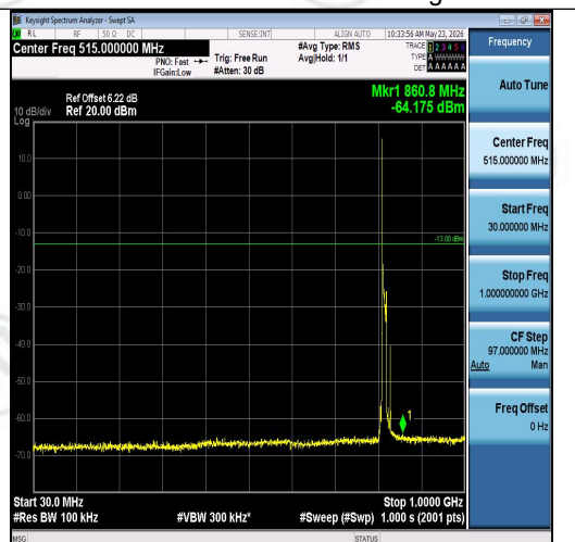
Band26(814-824)-10MHz-16QAM-26740-1RB#0 -30~1000-PASS
