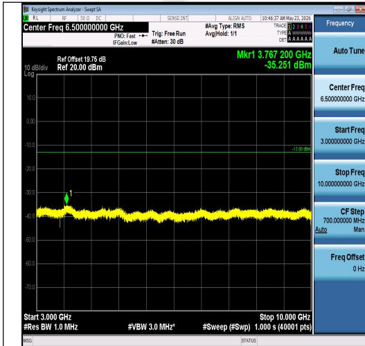
Band26(814-824)-15MHz-QPSK-26765-1RB#0-3 000~10000-PASS
