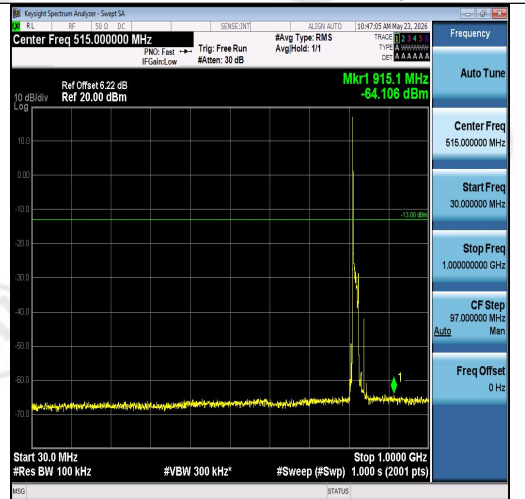
Band26(814-824)-15MHz-16QAM-26765-1RB#0 -30~1000-PASS
