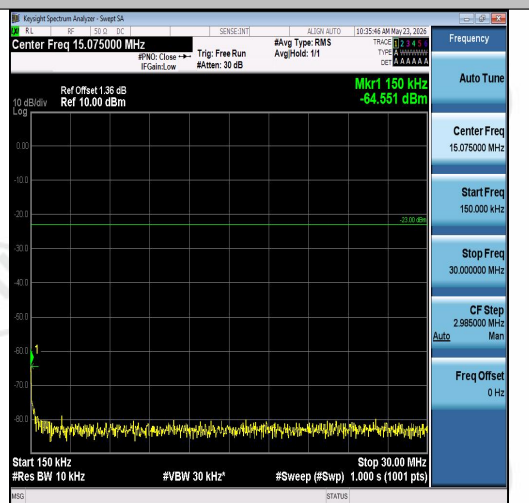
Band26(814-824)-10MHz-16QAM-26740-1RB#4 9-0.15~30-PASS
