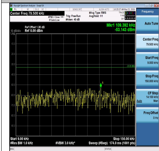
Band26(814-824)-10MHz-16QAM-26740-1RB#4 9-0.009~0.15-PASS
