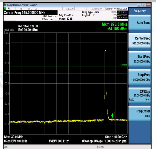
Band26(814-824)-10MHz-16QAM-26740-50RB#4 0-30~1000-PASS
