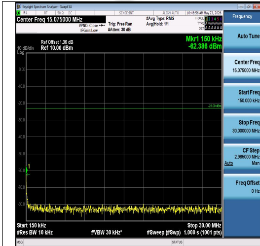
Band26(814-824)-15MHz-16QAM-26765-1RB#0 -0.15~30-PASS
