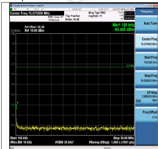
Band26(814-824)-10MHz-16QAM-26740-1RB#0 -0.15~30-PASS
