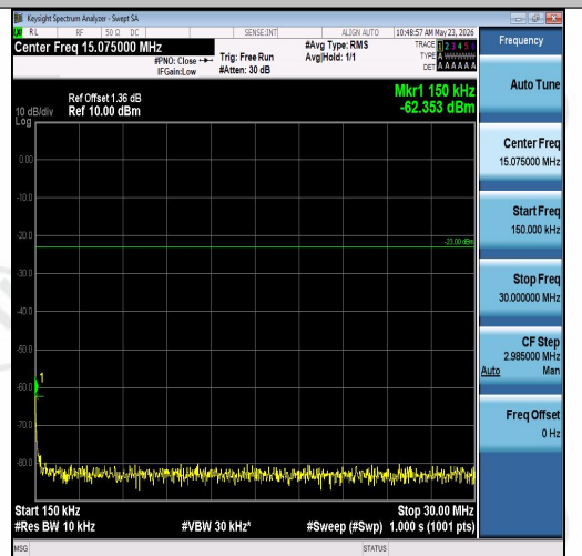
Band26(814-824)-15MHz-16QAM-26765-1RB#7 4-0.15~30-PASS
