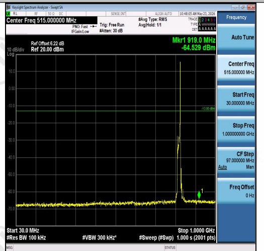
Band26(814-824)-15MHz-QPSK-26765-1RB#74- 30~1000-PASS
