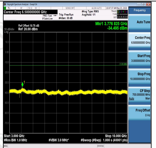
Band26(814-824)-15MHz-16QAM-26765-1RB#0 -3000~10000-PASS
