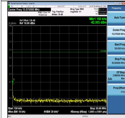
Band26(814-824)-15MHz-QPSK-26765-1RB#74- 0.15~30-PASS
