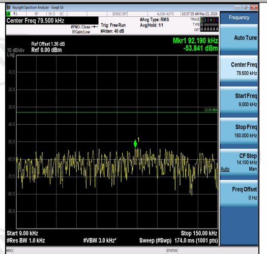
Band26(814-824)-10MHz-16QAM-26740-50RB#4 0-0.009~0.15-PASS
