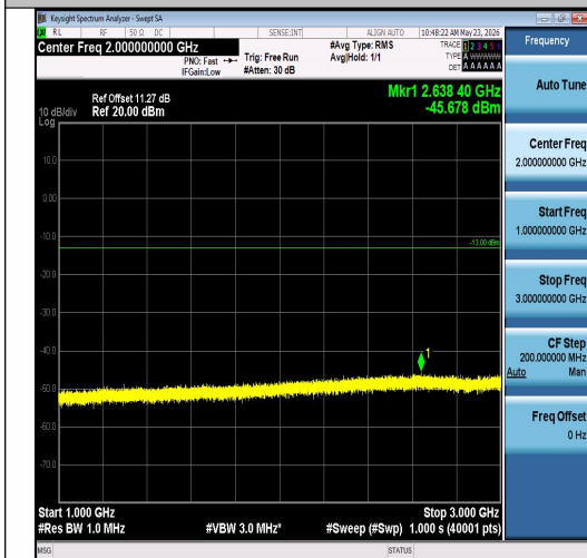
Band26(814-824)-15MHz-QPSK-26765-1RB#74- 1000~3000-PASS
