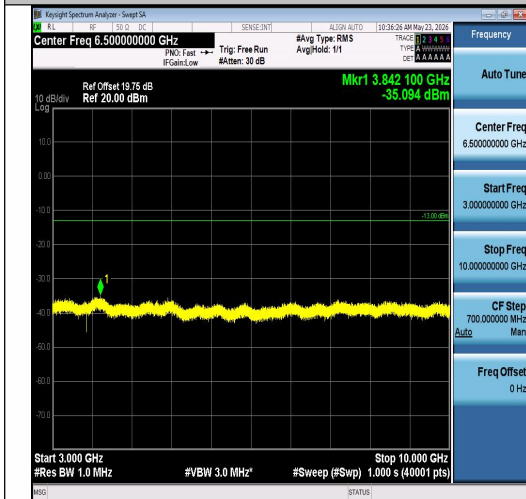
Band26(814-824)-10MHz-16QAM-26740-1RB#4 9-3000~10000-PASS
