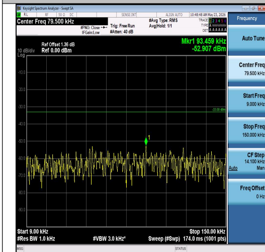
Band26(814-824)-15MHz-16QAM-26765-1RB#7 4-0.009~0.15-PASS
