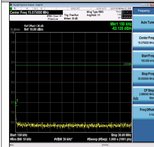
Band26(814-824)-10MHz-16QAM-26740-50RB#4 0-0.15~30-PASS
