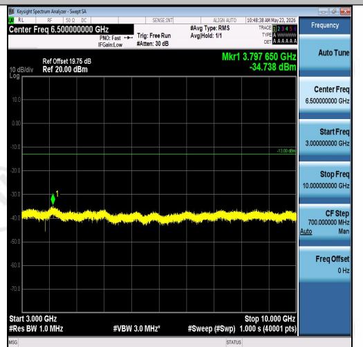
Band26(814-824)-15MHz-QPSK-26765-1RB#74- 3000~10000-PASS
