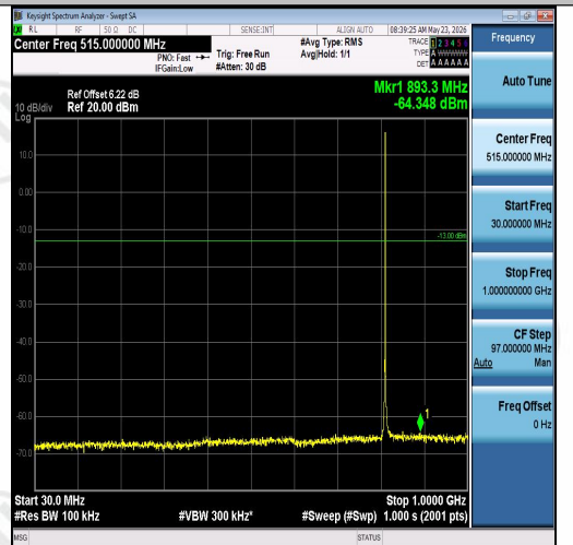
Band26(814-824)-1.4MHz-QPSK-26697-1RB#5-30~1000-PASS
