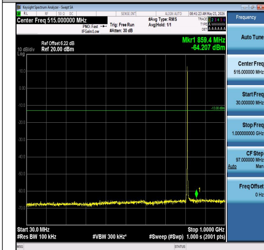
Band26(814-824)-1.4MHz-QPSK-26697-6RB#0-30~1000-PASS
