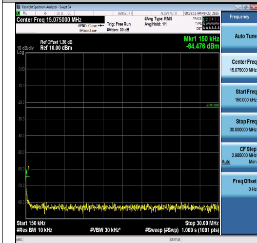
Band26(814-824)-1.4MHz-QPSK-26697-1RB#5-0.15~30-PASS
