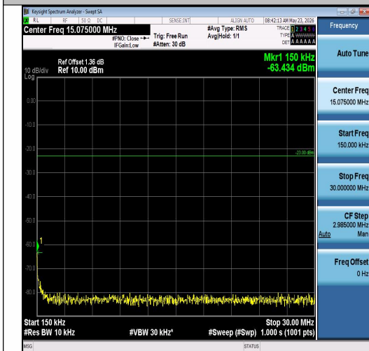
Band26(814-824)-1.4MHz-16QAM-26697-6RB#0 -0.15~30-PASS
