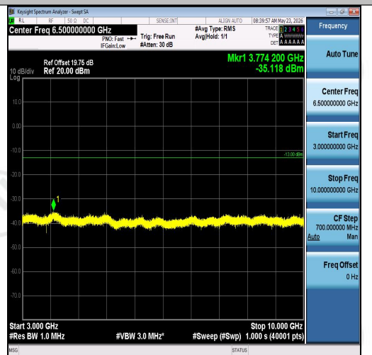
Band26(814-824)-1.4MHz-QPSK-26697-1RB#5-3000~10000-PASS
