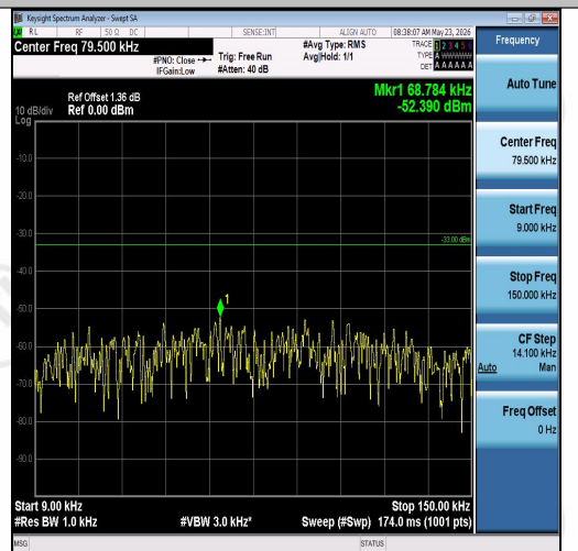
Band26(814-824)-1.4MHz-16QAM-26697-1RB#0-0.009~0.15-PASS
