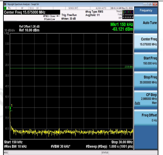
Band26(814-824)-1.4MHz-QPSK-26697-6RB#0-0.15~30-PASS
