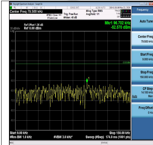
Band26(814-824)-1.4MHz-QPSK-26697-6RB#0-0.009~0.15-PASS
