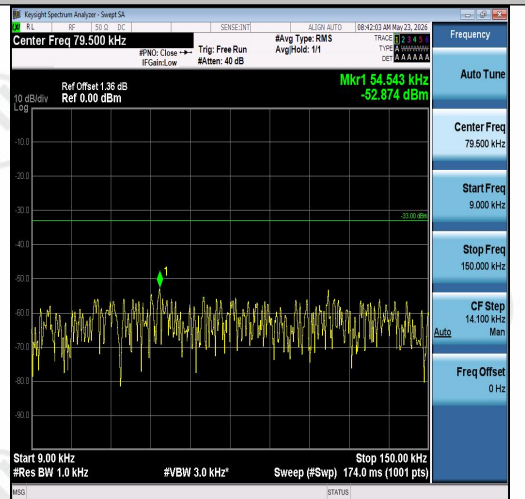
Band26(814-824)-1.4MHz-16QAM-26697-6RB#0 -0.009~0.15-PASS
