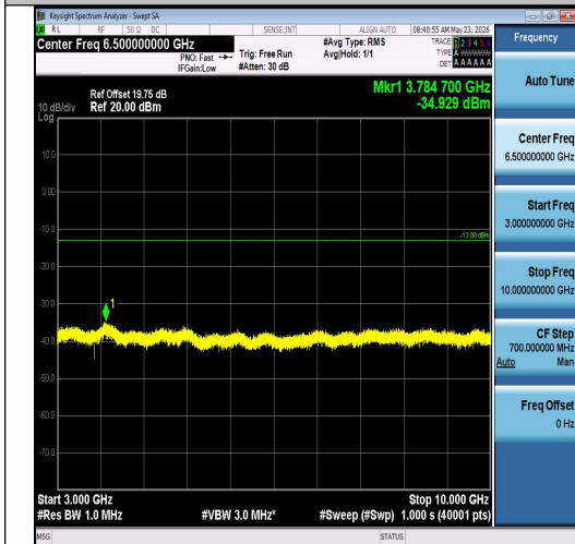
Band26(814-824)-1.4MHz-16QAM-26697-1RB#5 -3000~10000-PASS
