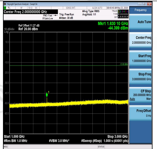
Band26(814-824)-1.4MHz-16QAM-26697-1RB#5 -1000~3000-PASS
