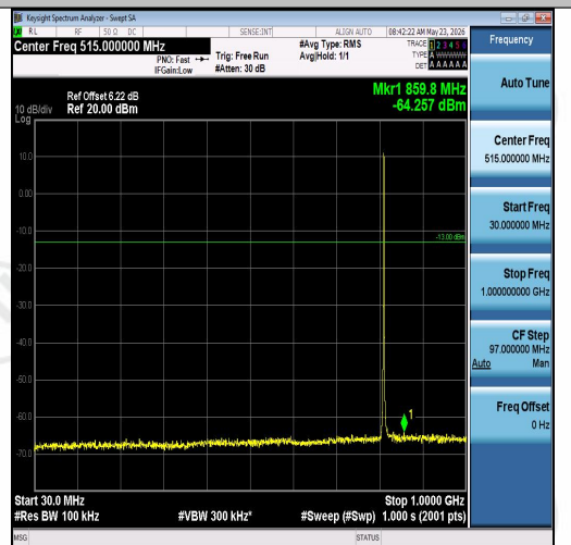
Band26(814-824)-1.4MHz-16QAM-26697-6RB#0 -30~1000-PASS
