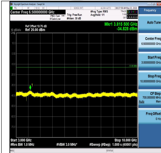
Band26(814-824)-1.4MHz-QPSK-26697-1RB#0-3000~10000-PASS
