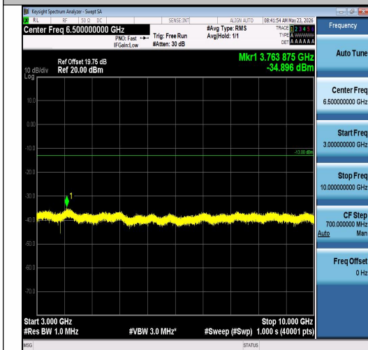
Band26(814-824)-1.4MHz-QPSK-26697-6RB#0-3000~10000-PASS
