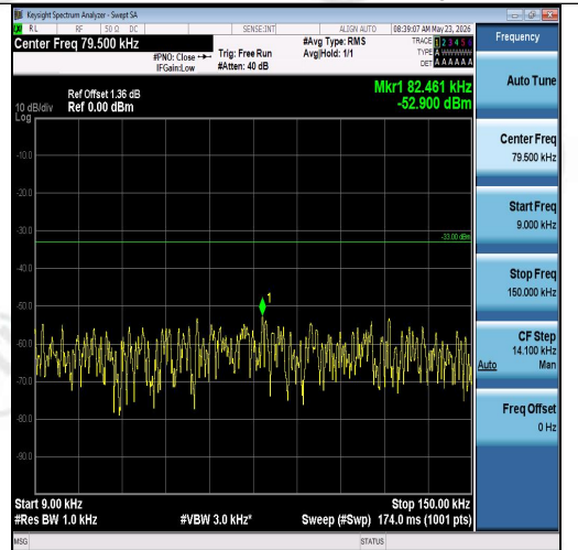
Band26(814-824)-1.4MHz-QPSK-26697-1RB#5-0.009~0.15-PASS
