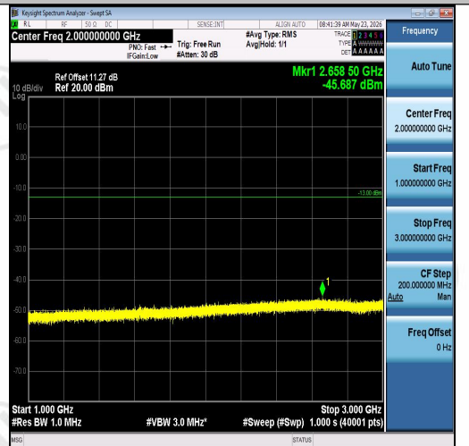
Band26(814-824)-1.4MHz-QPSK-26697-6RB#0-1000~3000-PASS
