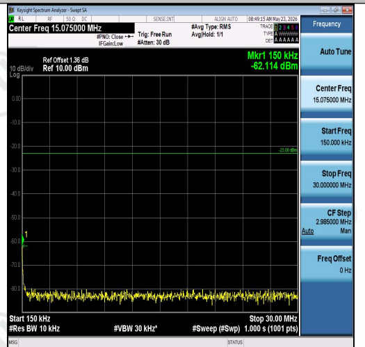
Band26(814-824)-1.4MHz-QPSK-26783-1RB#0- 0.15~30-PASS
