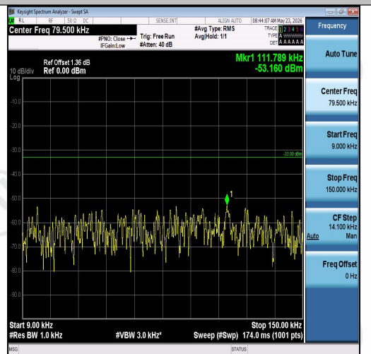
Band26(814-824)-1.4MHz-16QAM-26740-1RB#0-0.009~0.15-PASS
