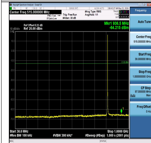
Band26(814-824)-1.4MHz-QPSK-26740-1RB#0- 30~1000-PASS
