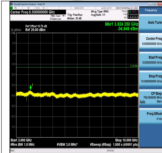
Band26(814-824)-1.4MHz-QPSK-26740-1RB#0-3000~10000-PASS
