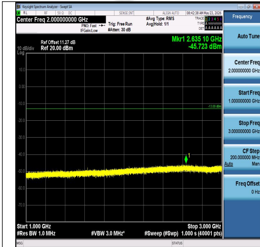
Band26(814-824)-1.4MHz-16QAM-26697-6RB#0 -1000~3000-PASS
