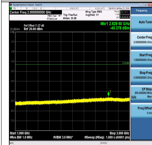
Band26(814-824)-1.4MHz-QPSK-26740-1RB#5-1000~3000-PASS
