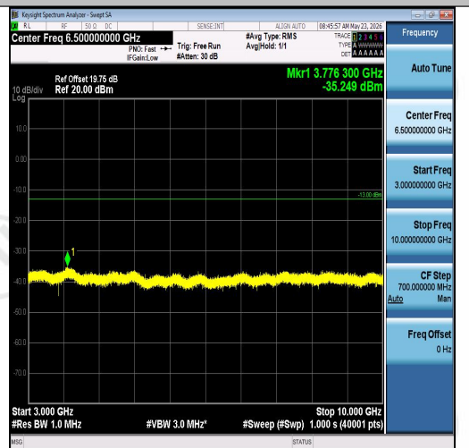
Band26(814-824)-1.4MHz-QPSK-26740-1RB#5-3000~10000-PASS
