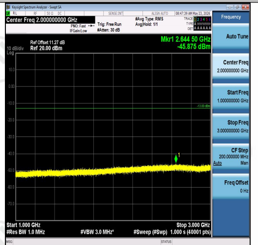
Band26(814-824)-1.4MHz-QPSK-26740-6RB#0-1000~3000-PASS
