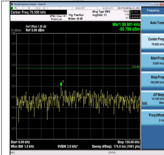
Band26(814-824)-1.4MHz-QPSK-26740-6RB#0-0.009~0.15-PASS
