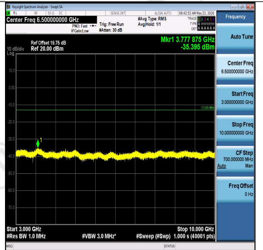
Band26(814-824)-1.4MHz-16QAM-26697-6RB#0 -3000~10000-PASS
