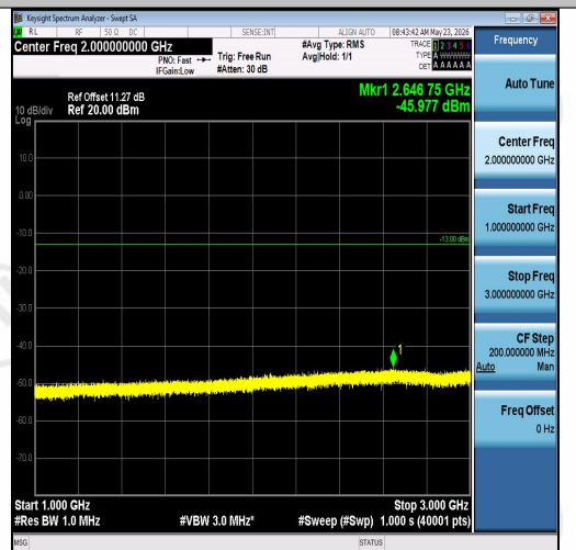
Band26(814-824)-1.4MHz-QPSK-26740-1RB#0- 1000~3000-PASS
