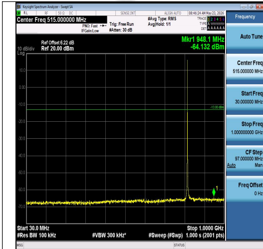
Band26(814-824)-1.4MHz-16QAM-26740-1RB#5 -30~1000-PASS
