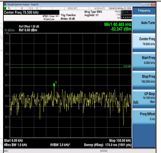
Band26(814-824)-1.4MHz-16QAM-26740-6RB#0 -0.009~0.15-PASS
