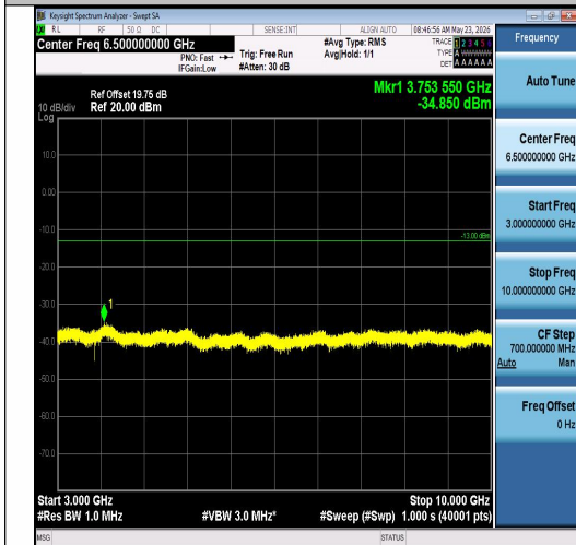
Band26(814-824)-1.4MHz-16QAM-26740-1RB#5 -3000~10000-PASS
