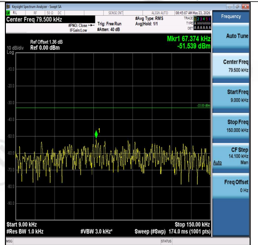
Band26(814-824)-1.4MHz-QPSK-26740-1RB#5-0.009~0.15-PASS
