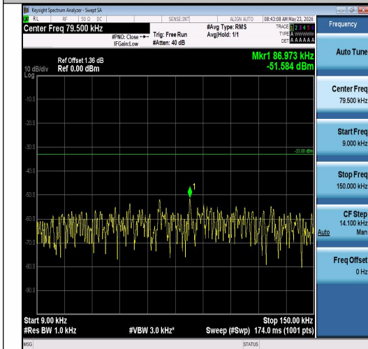
Band26(814-824)-1.4MHz-QPSK-26740-1RB#0- 0.009~0.15-PASS
