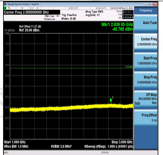
Band26(814-824)-1.4MHz-16QAM-26740-1RB#5 -1000~3000-PASS
