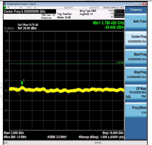
Band26(814-824)-1.4MHz-16QAM-26740-6RB#0 -3000~10000-PASS
