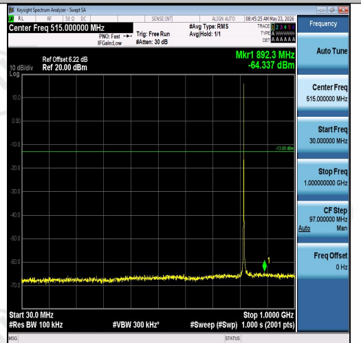
Band26(814-824)-1.4MHz-QPSK-26740-1RB#5-30~1000-PASS
