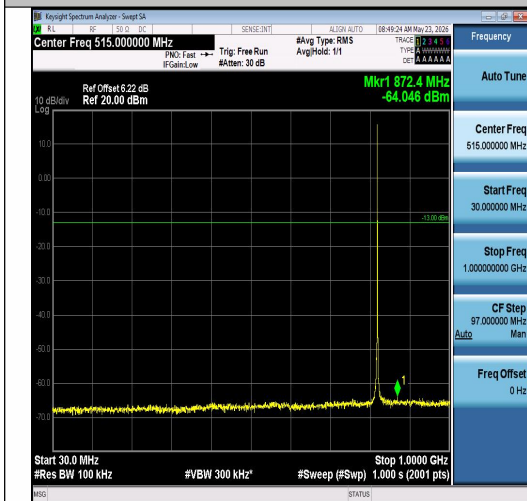
Band26(814-824)-1.4MHz-QPSK-26783-1RB#0- 30~1000-PASS
