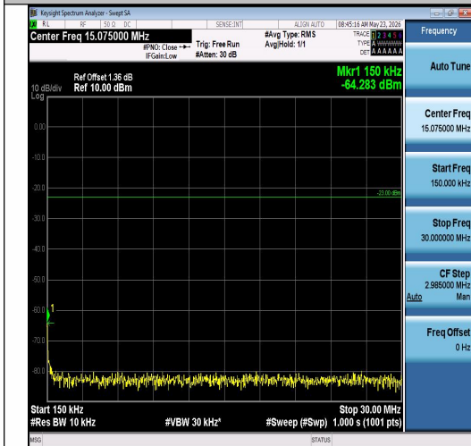
Band26(814-824)-1.4MHz-QPSK-26740-1RB#5-0.15~30-PASS
