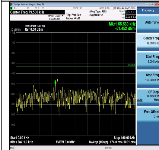
Band26(814-824)-1.4MHz-QPSK-26783-1RB#0- 0.009~0.15-PASS
