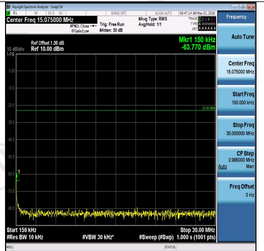
Band26(814-824)-1.4MHz-QPSK-26740-6RB#0-0.15~30-PASS
