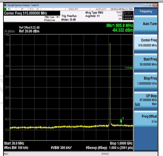
Band26(814-824)-1.4MHz-16QAM-26740-6RB#0 -30~1000-PASS
