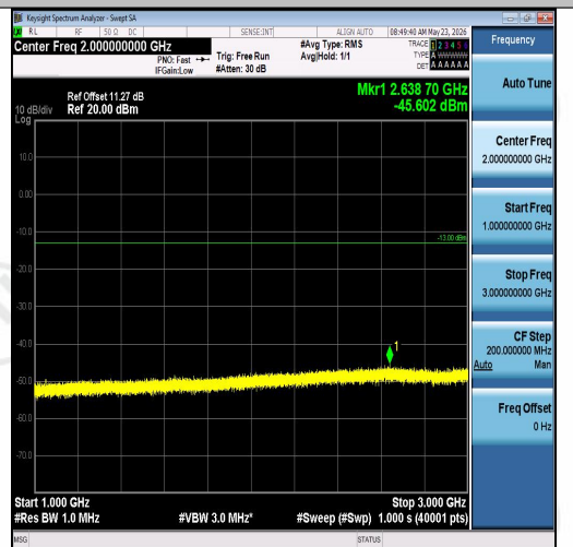
Band26(814-824)-1.4MHz-QPSK-26783-1RB#0- 1000~3000-PASS
