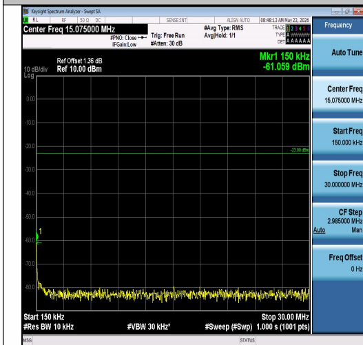
Band26(814-824)-1.4MHz-16QAM-26740-6RB#0 -0.15~30-PASS
