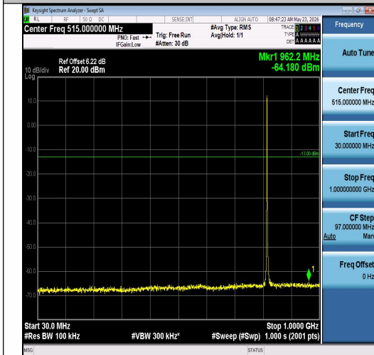
Band26(814-824)-1.4MHz-QPSK-26740-6RB#0-30~1000-PASS
