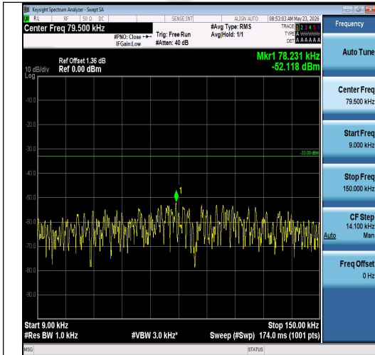
Band26(814-824)-1.4MHz-QPSK-26783-6RB#0-0.009~0.15-PASS
