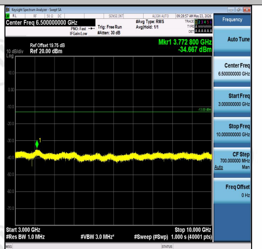
Band26(814-824)-3MHz-16QAM-26705-1RB#0-3000~10000-PASS
