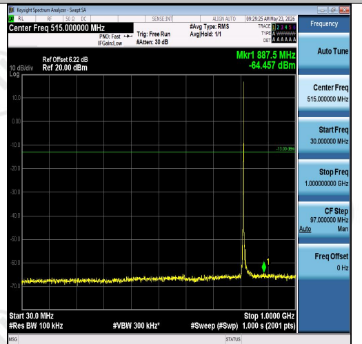
Band26(814-824)-3MHz-QPSK-26705-1RB#14-3 0~1000-PASS
