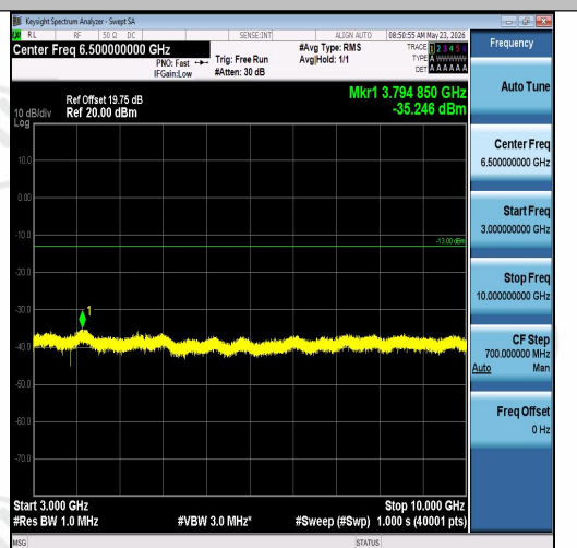
Band26(814-824)-1.4MHz-16QAM-26783-1RB#0 -3000~10000-PASS
