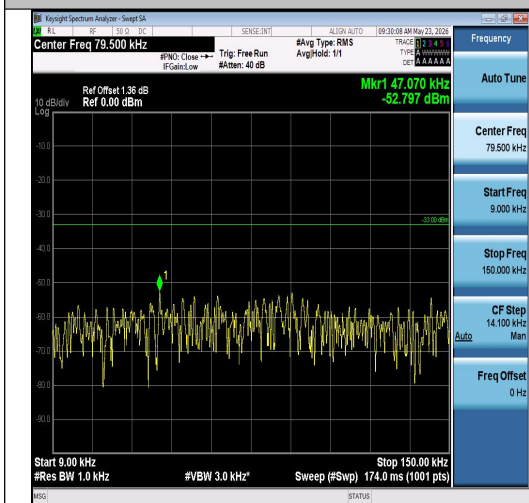
Band26(814-824)-3MHz-16QAM-26705-1RB#14-0.009~0.15-PASS
