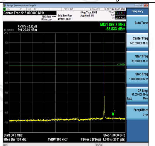
Band26(814-824)-1.4MHz-16QAM-26783-1RB#0 -30~1000-PASS
