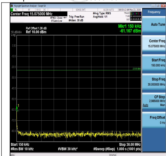
Band26(814-824)-1.4MHz-16QAM-26783-1RB#0 -0.15~30-PASS
