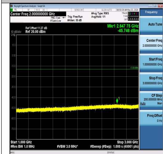
Band26(814-824)-1.4MHz-16QAM-26783-1RB#0 -1000~3000-PASS
