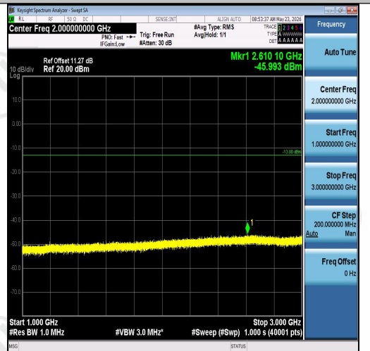
Band26(814-824)-1.4MHz-QPSK-26783-6RB#0-1000~3000-PASS
