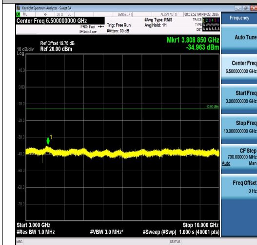
Band26(814-824)-1.4MHz-QPSK-26783-6RB#0-3000~10000-PASS
