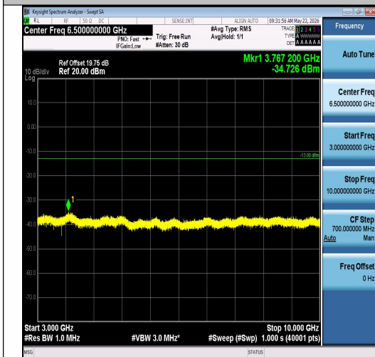
Band26(814-824)-3MHz-QPSK-26705-15RB#0-3 000~10000-PASS
