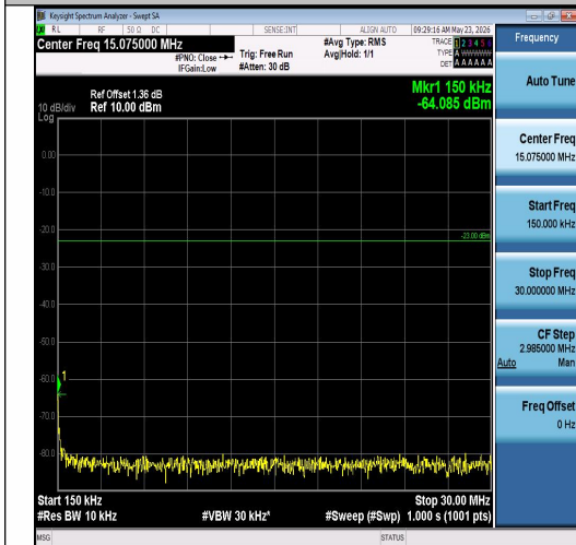
Band26(814-824)-3MHz-QPSK-26705-1RB#14-0 .15~30-PASS
