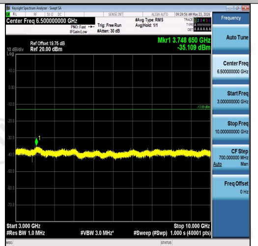
Band26(814-824)-3MHz-QPSK-26705-1RB#14-3 000~10000-PASS
