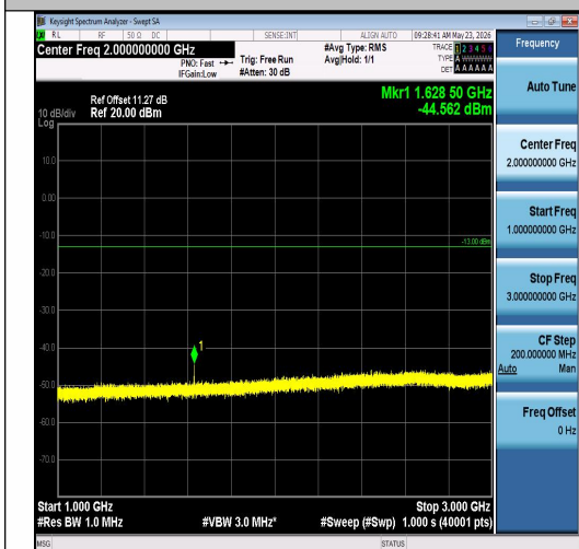
Band26(814-824)-3MHz-16QAM-26705-1RB#0-1000~3000-PASS
