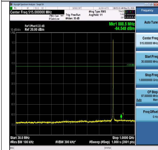
Band26(814-824)-1.4MHz-QPSK-26783-6RB#0-30~1000-PASS
