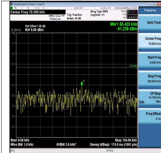
Band26(814-824)-3MHz-QPSK-26705-15RB#0-0 .009~0.15-PASS
