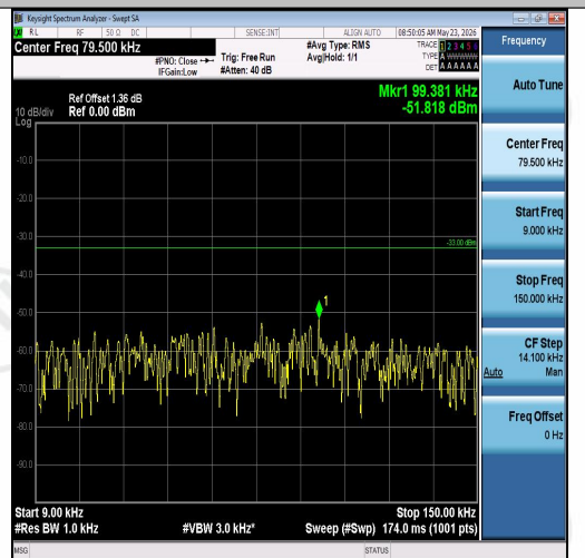
Band26(814-824)-1.4MHz-16QAM-26783-1RB#0-0.009~0.15-PASS
