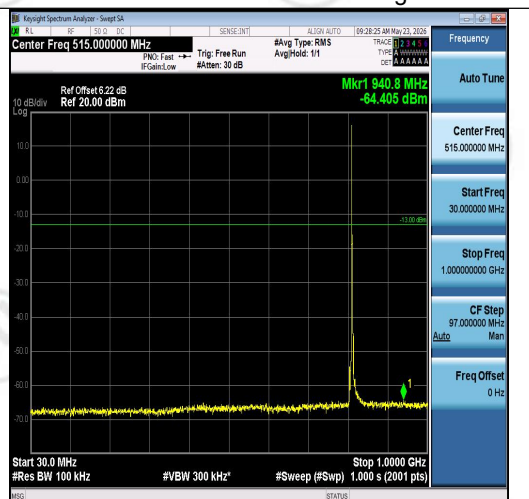
Band26(814-824)-3MHz-16QAM-26705-1RB#0-30~1000-PASS
