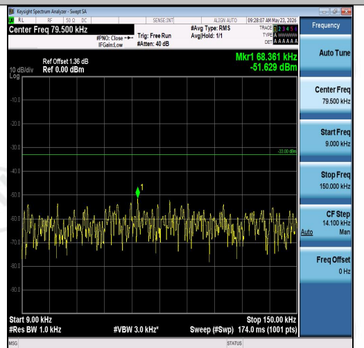
Band26(814-824)-3MHz-16QAM-26705-1RB#0- 0.009~0.15-PASS
