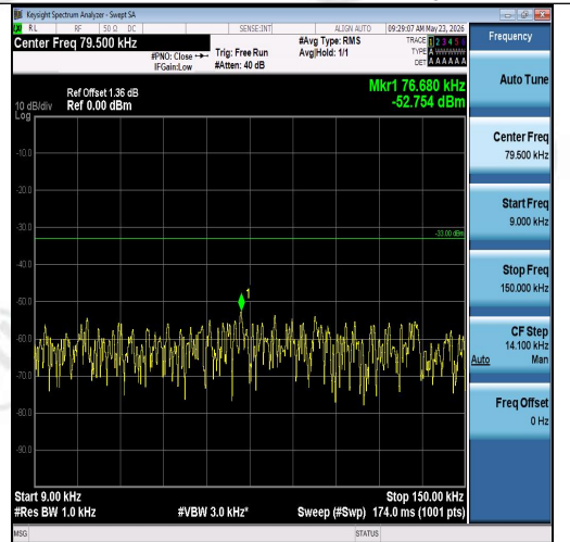
Band26(814-824)-3MHz-QPSK-26705-1RB#14-0 .009~0.15-PASS
