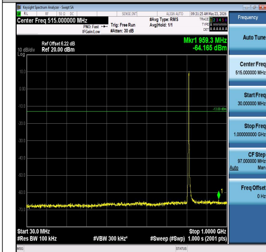
Band26(814-824)-3MHz-QPSK-26705-15RB#0-3 0~1000-PASS
