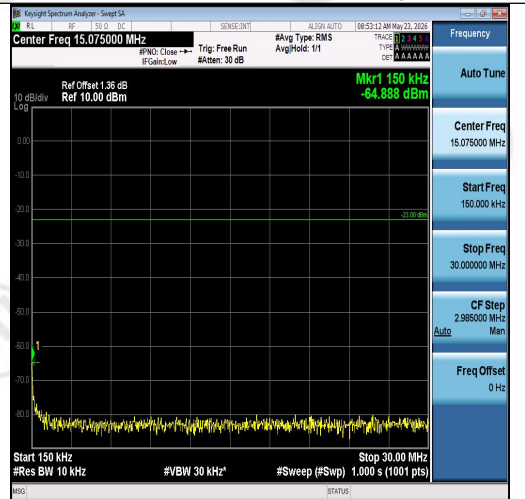
Band26(814-824)-1.4MHz-QPSK-26783-6RB#0-0.15~30-PASS
