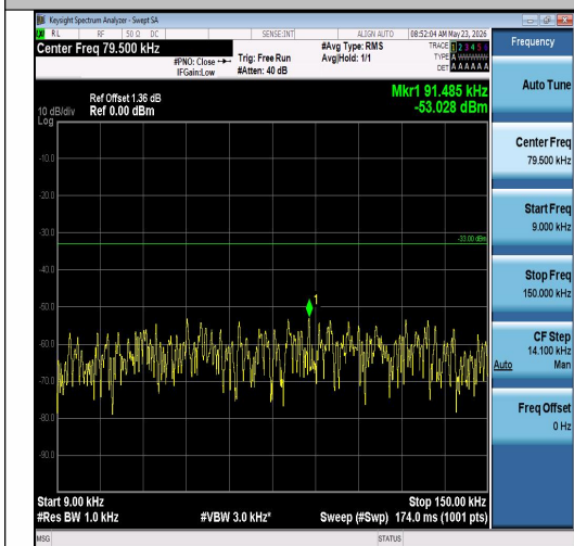
Band26(814-824)-1.4MHz-16QAM-26783-1RB#5 -0.009~0.15-PASS
