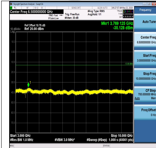
Band26(814-824)-3MHz-QPSK-26705-1RB#0-30 00~10000-PASS
