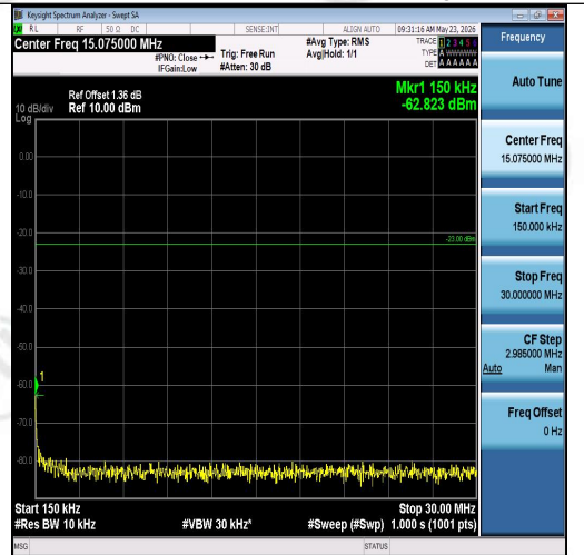
Band26(814-824)-3MHz-QPSK-26705-15RB#0-0 .15~30-PASS
