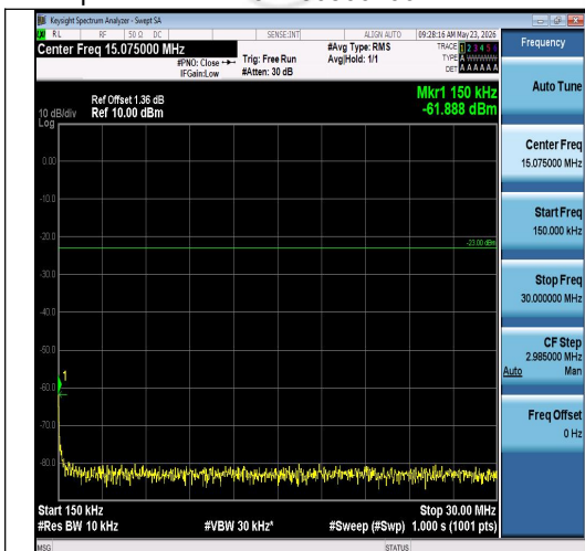
Band26(814-824)-3MHz-16QAM-26705-1RB#0-0.15~30-PASS
