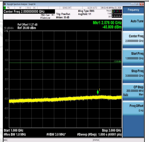
Band26(814-824)-3MHz-QPSK-26705-15RB#0-1 000~3000-PASS
