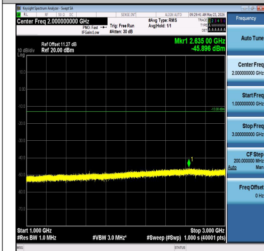
Band26(814-824)-3MHz-QPSK-26705-1RB#14-1 000~3000-PASS
