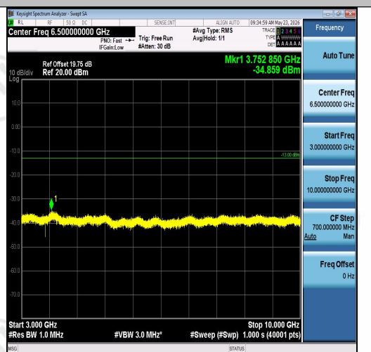
Band26(814-824)-3MHz-16QAM-26740-1RB#0-3000~10000-PASS
