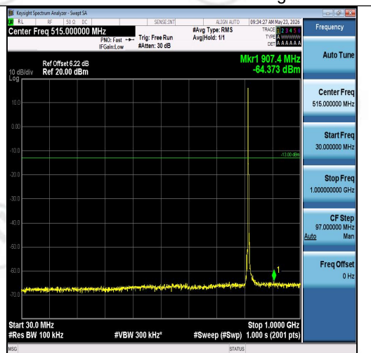
Band26(814-824)-3MHz-16QAM-26740-1RB#0-30~1000-PASS
