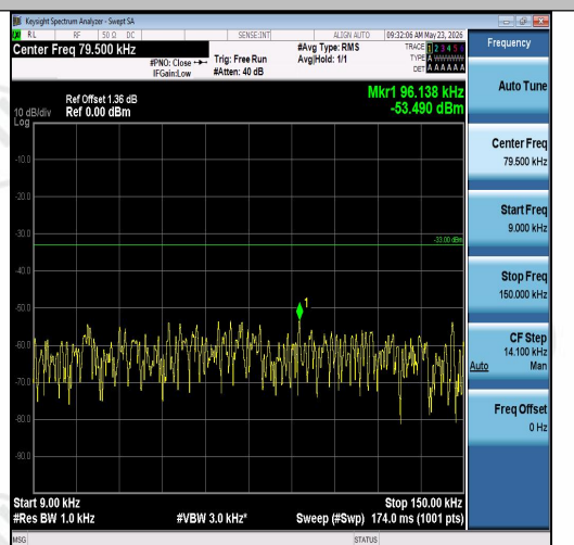
Band26(814-824)-3MHz-16QAM-26705-15RB#0 -0.009~0.15-PASS
