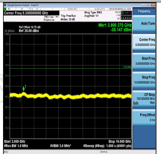
Band26(814-824)-3MHz-QPSK-26740-1RB#14-3 000~10000-PASS
