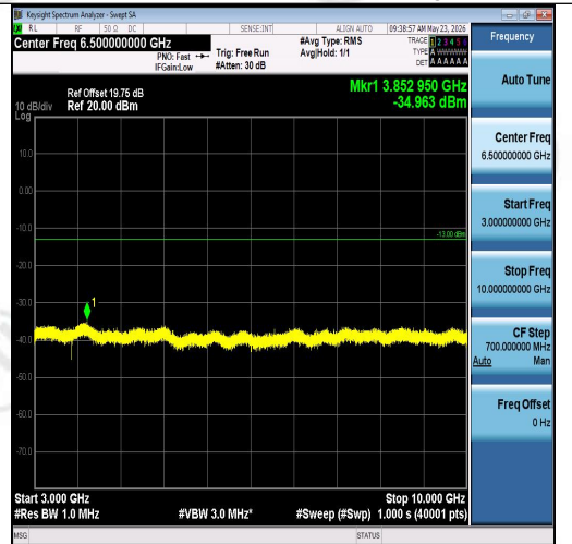
Band26(814-824)-3MHz-16QAM-26740-15RB#0 -3000~10000-PASS
