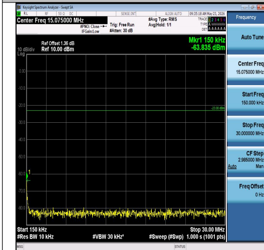
Band26(814-824)-3MHz-QPSK-26740-1RB#14-0 .15~30-PASS
