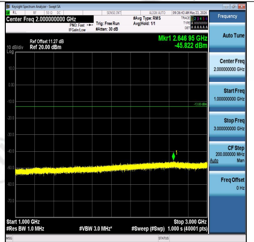
Band26(814-824)-3MHz-16QAM-26740-1RB#14 -1000~3000-PASS
