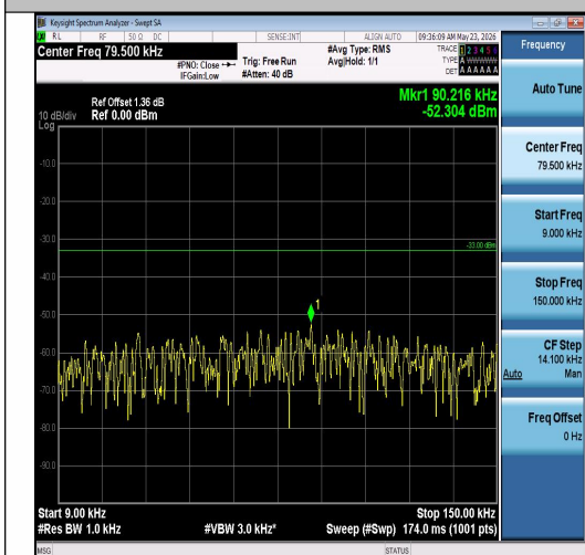
Band26(814-824)-3MHz-16QAM-26740-1RB#14-0.009~0.15-PASS
