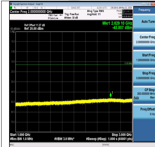
Band26(814-824)-3MHz-16QAM-26740-15RB#0 -1000~3000-PASS
