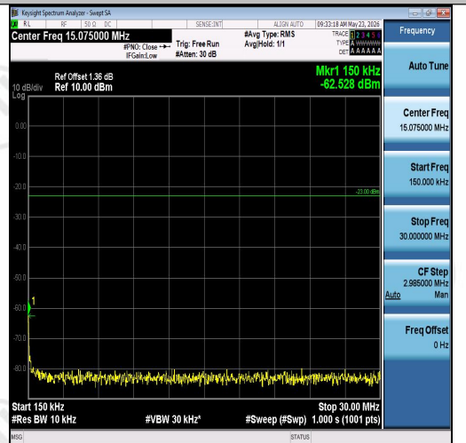
Band26(814-824)-3MHz-QPSK-26740-1RB#0-0. 15~30-PASS
