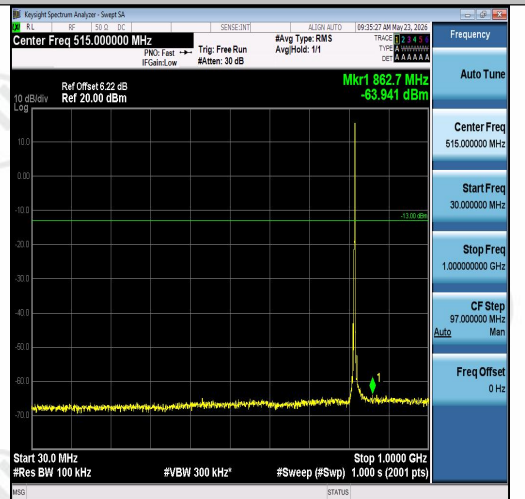
Band26(814-824)-3MHz-QPSK-26740-1RB#14-3 0~1000-PASS
