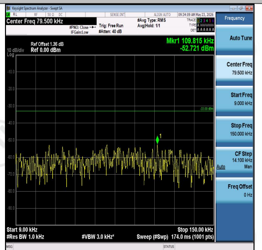
Band26(814-824)-3MHz-16QAM-26740-1RB#0-0 0.009~0.15-PASS
