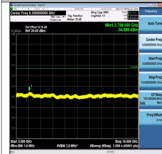
Band26(814-824)-3MHz-QPSK-26740-15RB#0-3 000~10000-PASS
