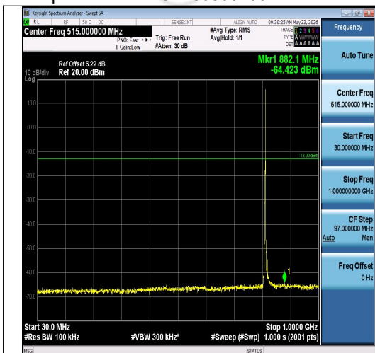
Band26(814-824)-3MHz-16QAM-26705-1RB#14 -30~1000-PASS
