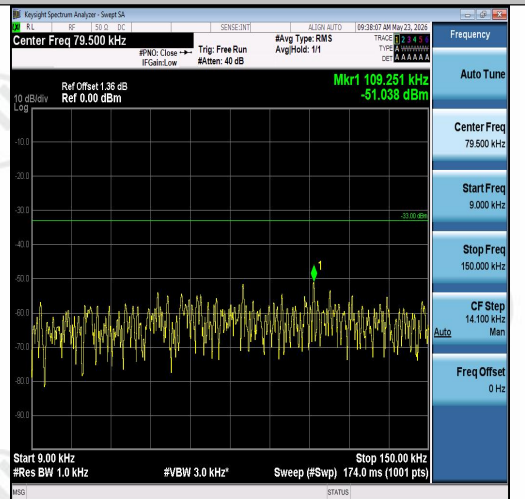
Band26(814-824)-3MHz-16QAM-26740-15RB#0 -0.009~0.15-PASS
