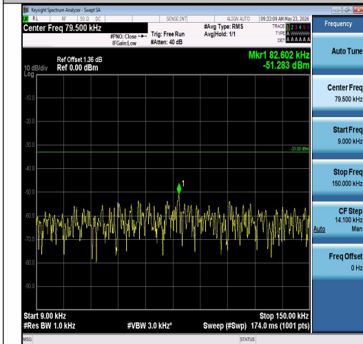
Band26(814-824)-3MHz-QPSK-26740-1RB#0-0. 009~0.15-PASS
