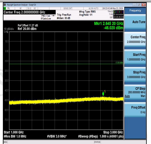
Band26(814-824)-3MHz-QPSK-26740-1RB#0-10 00~3000-PASS
