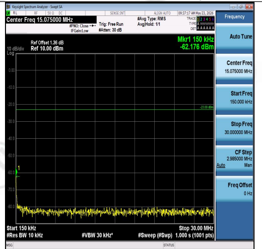
Band26(814-824)-3MHz-QPSK-26740-15RB#0-0 .15~30-PASS
