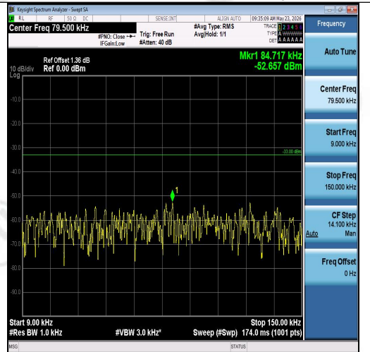
Band26(814-824)-3MHz-QPSK-26740-1RB#14-0 .009~0.15-PASS
