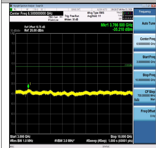
Band26(814-824)-3MHz-16QAM-26705-1RB#14 -3000~10000-PASS
