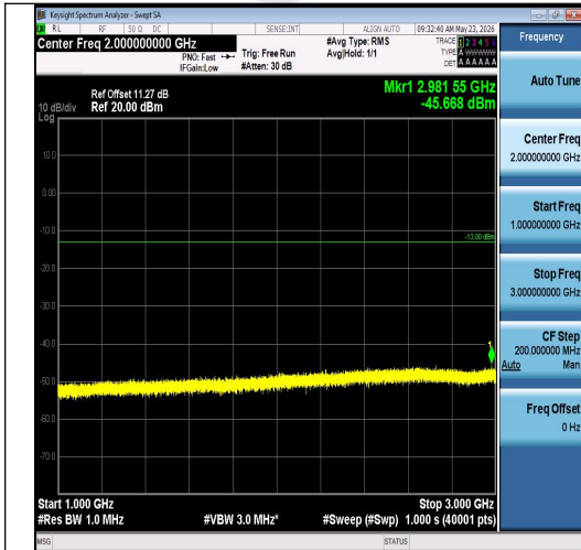
Band26(814-824)-3MHz-16QAM-26705-15RB#0 -1000~3000-PASS
