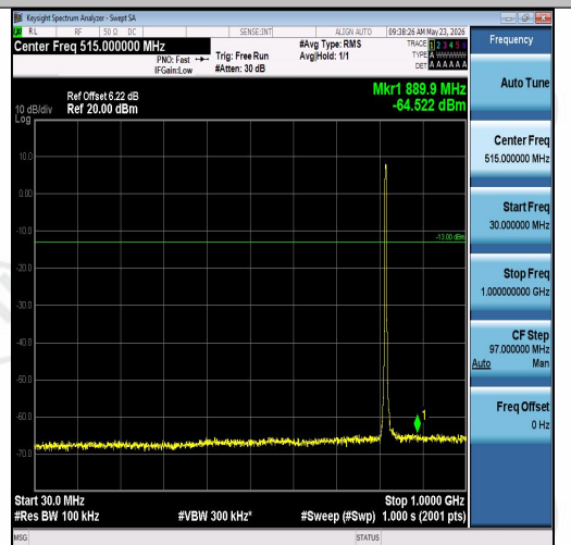
Band26(814-824)-3MHz-16QAM-26740-15RB#0 -30~1000-PASS
