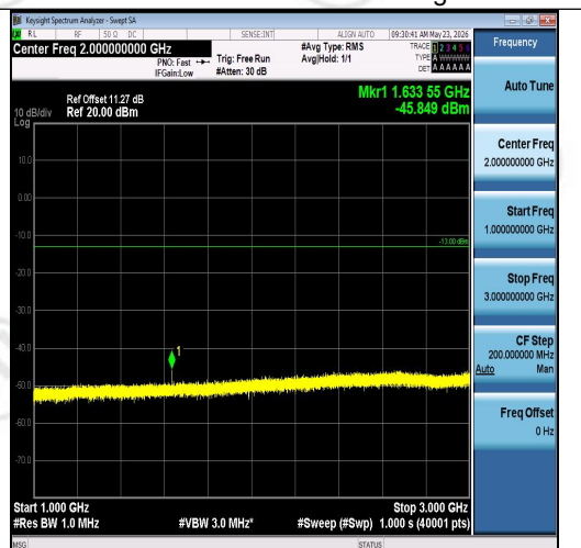
Band26(814-824)-3MHz-16QAM-26705-1RB#14 -1000~3000-PASS
