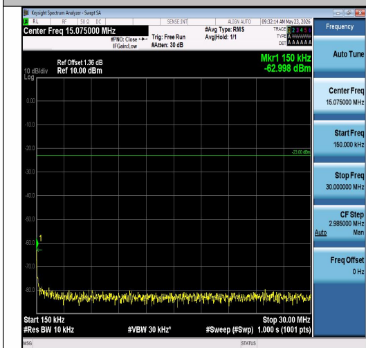
Band26(814-824)-3MHz-16QAM-26705-15RB#0 -0.15~30-PASS
