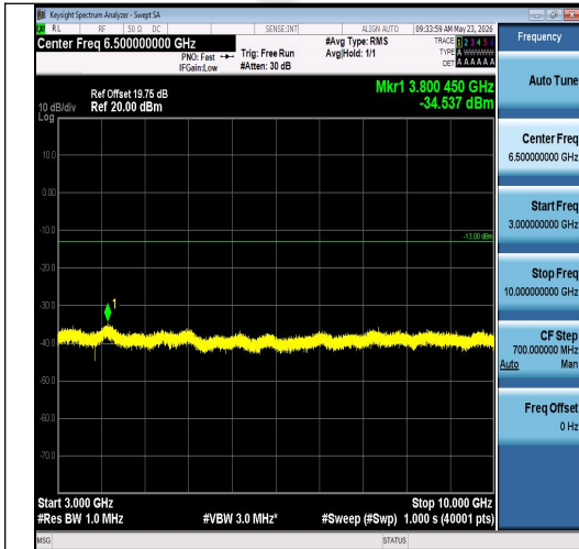
Band26(814-824)-3MHz-QPSK-26740-1RB#0-30 00~10000-PASS
