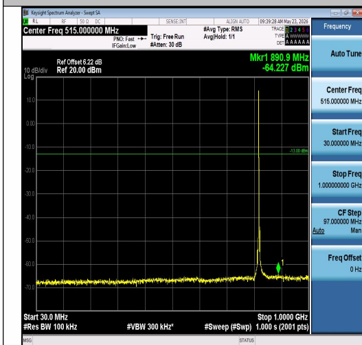
Band26(814-824)-3MHz-QPSK-26775-1RB#0-30 ~1000-PASS
