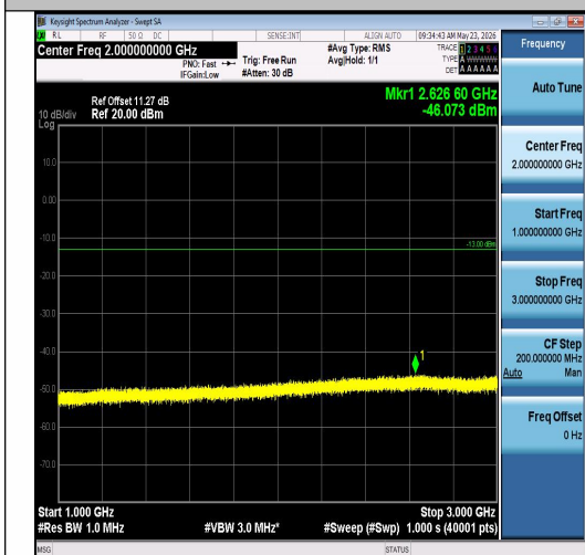
Band26(814-824)-3MHz-16QAM-26740-1RB#0-1000~3000-PASS
