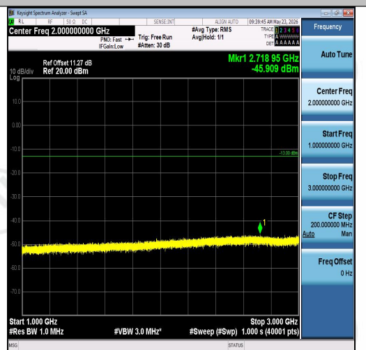
Band26(814-824)-3MHz-QPSK-26775-1RB#0-10 00~3000-PASS
