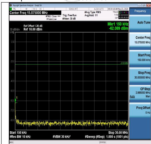
Band26(814-824)-3MHz-16QAM-26740-1RB#0-0.15~30-PASS
