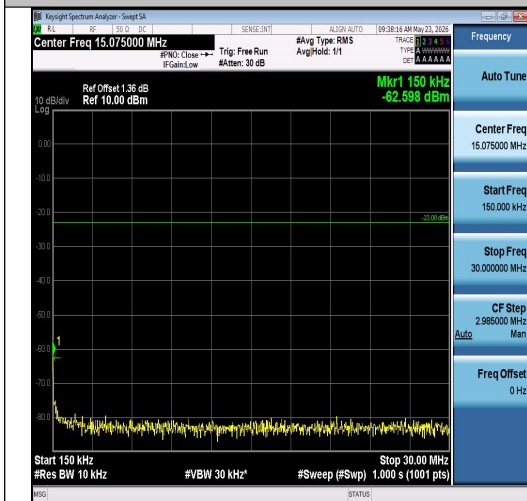
Band26(814-824)-3MHz-16QAM-26740-15RB#0 -0.15~30-PASS
