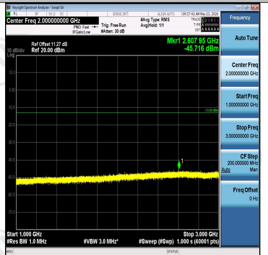
Band26(814-824)-3MHz-QPSK-26740-15RB#0-1 000~3000-PASS
