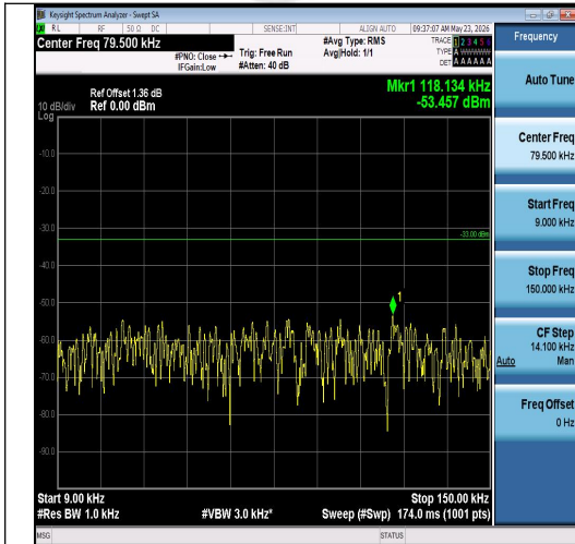
Band26(814-824)-3MHz-QPSK-26740-15RB#0-0 .009~0.15-PASS
