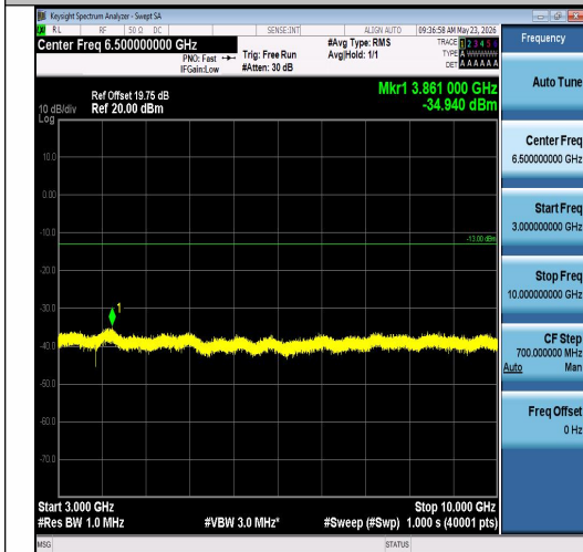
Band26(814-824)-3MHz-16QAM-26740-1RB#14 -3000~10000-PASS
