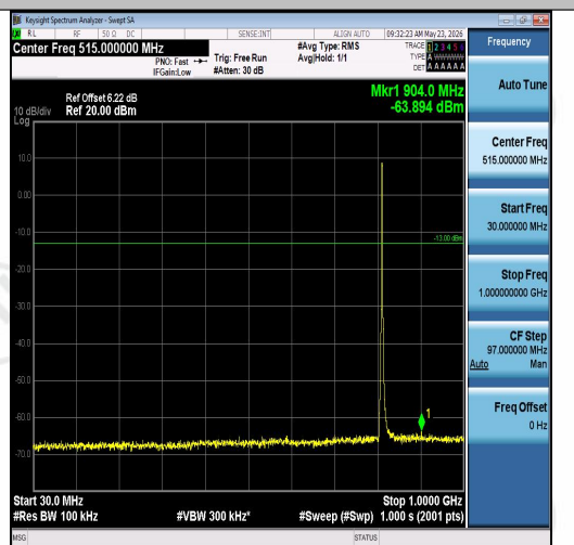
Band26(814-824)-3MHz-16QAM-26705-15RB#0 -30~1000-PASS
