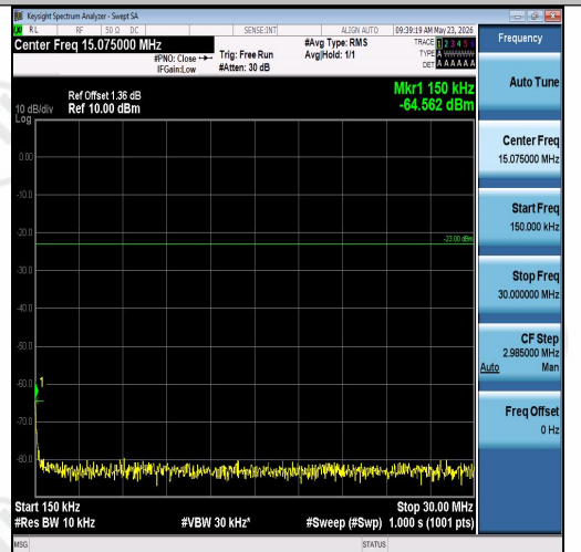
Band26(814-824)-3MHz-QPSK-26775-1RB#0-0. 15~30-PASS
