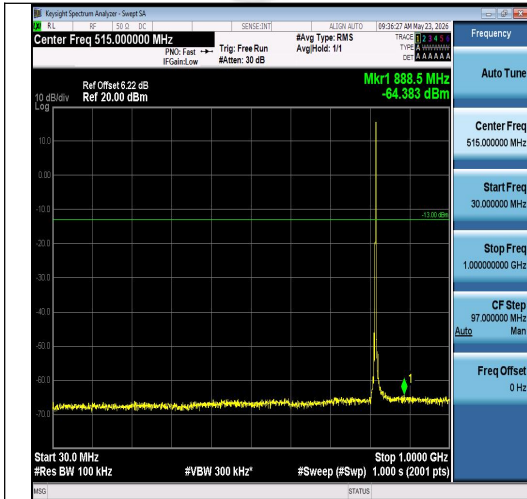
Band26(814-824)-3MHz-16QAM-26740-1RB#14 -30~1000-PASS
