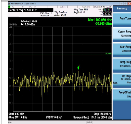
Band26(814-824)-3MHz-QPSK-26775-1RB#0-0. 009~0.15-PASS
