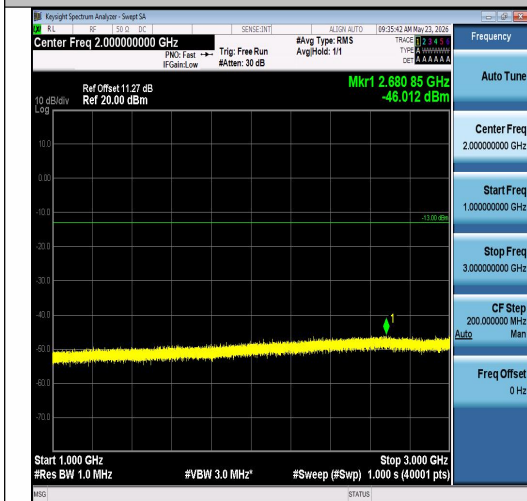
Band26(814-824)-3MHz-QPSK-26740-1RB#14-1 000~3000-PASS
