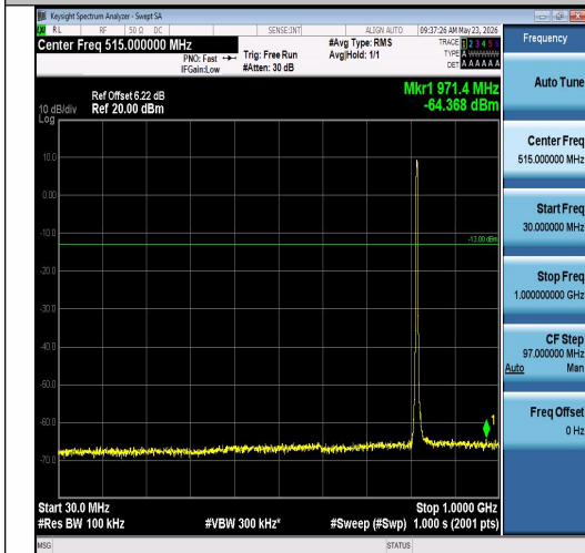
Band26(814-824)-3MHz-QPSK-26740-15RB#0-3 0~1000-PASS
