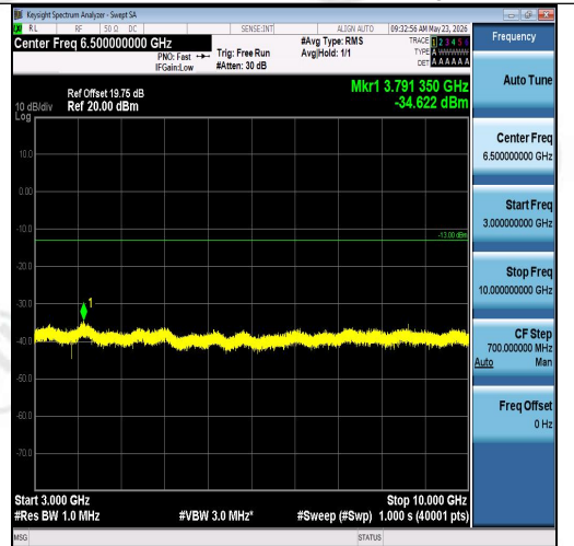
Band26(814-824)-3MHz-16QAM-26705-15RB#0 -3000~10000-PASS
