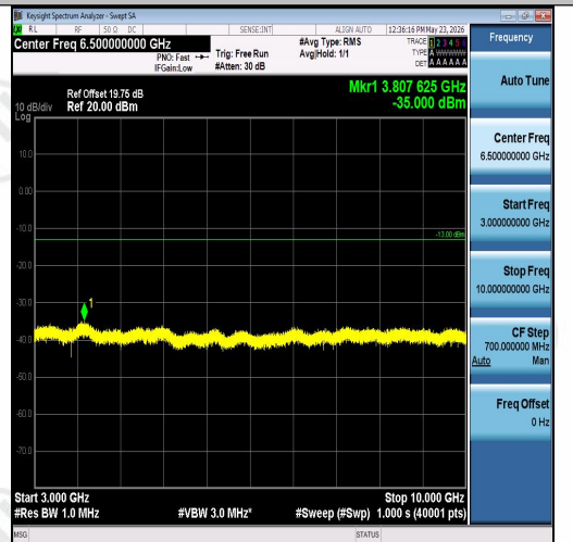
Band26(824-849)-5MHz-16QAM-26815-1RB#0-3000~10000-PASS
