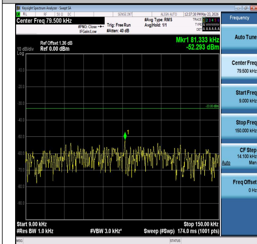
Band26(824-849)-5MHz-16QAM-26815-1RB#24-0.009~0.15-PASS
