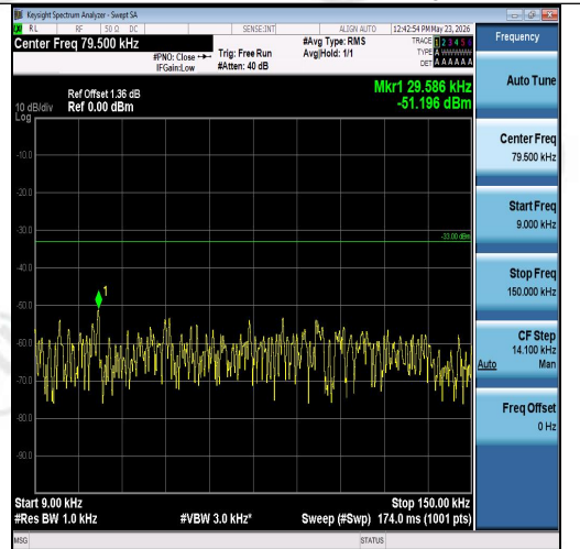
Band26(824-849)-5MHz-QPSK-26915-1RB#24-0 .009~0.15-PASS
