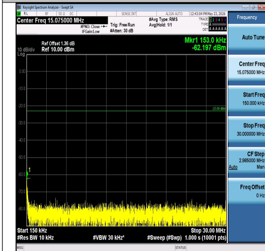
Band26(824-849)-5MHz-QPSK-26915-1RB#24-0 .15~30-PASS
