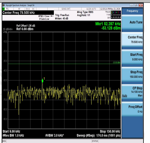
Band26(824-849)-5MHz-16QAM-26815-1RB#0-0 0.009~0.15-PASS
