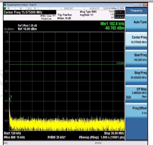
Band26(824-849)-5MHz-16QAM-26815-1RB#24-0.15~30-PASS
