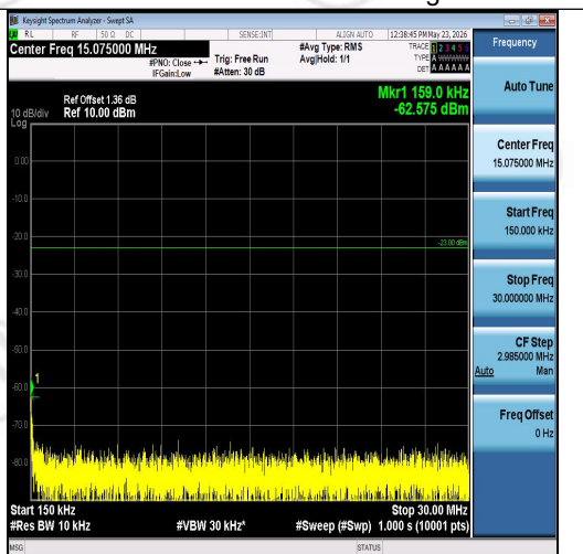
Band26(824-849)-5MHz-QPSK-26815-25RB#0-0 .15~30-PASS
