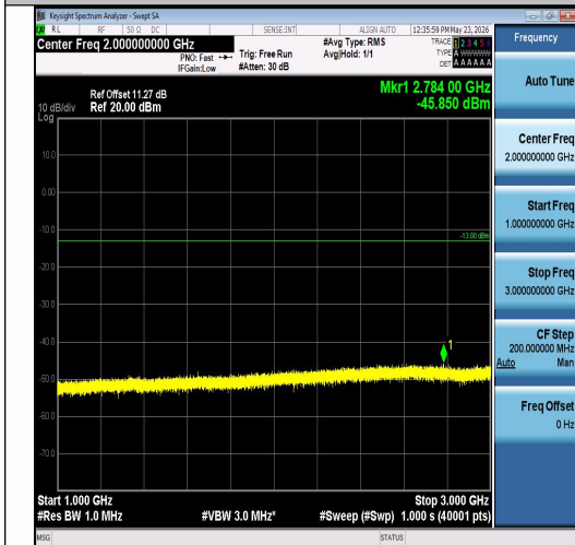
Band26(824-849)-5MHz-16QAM-26815-1RB#0-1000~3000-PASS
