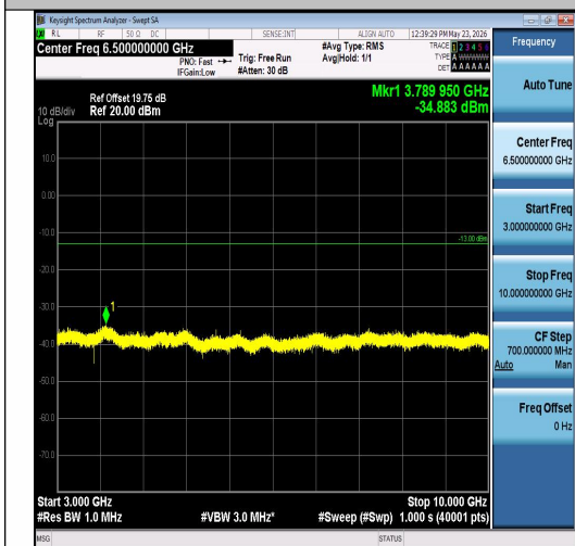
Band26(824-849)-5MHz-QPSK-26815-25RB#0-3 000~10000-PASS
