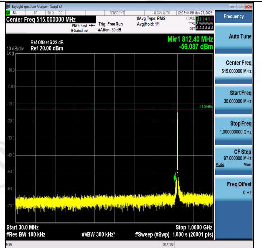
Band26(824-849)-5MHz-16QAM-26815-1RB#0-30~1000-PASS
