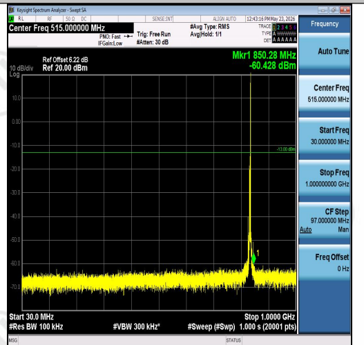
Band26(824-849)-5MHz-QPSK-26915-1RB#24-3 0~1000-PASS
