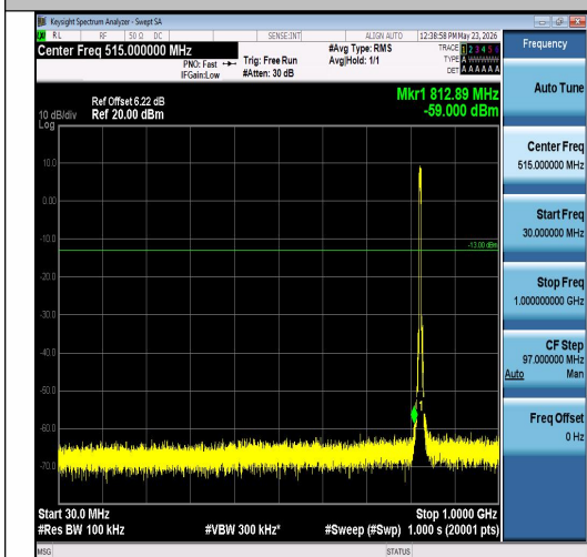
Band26(824-849)-5MHz-QPSK-26815-25RB#0-3 0~1000-PASS
