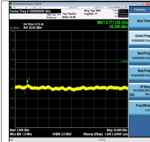
Band26(824-849)-5MHz-QPSK-26915-1RB#0-30 00~10000-PASS
