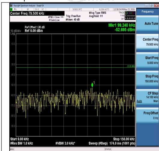
Band26(824-849)-5MHz-QPSK-26815-25RB#0-0 .009~0.15-PASS
