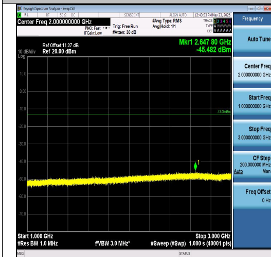
Band26(824-849)-5MHz-QPSK-26915-1RB#24-1 000~3000-PASS
