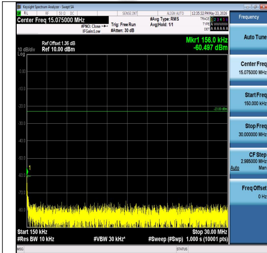
Band26(824-849)-5MHz-16QAM-26815-1RB#0-0.15~30-PASS
