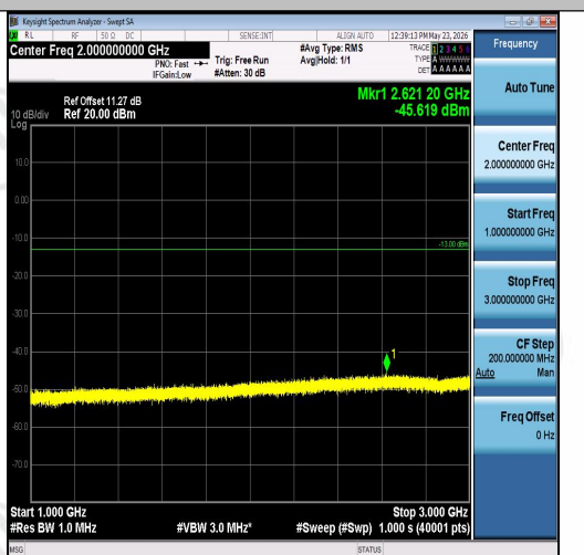
Band26(824-849)-5MHz-QPSK-26815-25RB#0-1 000~3000-PASS
