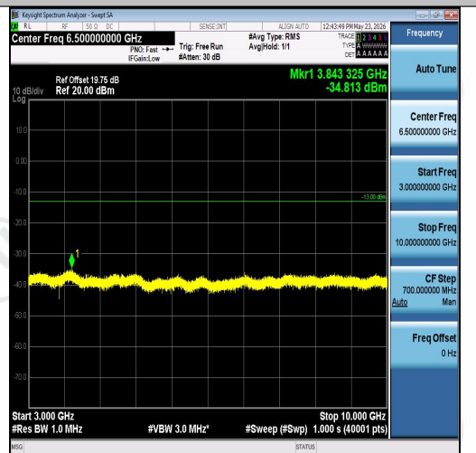
Band26(824-849)-5MHz-QPSK-26915-1RB#24-3 000~10000-PASS
