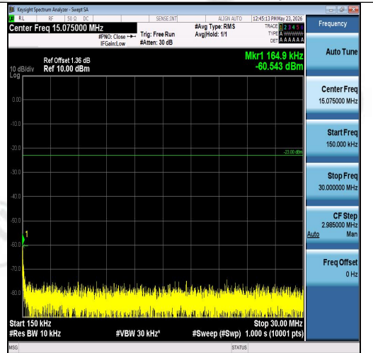
Band26(824-849)-5MHz-QPSK-26915-25RB#0-0 .15~30-PASS
