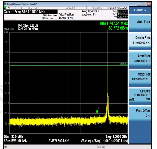
Band26(824-849)-5MHz-16QAM-26915-1RB#0-30~1000-PASS
