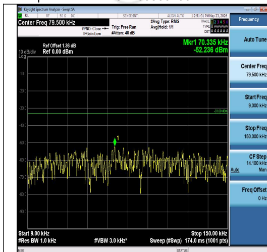
Band26(824-849)-5MHz-QPSK-27015-25RB#0-0 .009~0.15-PASS
