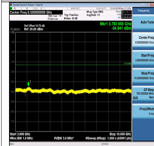
Band26(824-849)-5MHz-QPSK-26915-25RB#0-3 000~10000-PASS
