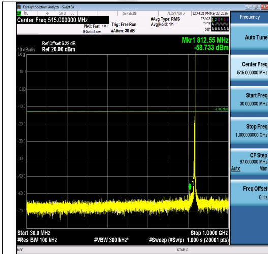
Band26(824-849)-5MHz-16QAM-26915-1RB#24 -30~1000-PASS
