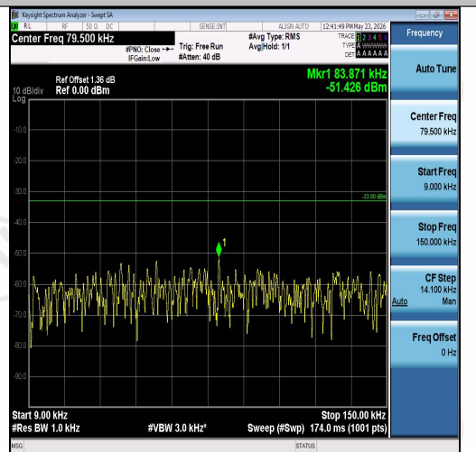
Band26(824-849)-5MHz-16QAM-26915-1RB#0-0 0.009~0.15-PASS
