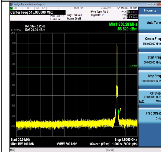
Band26(824-849)-5MHz-QPSK-26915-25RB#0-3 0~1000-PASS
