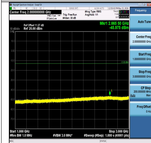
Band26(824-849)-5MHz-QPSK-27015-1RB#24-1 000~3000-PASS
