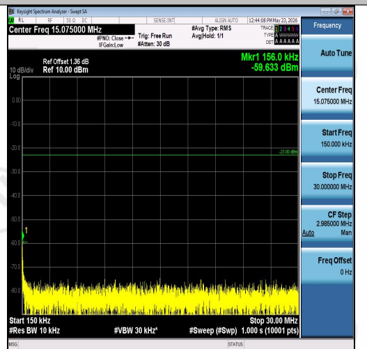
Band26(824-849)-5MHz-16QAM-26915-1RB#24-0.15~30-PASS
