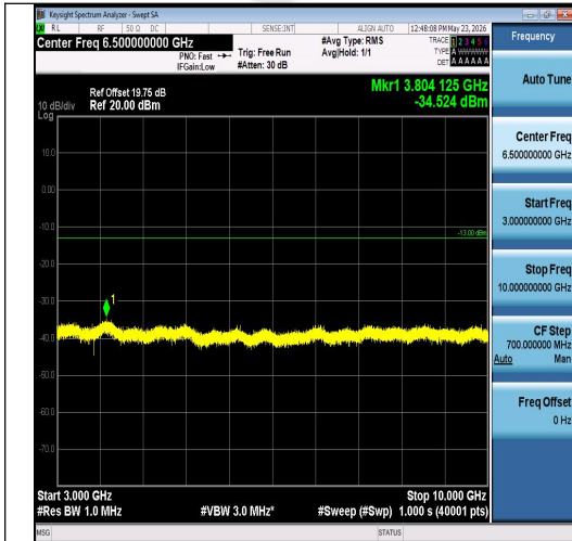
Band26(824-849)-5MHz-QPSK-27015-1RB#0-30 00~10000-PASS
