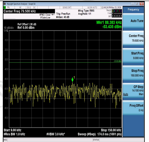
Band26(824-849)-5MHz-QPSK-27015-1RB#24-0 .009~0.15-PASS
