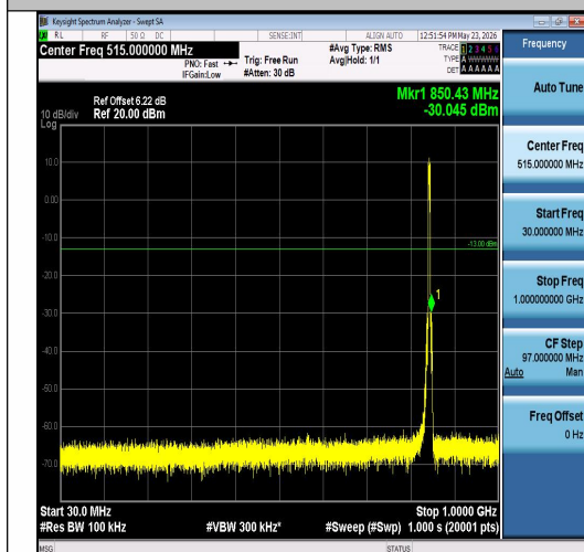
Band26(824-849)-5MHz-QPSK-27015-25RB#0-3 0~1000-PASS
