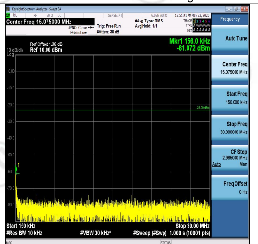
Band26(824-849)-5MHz-QPSK-27015-25RB#0-0 .15~30-PASS
