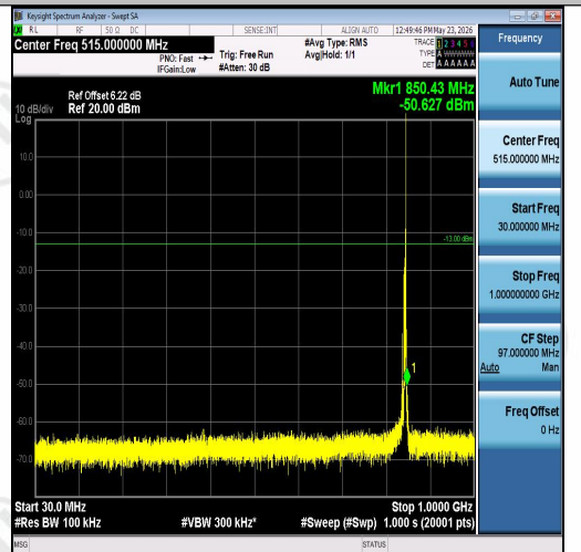
Band26(824-849)-5MHz-QPSK-27015-1RB#24-3 0~1000-PASS
