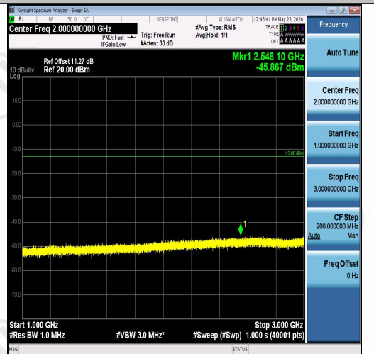
Band26(824-849)-5MHz-QPSK-26915-25RB#0-1 000~3000-PASS
