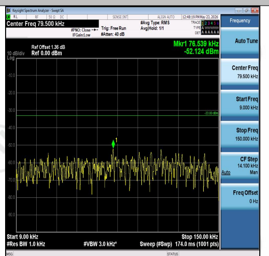
Band26(824-849)-5MHz-16QAM-27015-1RB#0- 0.009~0.15-PASS
