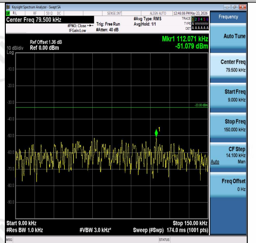
Band26(824-849)-5MHz-16QAM-26915-25RB#0 -0.009~0.15-PASS
