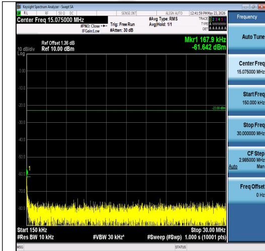
Band26(824-849)-5MHz-16QAM-26915-1RB#0-0.15~30-PASS
