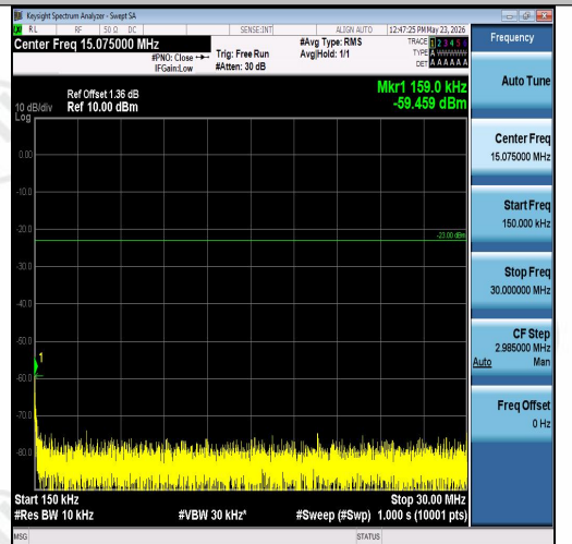
Band26(824-849)-5MHz-QPSK-27015-1RB#0-0. 15~30-PASS
