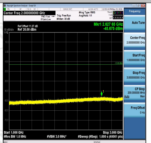
Band26(824-849)-5MHz-QPSK-27015-25RB#0-1 000~3000-PASS
