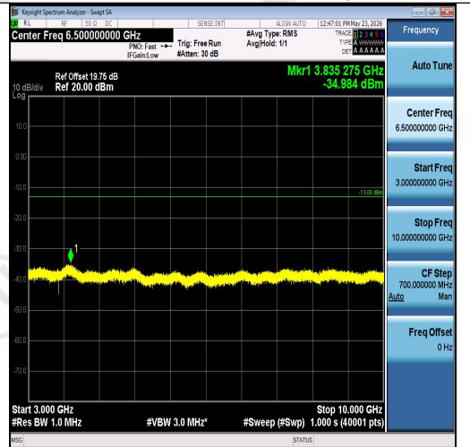
Band26(824-849)-5MHz-16QAM-26915-25RB#0 -3000~10000-PASS
