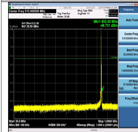
Band26(824-849)-5MHz-QPSK-27015-1RB#0-30 ~1000-PASS
