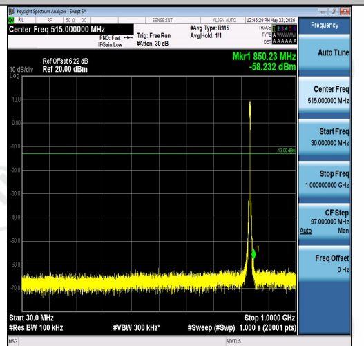
Band26(824-849)-5MHz-16QAM-26915-25RB#0 -30~1000-PASS
