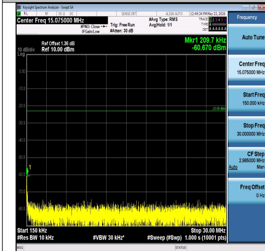
Band26(824-849)-5MHz-QPSK-27015-1RB#24-0 .15~30-PASS
