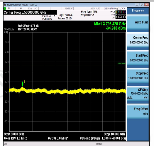
Band26(824-849)-5MHz-QPSK-27015-1RB#24-3 000~10000-PASS
