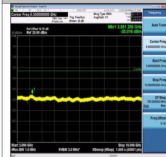
Band26(824-849)-5MHz-QPSK-27015-25RB#0-3 000~10000-PASS
