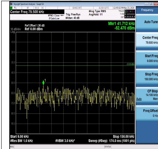
Band26(824-849)-5MHz-QPSK-26915-25RB#0-0 .009~0.15-PASS
