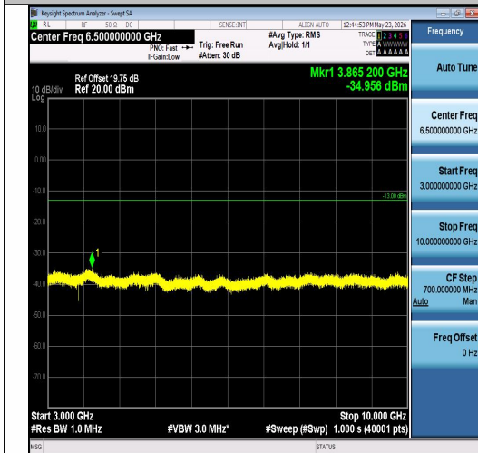
Band26(824-849)-5MHz-16QAM-26915-1RB#24 -3000~10000-PASS
