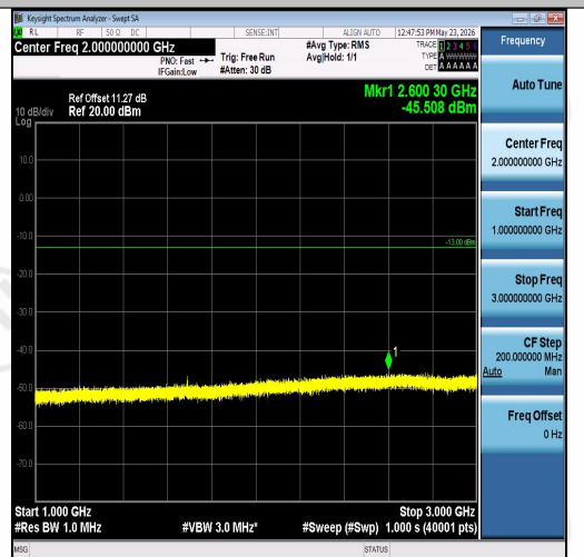
Band26(824-849)-5MHz-QPSK-27015-1RB#0-10 00~3000-PASS
