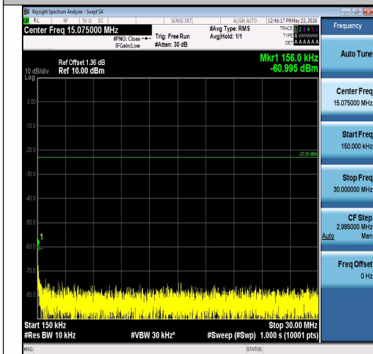
Band26(824-849)-5MHz-16QAM-26915-25RB#0 -0.15~30-PASS
