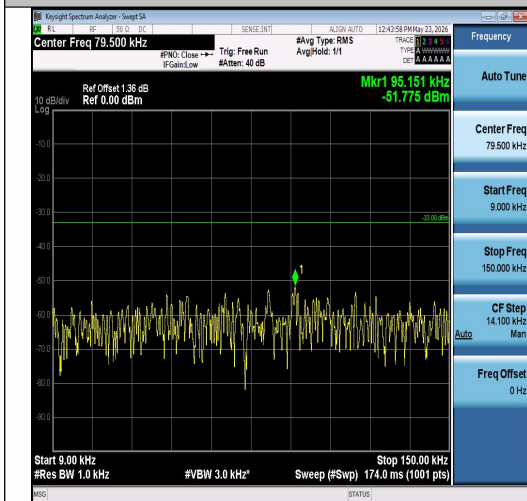
Band26(824-849)-5MHz-16QAM-26915-1RB#24-0.009~0.15-PASS
