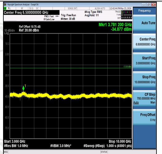
Band26(824-849)-5MHz-16QAM-26915-1RB#0-3000~10000-PASS
