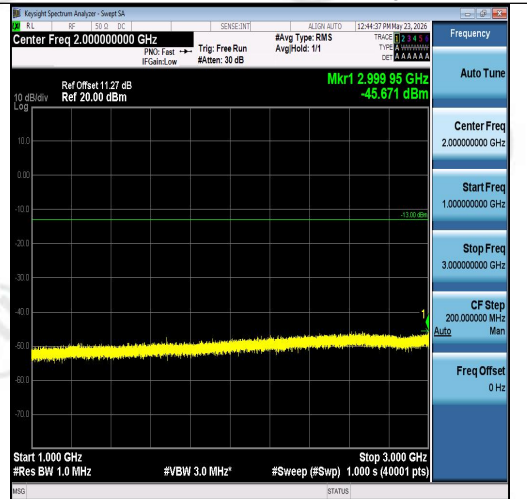
Band26(824-849)-5MHz-16QAM-26915-1RB#24 -1000~3000-PASS
