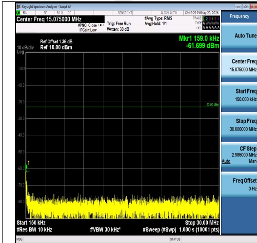
Band26(824-849)-5MHz-16QAM-27015-1RB#0-0.15~30-PASS
