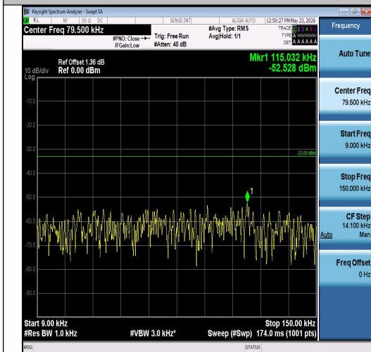
Band26(824-849)-5MHz-16QAM-27015-1RB#24-0.009~0.15-PASS
