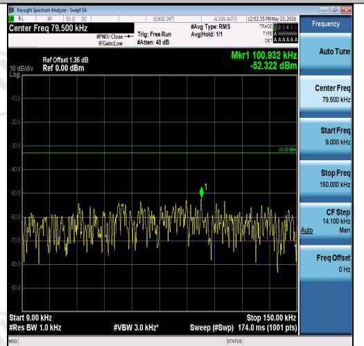
Band26(824-849)-5MHz-16QAM-27015-25RB#0 -0.009~0.15-PASS
