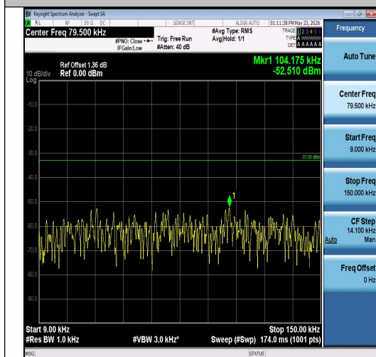
Band26(824-849)-10MHz-QPSK-26840-1RB#0-0 .009~0.15-PASS
