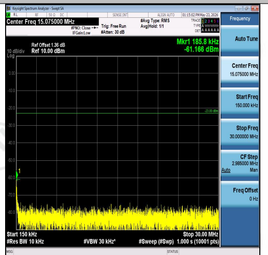
Band26(824-849)-10MHz-16QAM-26840-1RB#4 9-0.15~30-PASS
