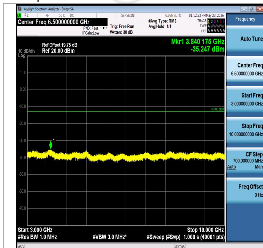
Band26(824-849)-10MHz-QPSK-26840-1RB#0-3 000~10000-PASS
