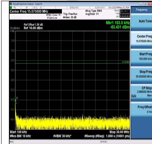
Band26(824-849)-10MHz-16QAM-26840-1RB#0 -0.15~30-PASS
