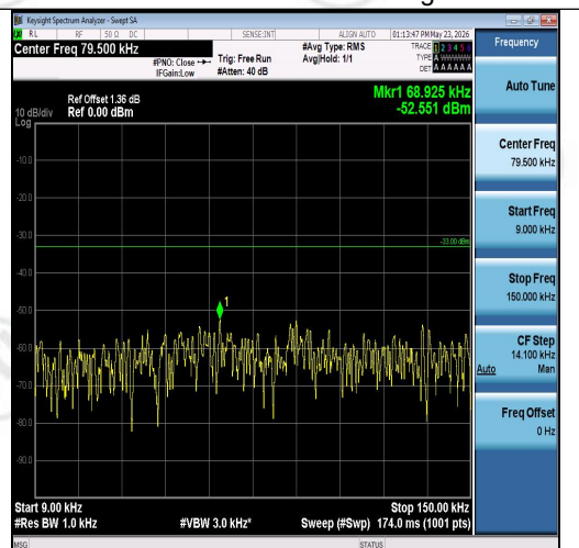
Band26(824-849)-10MHz-QPSK-26840-1RB#49- 0.009~0.15-PASS
