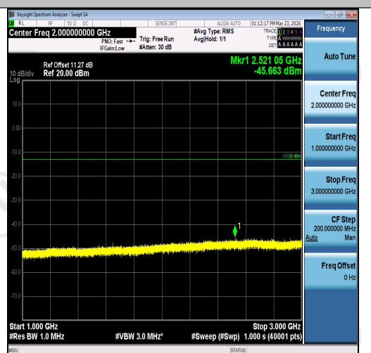
Band26(824-849)-10MHz-QPSK-26840-1RB#0-1 000~3000-PASS
