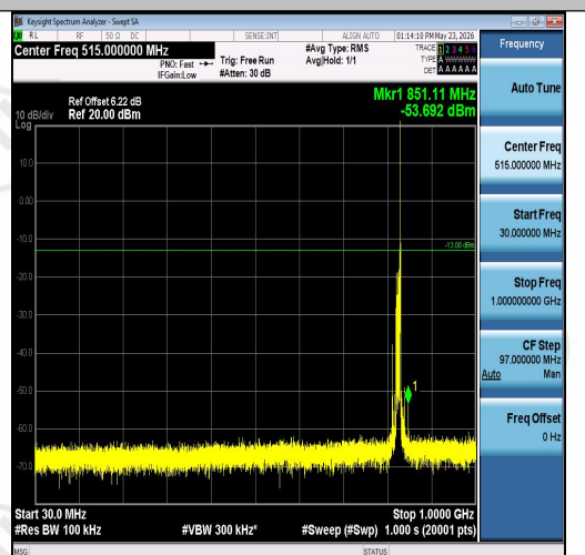
Band26(824-849)-10MHz-QPSK-26840-1RB#49- 30~1000-PASS
