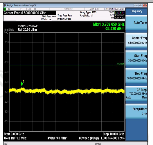
Band26(824-849)-10MHz-QPSK-26840-1RB#49- 3000~10000-PASS
