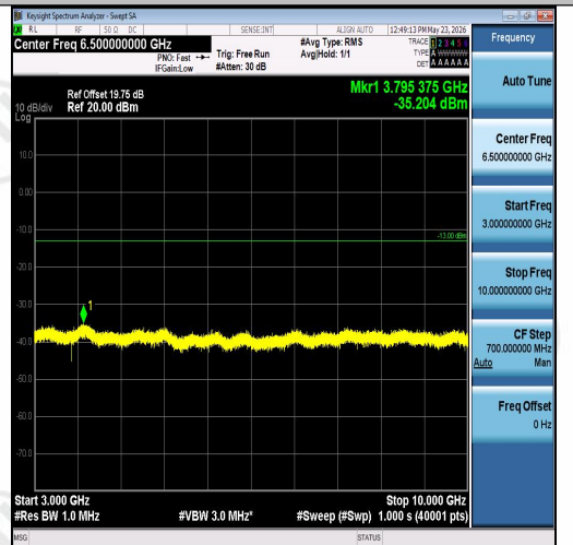
Band26(824-849)-5MHz-16QAM-27015-1RB#0-3000~10000-PASS
