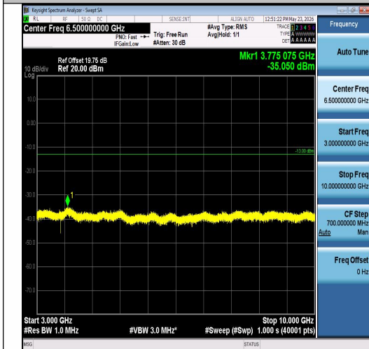
Band26(824-849)-5MHz-16QAM-27015-1RB#24 -3000~10000-PASS
