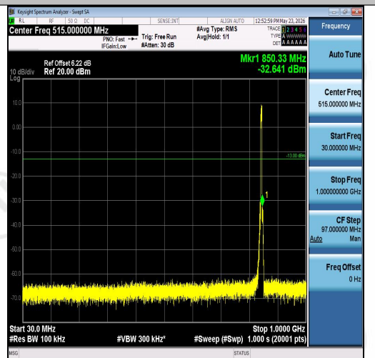
Band26(824-849)-5MHz-16QAM-27015-25RB#0 -30~1000-PASS
