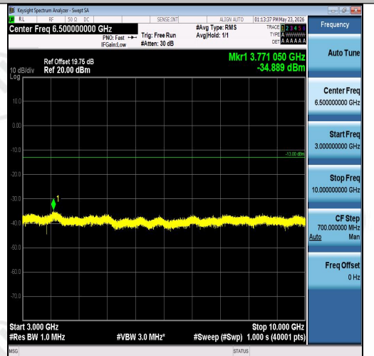
Band26(824-849)-10MHz-16QAM-26840-1RB#0 -3000~10000-PASS
