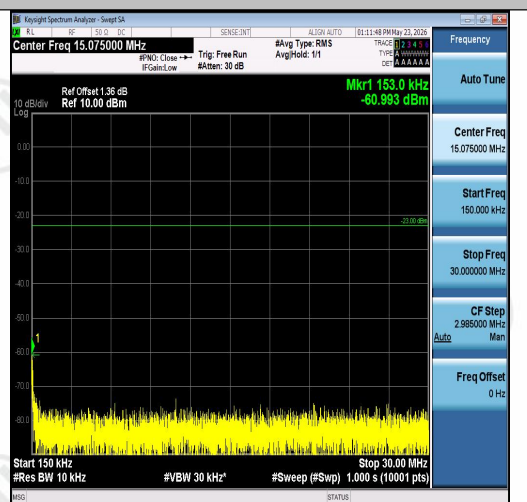
Band26(824-849)-10MHz-QPSK-26840-1RB#0-0 .15~30-PASS
