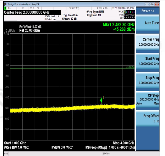
Band26(824-849)-5MHz-16QAM-27015-1RB#24 -1000~3000-PASS
