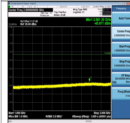
Band26(824-849)-5MHz-16QAM-27015-1RB#0-1000~3000-PASS
