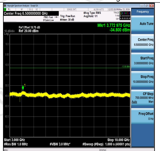
Band26(824-849)-5MHz-16QAM-27015-25RB#0 -3000~10000-PASS
