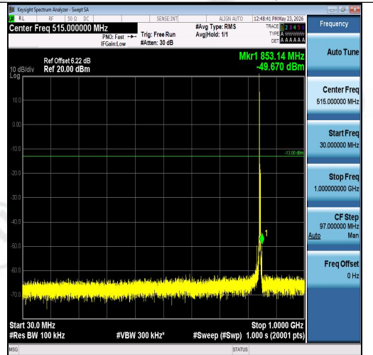
Band26(824-849)-5MHz-16QAM-27015-1RB#0-30~1000-PASS
