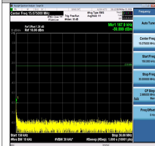
Band26(824-849)-10MHz-QPSK-26840-1RB#49- 0.15~30-PASS
