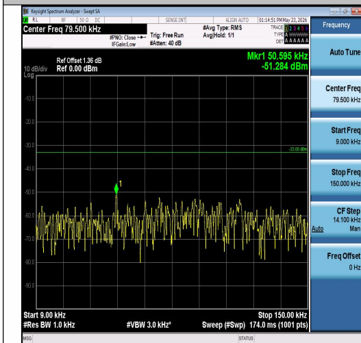
Band26(824-849)-10MHz-16QAM-26840-1RB#4 9-0.009~0.15-PASS
