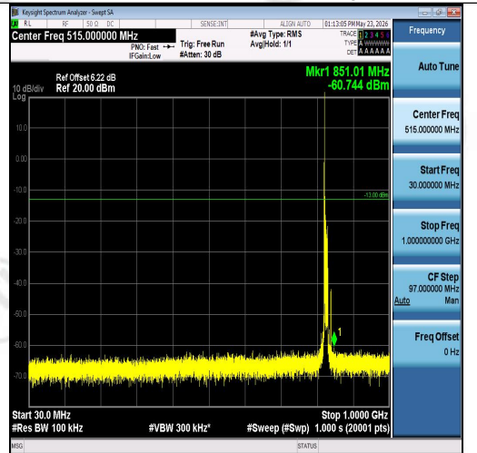
Band26(824-849)-10MHz-16QAM-26840-1RB#0 -30~1000-PASS
