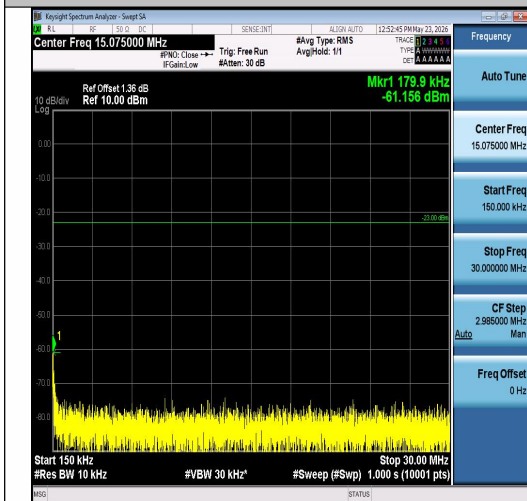
Band26(824-849)-5MHz-16QAM-27015-25RB#0 -0.15~30-PASS
