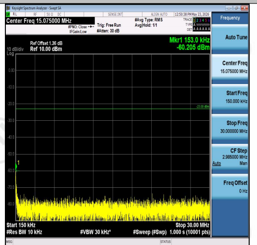
Band26(824-849)-5MHz-16QAM-27015-1RB#24-0.15~30-PASS
