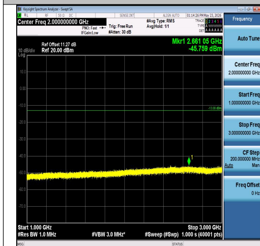
Band26(824-849)-10MHz-QPSK-26840-1RB#49- 1000~3000-PASS
