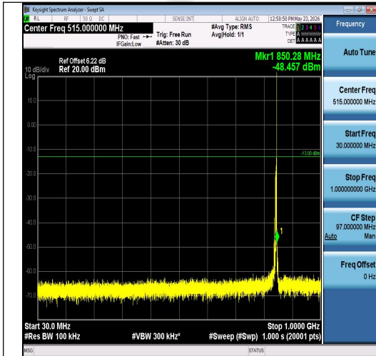
Band26(824-849)-5MHz-16QAM-27015-1RB#24 -30~1000-PASS
