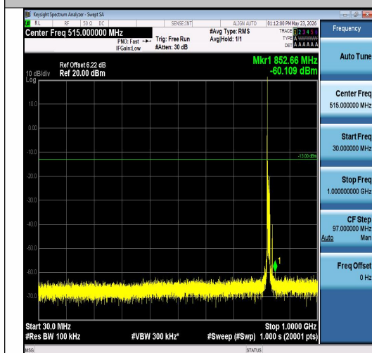
Band26(824-849)-10MHz-QPSK-26840-1RB#0-3 0~1000-PASS
