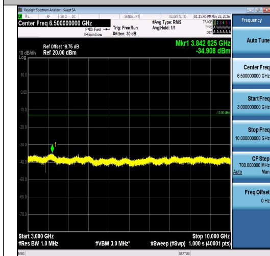
Band26(824-849)-10MHz-16QAM-26840-1RB#4 9-3000~10000-PASS
