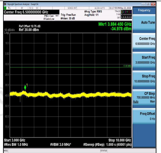
Band26(824-849)-10MHz-16QAM-26840-50RB# 0-3000~10000-PASS
