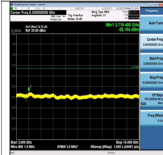
Band26(824-849)-10MHz-16QAM-26915-1RB#4 9-3000~10000-PASS
