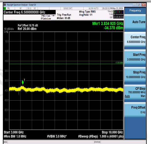
Band26(824-849)-10MHz-QPSK-26915-1RB#49- 3000~10000-PASS
