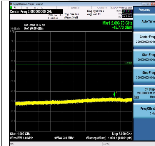
Band26(824-849)-10MHz-16QAM-26840-50RB# 0-1000~3000-PASS
