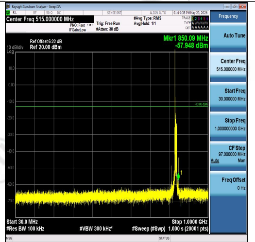
Band26(824-849)-10MHz-16QAM-26915-1RB#0 -30~1000-PASS
