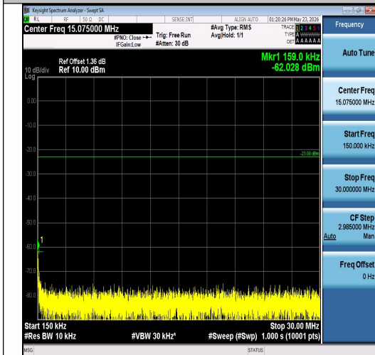
Band26(824-849)-10MHz-QPSK-26915-1RB#49- 0.15~30-PASS
