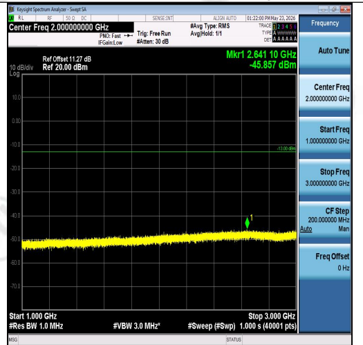
Band26(824-849)-10MHz-16QAM-26915-1RB#4 9-1000~3000-PASS
