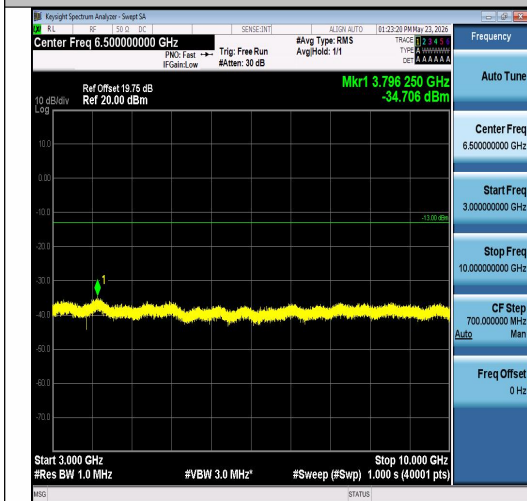
Band26(824-849)-10MHz-QPSK-26915-50RB#0-3000~10000-PASS
