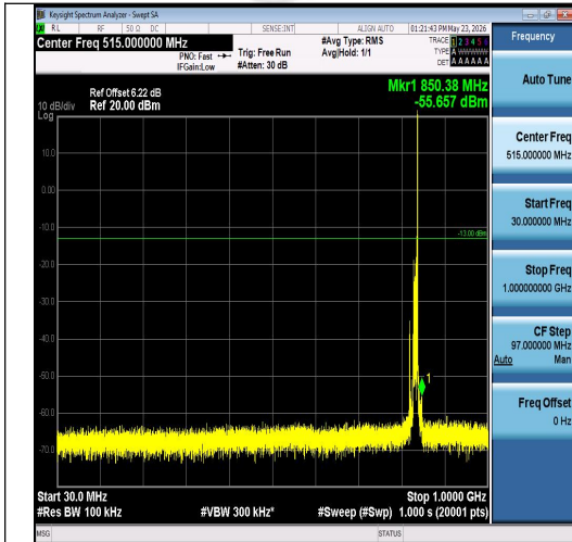
Band26(824-849)-10MHz-16QAM-26915-1RB#4 9-30~1000-PASS
