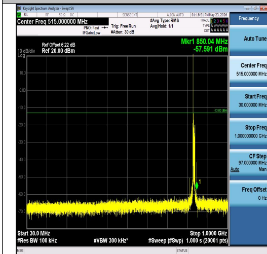
Band26(824-849)-10MHz-QPSK-26915-1RB#0-3 0~1000-PASS
