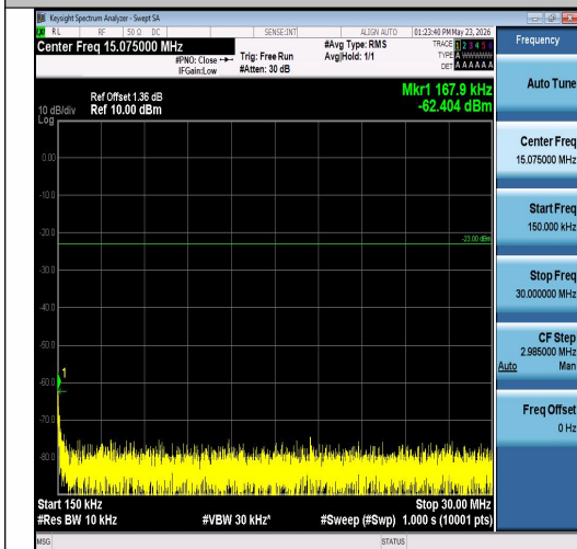
Band26(824-849)-10MHz-16QAM-26915-50RB#4 0-0.15~30-PASS
