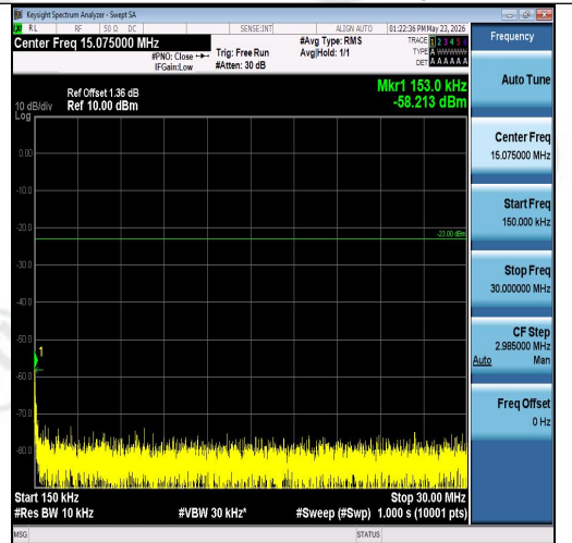
Band26(824-849)-10MHz-QPSK-26915-50RB#0-0.15~30-PASS
