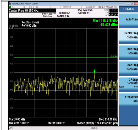
Band26(824-849)-10MHz-QPSK-26915-1RB#0-0 .009~0.15-PASS
