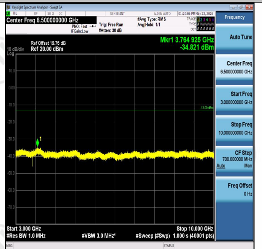
Band26(824-849)-10MHz-16QAM-26915-1RB#0 -3000~10000-PASS
