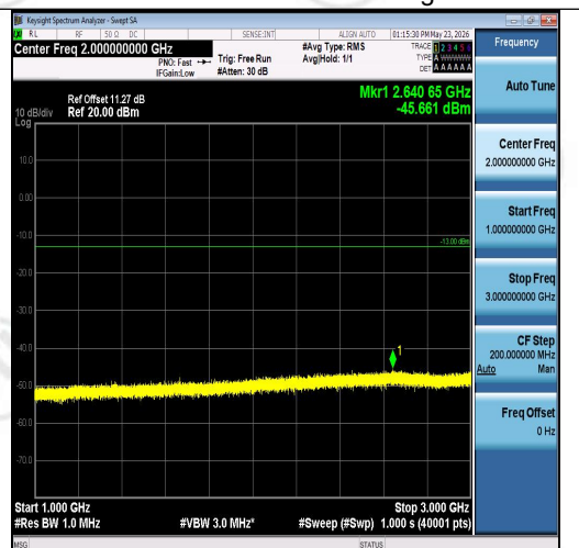
Band26(824-849)-10MHz-16QAM-26840-1RB#4 9-1000~3000-PASS
