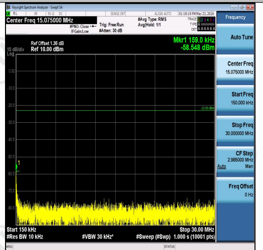
Band26(824-849)-10MHz-QPSK-26915-1RB#0-0 .15~30-PASS
