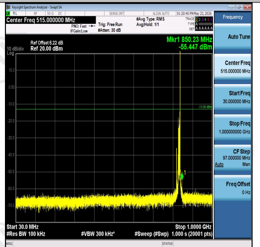
Band26(824-849)-10MHz-QPSK-26915-1RB#49- 30~1000-PASS
