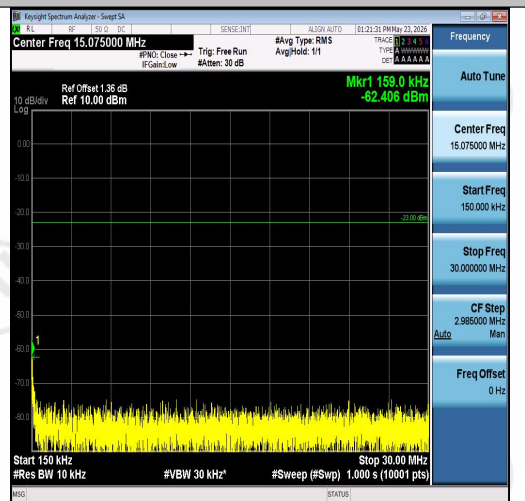
Band26(824-849)-10MHz-16QAM-26915-1RB#4 9-0.15~30-PASS
