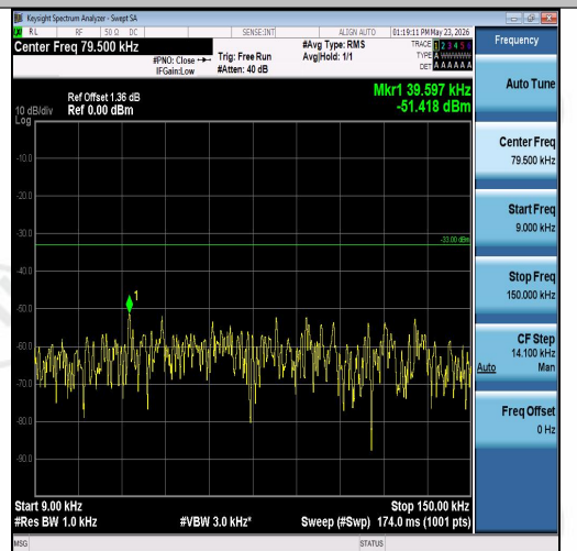
Band26(824-849)-10MHz-16QAM-26915-1RB#0-0.009~0.15-PASS
