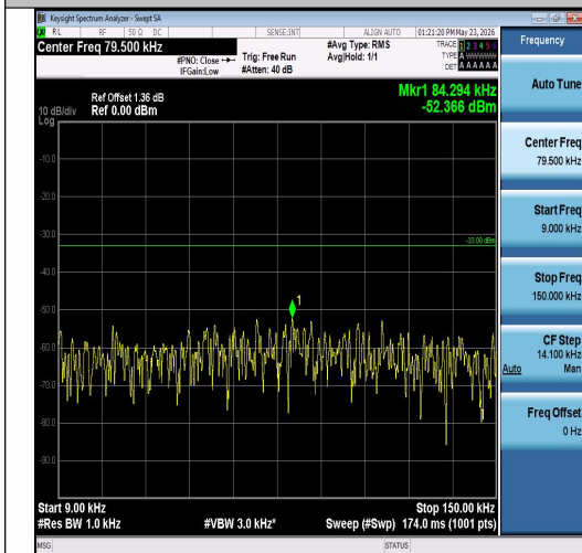
Band26(824-849)-10MHz-16QAM-26915-1RB#4 9-0.009~0.15-PASS
