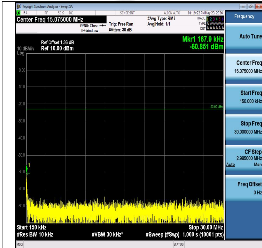
Band26(824-849)-10MHz-16QAM-26915-1RB#0 -0.15~30-PASS
