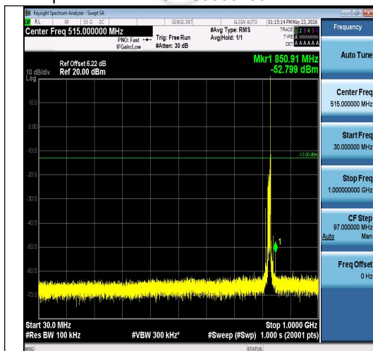
Band26(824-849)-10MHz-16QAM-26840-1RB#4 9-30~1000-PASS
