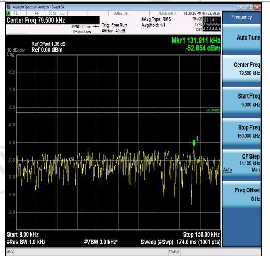
Band26(824-849)-10MHz-QPSK-26915-1RB#49- 0.009~0.15-PASS
