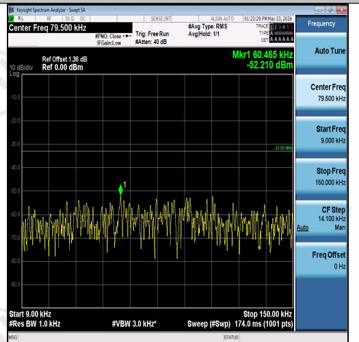
Band26(824-849)-10MHz-16QAM-26915-50RB#4 0-0.009~0.15-PASS
