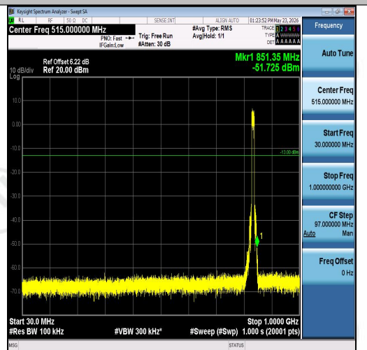
Band26(824-849)-10MHz-16QAM-26915-50RB#4 0-30~1000-PASS
