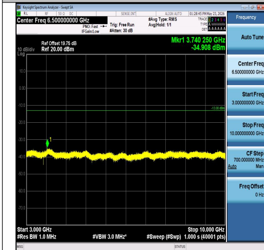
Band26(824-849)-10MHz-16QAM-26990-1RB#4 9-3000~10000-PASS
