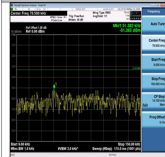
Band26(824-849)-10MHz-16QAM-26990-1RB#4 9-0.009~0.15-PASS
