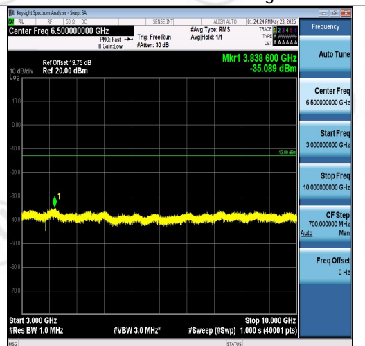
Band26(824-849)-10MHz-16QAM-26915-50RB# 0-3000~10000-PASS
