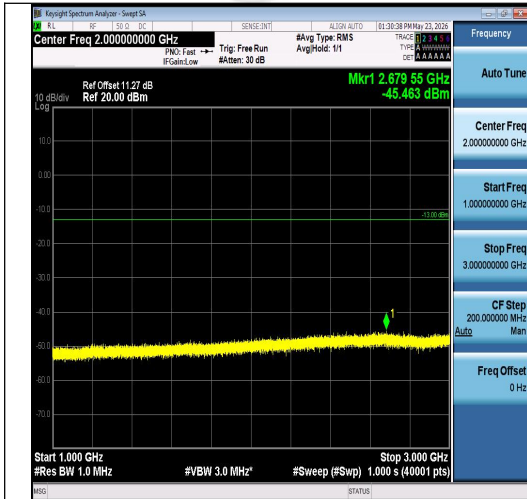
Band26(824-849)-10MHz-16QAM-26990-50RB# 0-1000~3000-PASS
