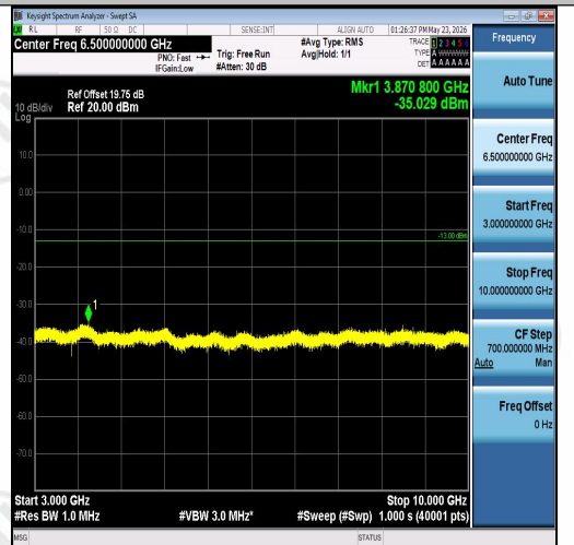
Band26(824-849)-10MHz-16QAM-26990-1RB#0 -3000~10000-PASS
