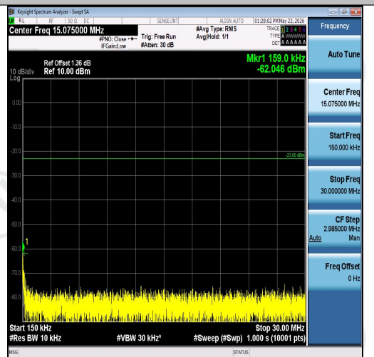
Band26(824-849)-10MHz-16QAM-26990-1RB#4 9-0.15~30-PASS
