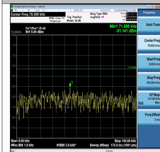
Band26(824-849)-10MHz-QPSK-26990-1RB#0-0 .009~0.15-PASS
