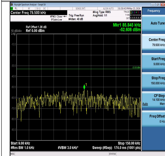
Band26(824-849)-15MHz-QPSK-26865-1RB#0-0 .009~0.15-PASS
