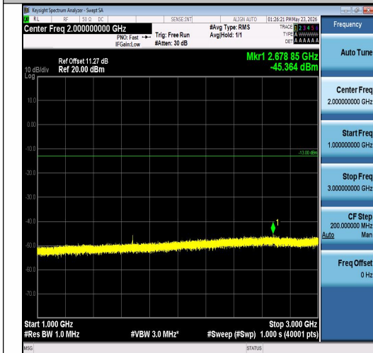
Band26(824-849)-10MHz-16QAM-26990-1RB#0 -1000~3000-PASS
