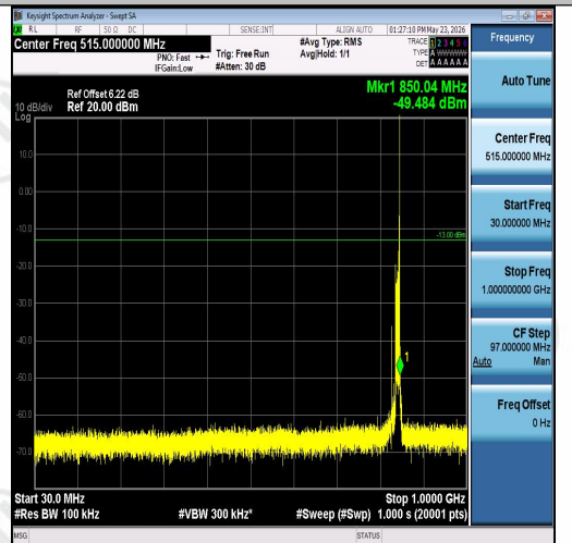
Band26(824-849)-10MHz-QPSK-26990-1RB#49- 30~1000-PASS
