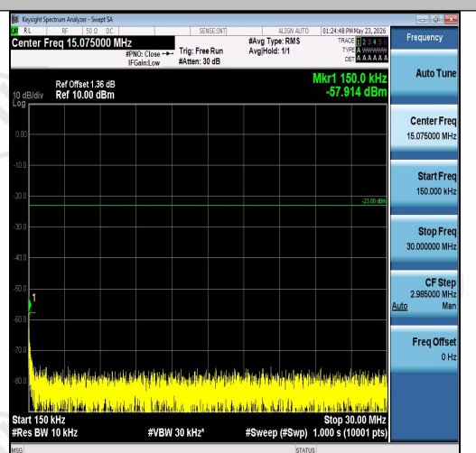
Band26(824-849)-10MHz-QPSK-26990-1RB#0-0 .15~30-PASS
