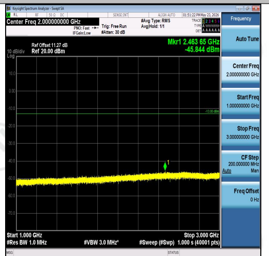
Band26(824-849)-15MHz-QPSK-26865-1RB#0-1 000~3000-PASS
