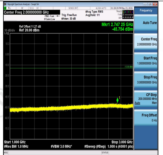
Band26(824-849)-10MHz-16QAM-26990-1RB#4 9-1000~3000-PASS
