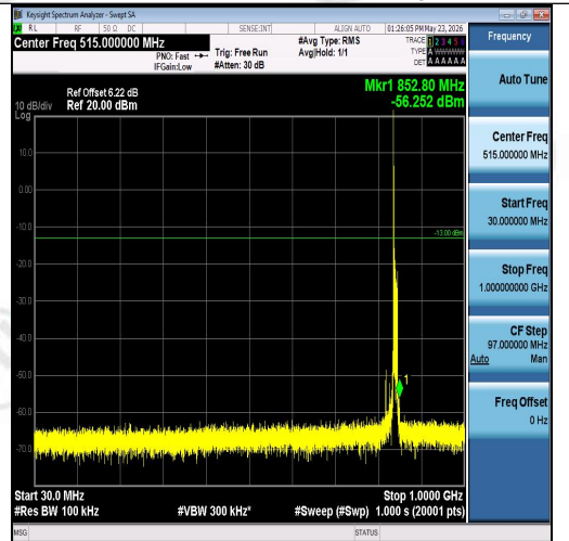
Band26(824-849)-10MHz-16QAM-26990-1RB#0 -30~1000-PASS
