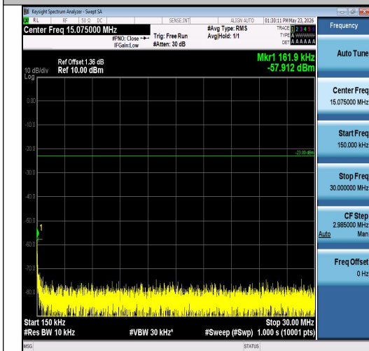
Band26(824-849)-10MHz-16QAM-26990-50RB#4 0-0.15~30-PASS
