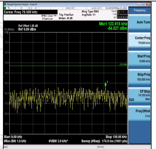
Band26(824-849)-10MHz-16QAM-26990-50RB#4 0-0.009~0.15-PASS
