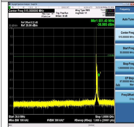
Band26(824-849)-15MHz-QPSK-26865-1RB#0-3 0~1000-PASS
