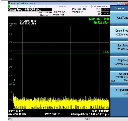
Band26(824-849)-10MHz-16QAM-26990-1RB#0 -0.15~30-PASS
