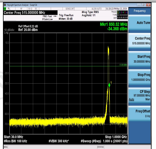
Band26(824-849)-10MHz-16QAM-26990-50RB#4 0-30~1000-PASS
