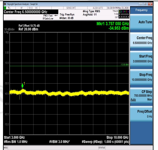
Band26(824-849)-10MHz-16QAM-26990-50RB# 0-3000~10000-PASS
