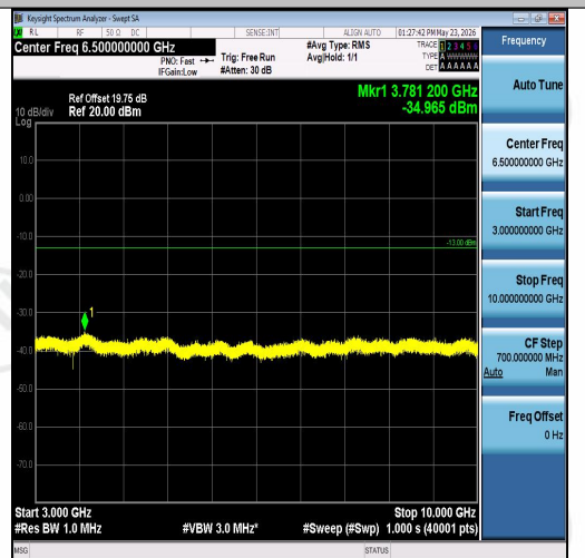
Band26(824-849)-10MHz-QPSK-26990-1RB#49- 3000~10000-PASS
