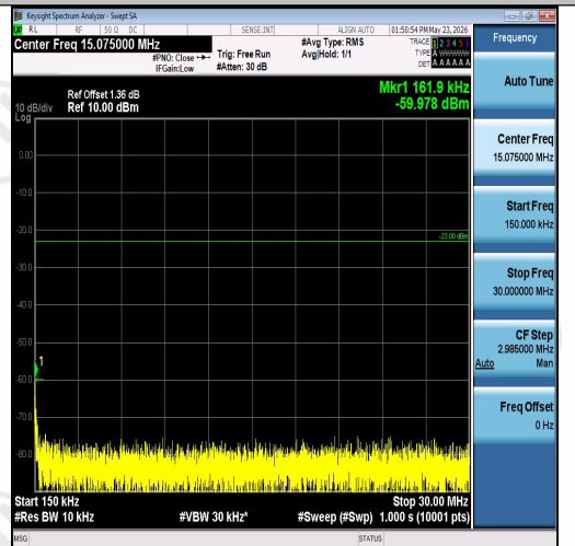
Band26(824-849)-15MHz-QPSK-26865-1RB#0-0 .15~30-PASS
