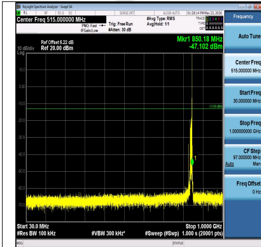
Band26(824-849)-10MHz-16QAM-26990-1RB#4 9-30~1000-PASS
