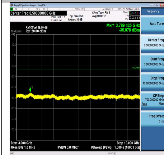
Band26(824-849)-15MHz-16QAM-26865-1RB#7 4-3000~10000-PASS
