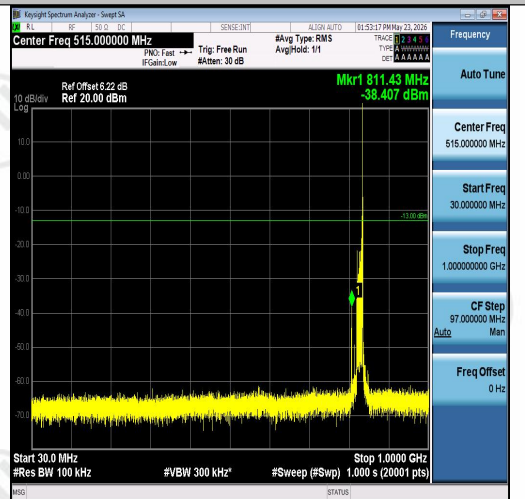
Band26(824-849)-15MHz-QPSK-26865-1RB#74- 30~1000-PASS
