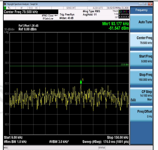
Band26(824-849)-15MHz-QPSK-26865-1RB#74- 0.009~0.15-PASS
