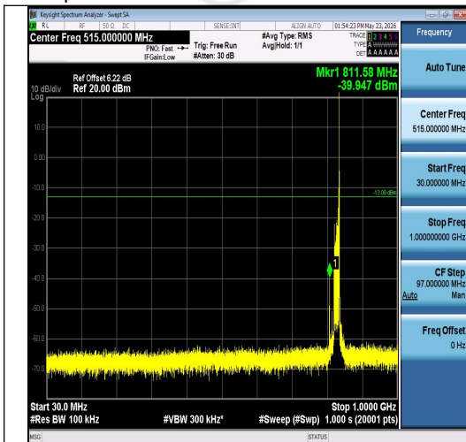
Band26(824-849)-15MHz-16QAM-26865-1RB#7 4-30~1000-PASS
