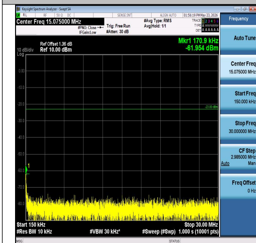
Band26(824-849)-15MHz-16QAM-26865-75RB# 0-0.15~30-PASS
