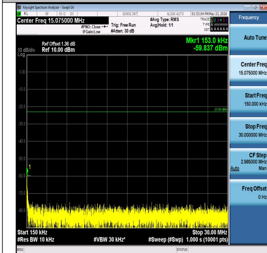
Band26(824-849)-15MHz-QPSK-26865-1RB#74- 0.15~30-PASS
