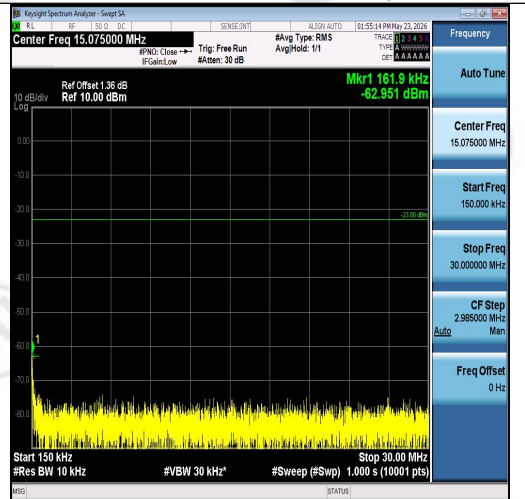
Band26(824-849)-15MHz-QPSK-26865-75RB#0-0.15~30-PASS
