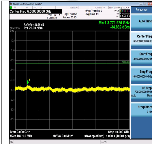
Band26(824-849)-15MHz-QPSK-26865-1RB#0-3 000~10000-PASS
