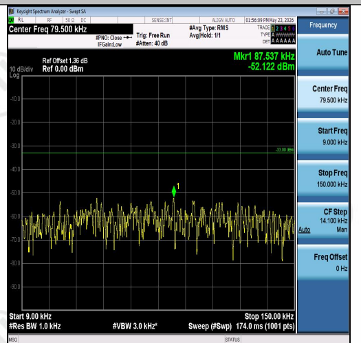
Band26(824-849)-15MHz-16QAM-26865-75RB# 0-0.009~0.15-PASS
