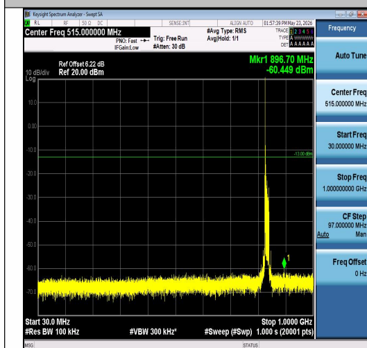
Band26(824-849)-15MHz-QPSK-26915-1RB#0-0 0~1000-PASS
