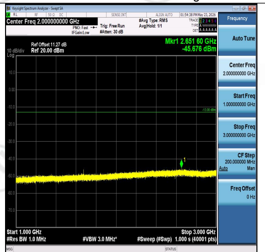
Band26(824-849)-15MHz-16QAM-26865-1RB#7 4-1000~3000-PASS
