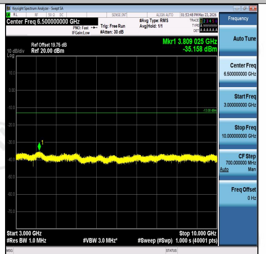
Band26(824-849)-15MHz-QPSK-26865-1RB#74- 3000~10000-PASS
