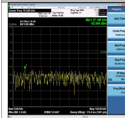
Band26(824-849)-15MHz-QPSK-26915-1RB#0-0 .009~0.15-PASS
