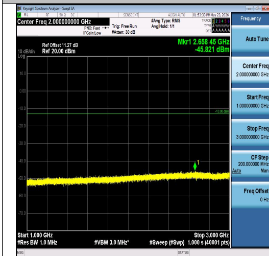
Band26(824-849)-15MHz-QPSK-26865-1RB#74- 1000~3000-PASS
