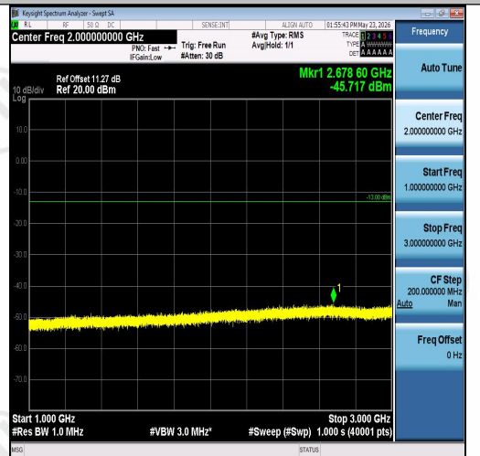
Band26(824-849)-15MHz-QPSK-26865-75RB#0-1000~3000-PASS
