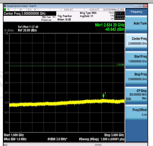
Band26(824-849)-15MHz-QPSK-26915-1RB#0-0 000~3000-PASS
