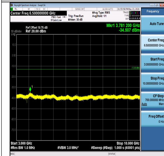
Band26(824-849)-15MHz-QPSK-26865-75RB#0-3000~10000-PASS
