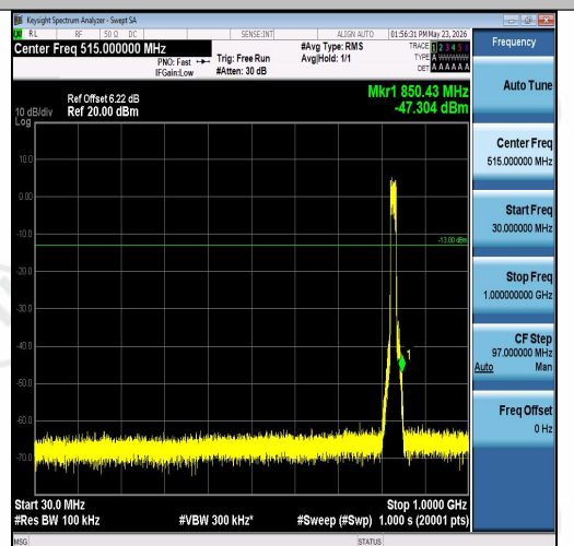
Band26(824-849)-15MHz-16QAM-26865-75RB# 0-30~1000-PASS
