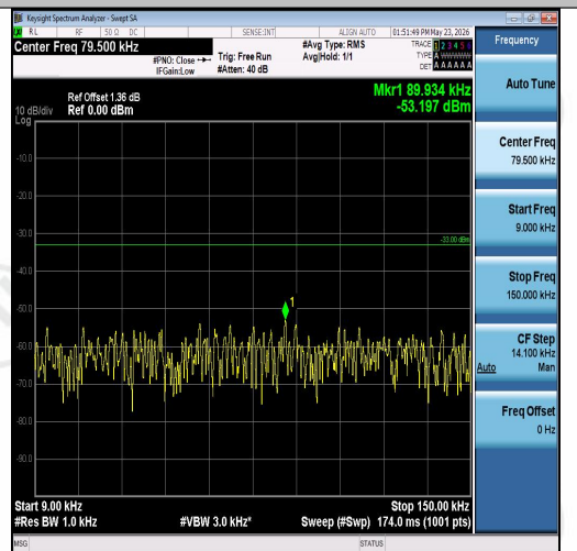
Band26(824-849)-15MHz-16QAM-26865-1RB#0-0.009~0.15-PASS
