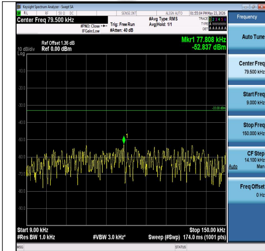
Band26(824-849)-15MHz-QPSK-26865-75RB#0-0.009~0.15-PASS
