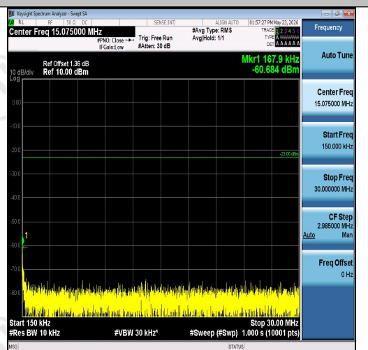
Band26(824-849)-15MHz-QPSK-26915-1RB#0-0 .15~30-PASS
