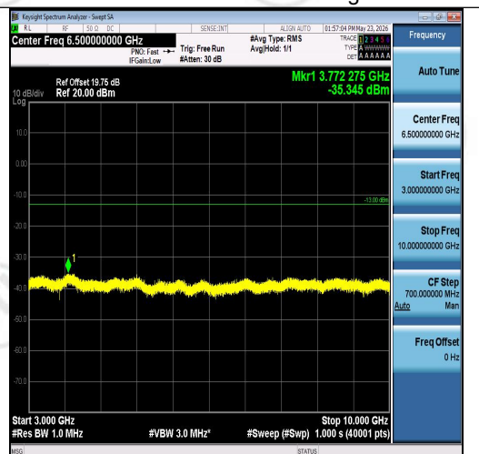
Band26(824-849)-15MHz-16QAM-26865-75RB# 0-3000~10000-PASS
