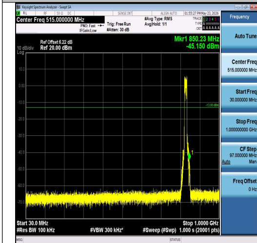
Band26(824-849)-15MHz-QPSK-26865-75RB#0-30~1000-PASS
