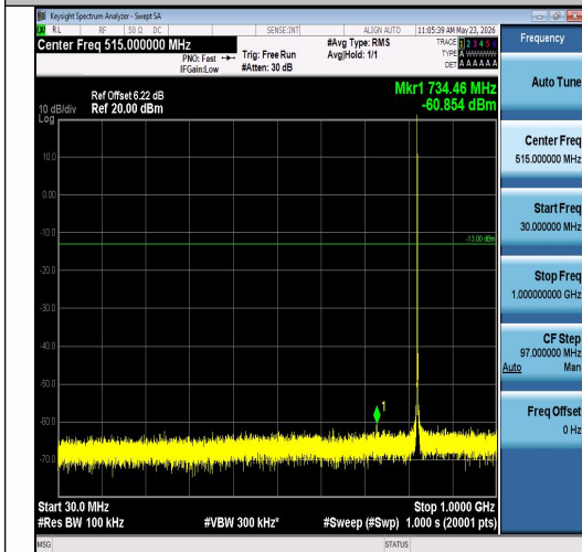
Band26(824-849)-1.4MHz-QPSK-26797-1RB#0-30~1000-PASS
