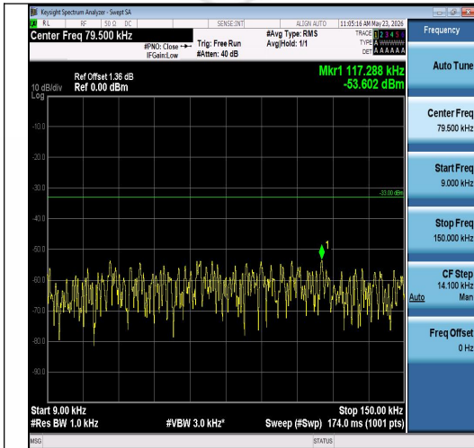
Band26(824-849)-1.4MHz-QPSK-26797-1RB#0-0.009~0.15-PASS
