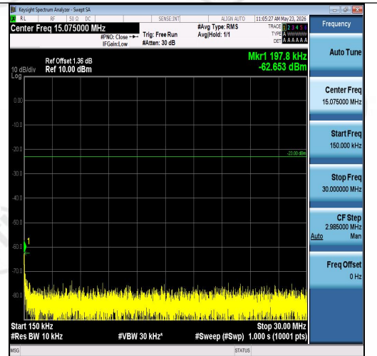
Band26(824-849)-1.4MHz-QPSK-26797-1RB#0-0.15~30-PASS
