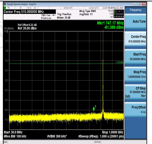
Band26(824-849)-1.4MHz-QPSK-26797-1RB#5-30~1000-PASS
