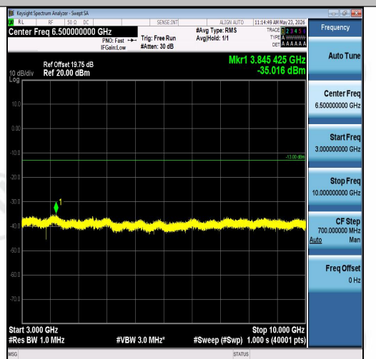
Band26(824-849)-1.4MHz-QPSK-26915-1RB#5-3000~10000-PASS
