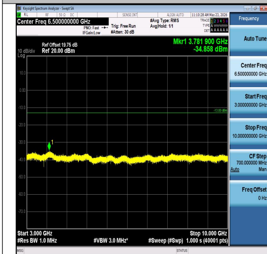
Band26(824-849)-1.4MHz-QPSK-26797-6RB#0-3000~10000-PASS
