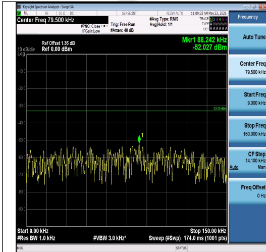
Band26(824-849)-1.4MHz-QPSK-26797-6RB#0-0.009~0.15-PASS
