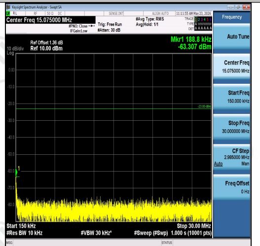
Band26(824-849)-1.4MHz-QPSK-26915-1RB#0- 0.15~30-PASS
