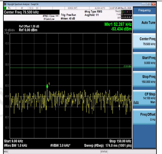
Band26(824-849)-1.4MHz-QPSK-26797-1RB#5-0.009~0.15-PASS
