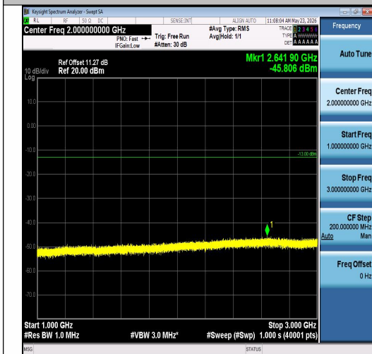
Band26(824-849)-1.4MHz-QPSK-26797-1RB#5-1000~3000-PASS
