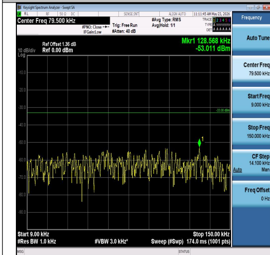
Band26(824-849)-1.4MHz-QPSK-26915-1RB#0- 0.009~0.15-PASS
