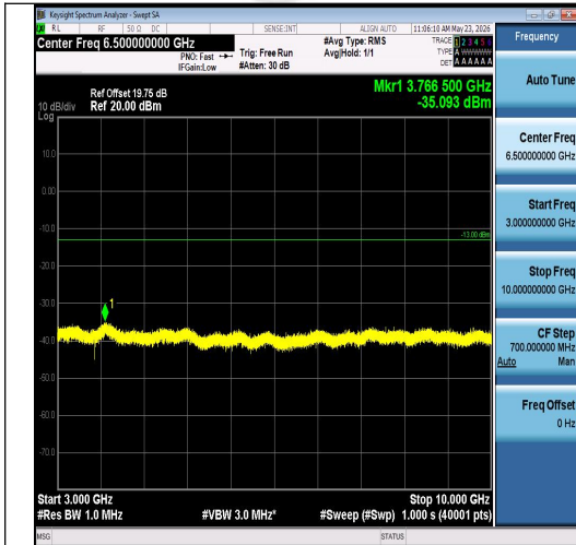
Band26(824-849)-1.4MHz-QPSK-26797-1RB#0-3000~10000-PASS
