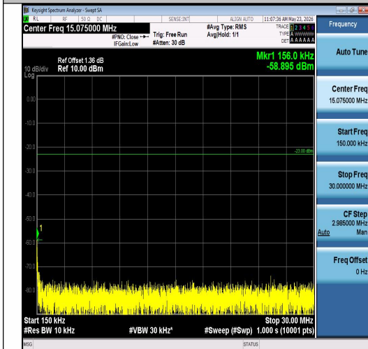
Band26(824-849)-1.4MHz-QPSK-26797-1RB#5-0.15~30-PASS
