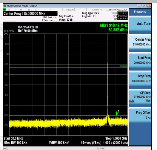
Band26(824-849)-1.4MHz-QPSK-26915-1RB#5-30~1000-PASS
