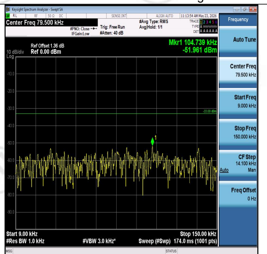
Band26(824-849)-1.4MHz-QPSK-26915-1RB#5-0.009~0.15-PASS
