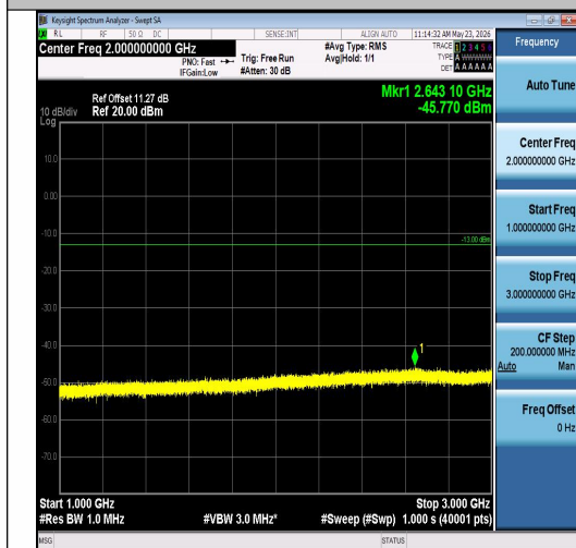
Band26(824-849)-1.4MHz-QPSK-26915-1RB#5-1000~3000-PASS
