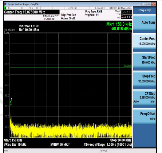
Band26(824-849)-1.4MHz-QPSK-26797-6RB#0-0.15~30-PASS
