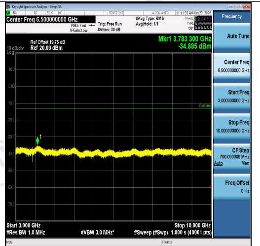
Band26(824-849)-1.4MHz-16QAM-26797-6RB#0 -3000~10000-PASS
