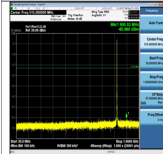
Band26(824-849)-1.4MHz-QPSK-26797-6RB#0-30~1000-PASS
