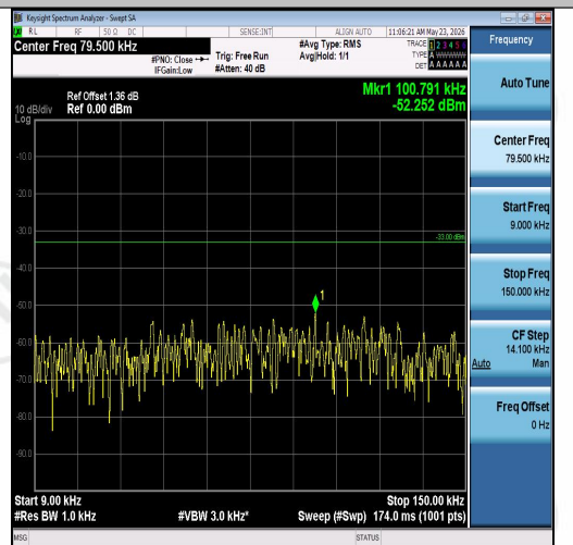
Band26(824-849)-1.4MHz-16QAM-26797-1RB#0-0.009~0.15-PASS
