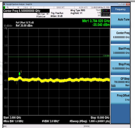
Band26(824-849)-1.4MHz-QPSK-26797-1RB#5-3000~10000-PASS
