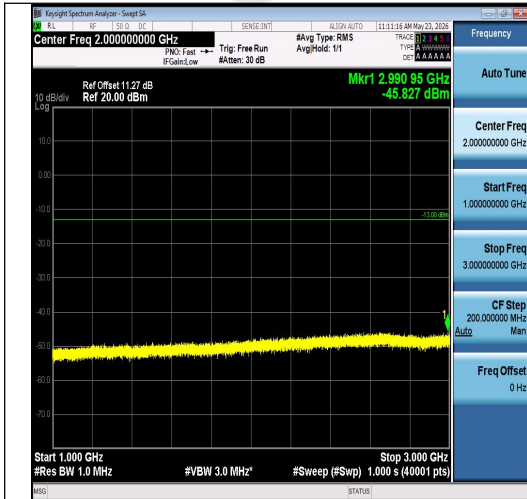
Band26(824-849)-1.4MHz-16QAM-26797-6RB#0 -1000~3000-PASS
