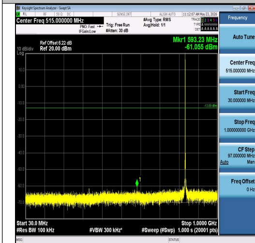
Band26(824-849)-1.4MHz-QPSK-26915-1RB#0- 30~1000-PASS
