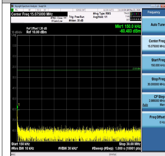
Band26(824-849)-1.4MHz-QPSK-26915-1RB#5-0.15~30-PASS
