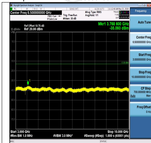
Band26(824-849)-1.4MHz-QPSK-26915-1RB#0-3000~10000-PASS
