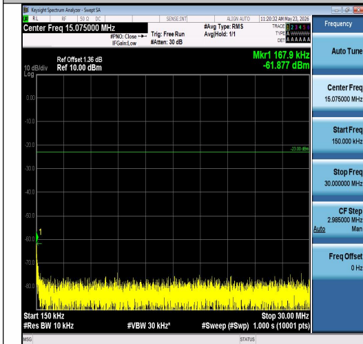
Band26(824-849)-1.4MHz-QPSK-27033-1RB#5-0.15~30-PASS
