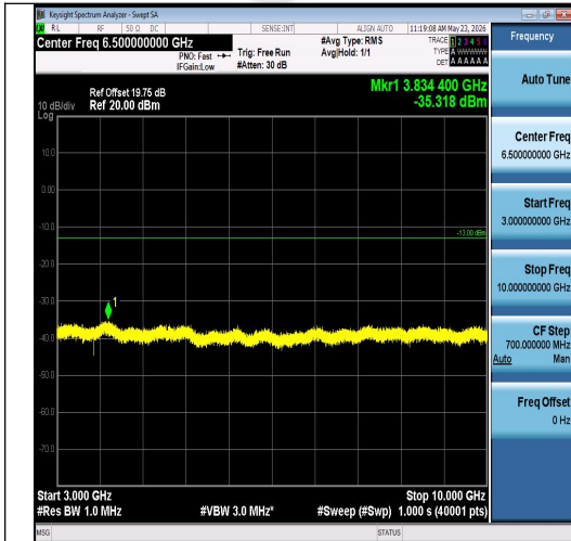
Band26(824-849)-1.4MHz-QPSK-27033-1RB#0-3000~10000-PASS
