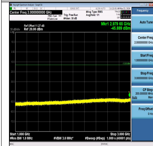
Band26(824-849)-1.4MHz-QPSK-27033-1RB#5-1000~3000-PASS
