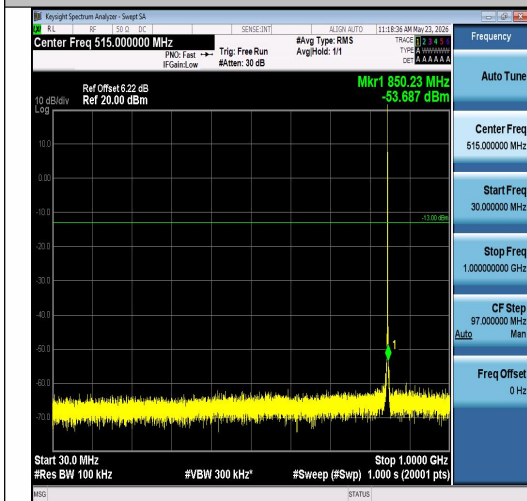
Band26(824-849)-1.4MHz-QPSK-27033-1RB#0- 30~1000-PASS
