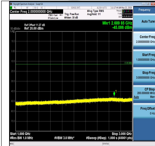
Band26(824-849)-1.4MHz-16QAM-26915-6RB#0 -1000~3000-PASS
