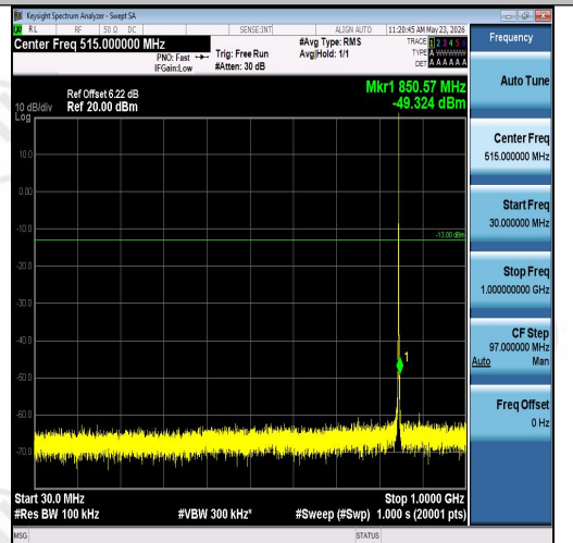
Band26(824-849)-1.4MHz-QPSK-27033-1RB#5-30~1000-PASS
