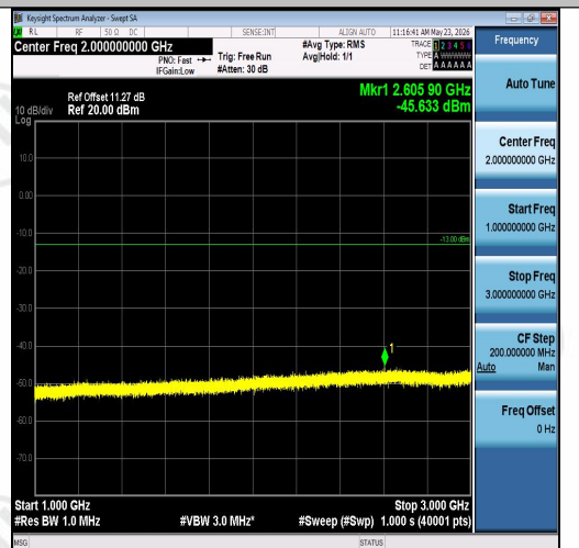
Band26(824-849)-1.4MHz-QPSK-26915-6RB#0-1000~3000-PASS
