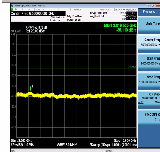
Band26(824-849)-1.4MHz-QPSK-26915-6RB#0-3000~10000-PASS
