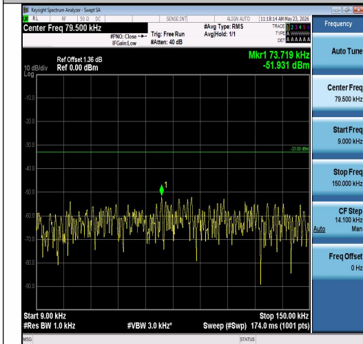
Band26(824-849)-1.4MHz-QPSK-27033-1RB#0- 0.009~0.15-PASS
