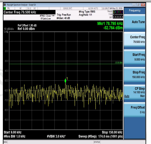
Band26(824-849)-1.4MHz-16QAM-27033-1RB#0-0.009~0.15-PASS
