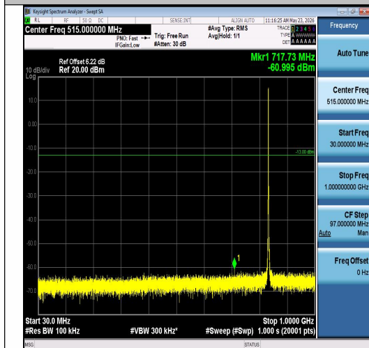
Band26(824-849)-1.4MHz-QPSK-26915-6RB#0-30~1000-PASS
