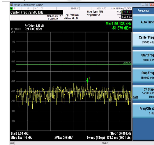
Band26(824-849)-1.4MHz-QPSK-26915-6RB#0-0.009~0.15-PASS
