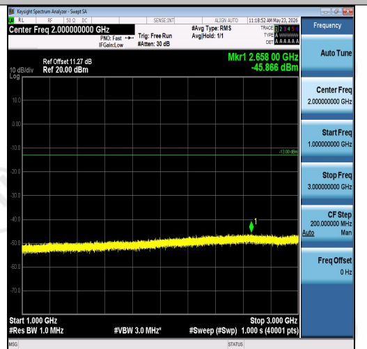
Band26(824-849)-1.4MHz-QPSK-27033-1RB#0- 1000~3000-PASS
