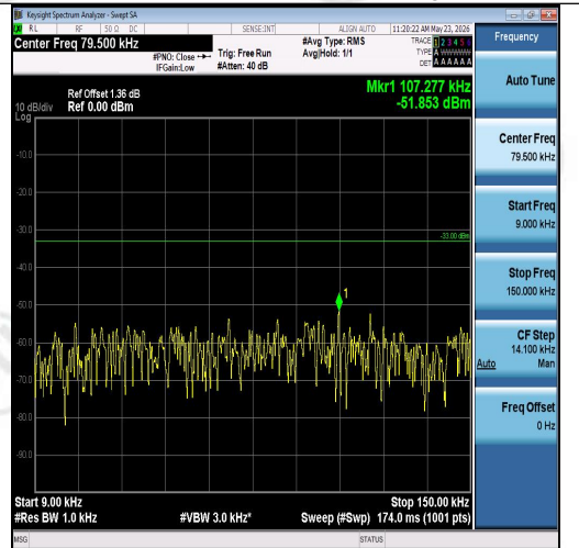
Band26(824-849)-1.4MHz-QPSK-27033-1RB#5-0.009~0.15-PASS
