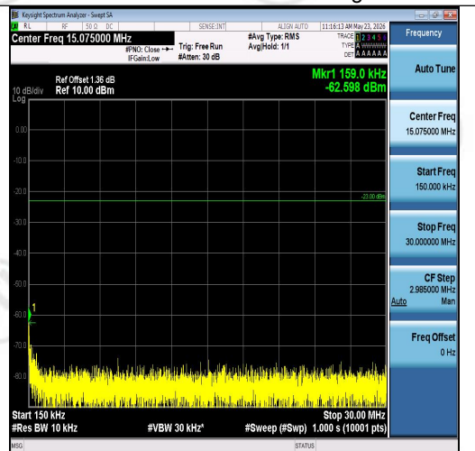
Band26(824-849)-1.4MHz-QPSK-26915-6RB#0-0.15~30-PASS
