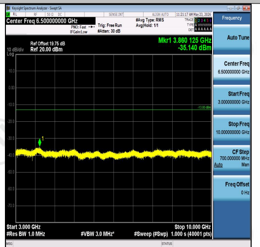
Band26(824-849)-1.4MHz-QPSK-27033-1RB#5-3000~10000-PASS
