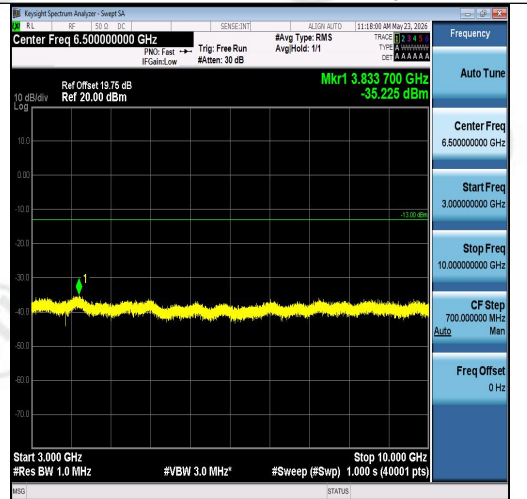
Band26(824-849)-1.4MHz-16QAM-26915-6RB#0 -3000~10000-PASS
