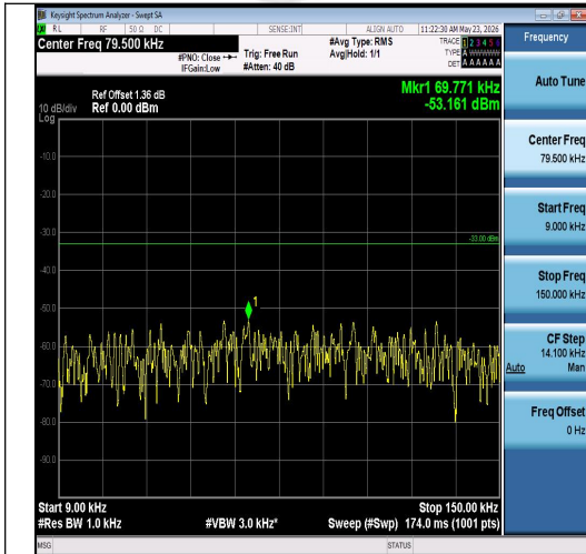
Band26(824-849)-1.4MHz-QPSK-27033-6RB#0-0.009~0.15-PASS
