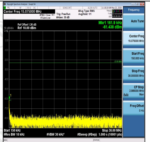
Band26(824-849)-1.4MHz-QPSK-27033-1RB#0- 0.15~30-PASS
