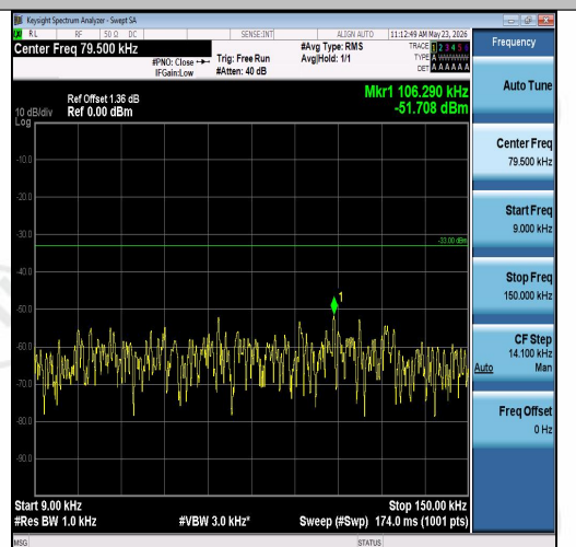
Band26(824-849)-1.4MHz-16QAM-26915-1RB#0-0.009~0.15-PASS
