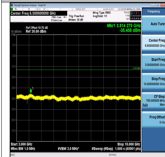
Band26(824-849)-1.4MHz-QPSK-27033-6RB#0-3000~10000-PASS
