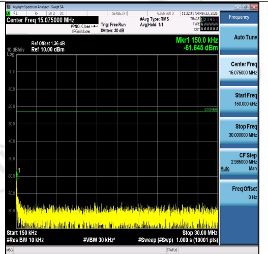
Band26(824-849)-1.4MHz-QPSK-27033-6RB#0-0.15~30-PASS
