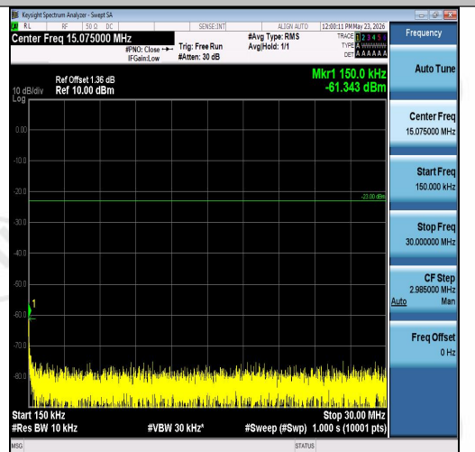
Band26(824-849)-3MHz-16QAM-26805-1RB#14-0.15~30-PASS
