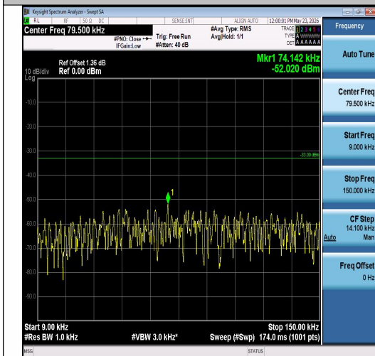
Band26(824-849)-3MHz-16QAM-26805-1RB#14-0.009~0.15-PASS
