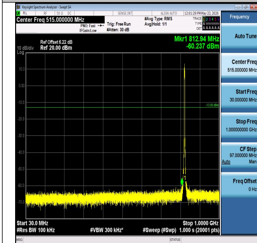
Band26(824-849)-3MHz-QPSK-26805-15RB#0-3 0~1000-PASS
