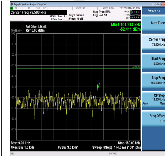
Band26(824-849)-3MHz-QPSK-26805-15RB#0-0 .009~0.15-PASS
