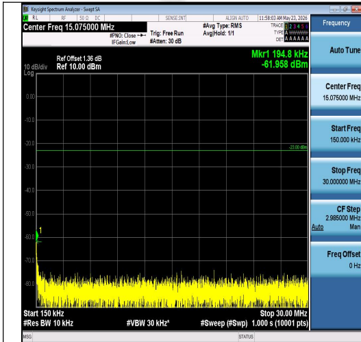
Band26(824-849)-3MHz-16QAM-26805-1RB#0-0.15~30-PASS
