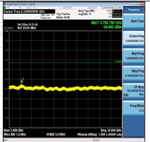
Band26(824-849)-3MHz-16QAM-26805-1RB#0-3000~10000-PASS
