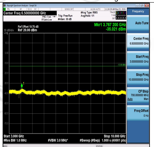
Band26(824-849)-1.4MHz-16QAM-27033-6RB#0 -3000~10000-PASS
