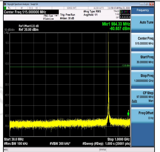
Band26(824-849)-3MHz-16QAM-26805-1RB#0-30~1000-PASS
