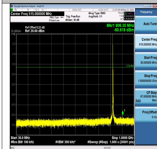
Band26(824-849)-3MHz-QPSK-26805-1RB#0-30 ~1000-PASS
