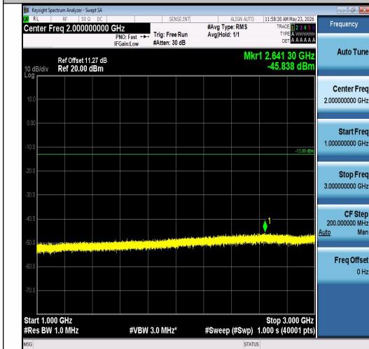
Band26(824-849)-3MHz-16QAM-26805-1RB#0-1000~3000-PASS
