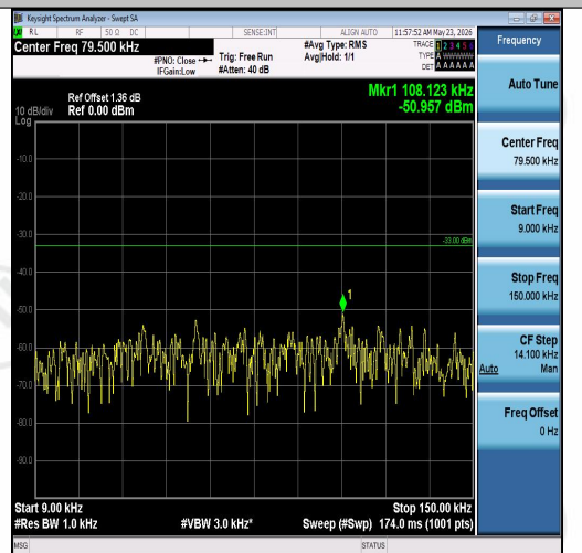
Band26(824-849)-3MHz-16QAM-26805-1RB#0- 0.009~0.15-PASS
