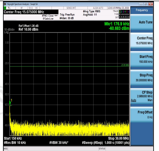
Band26(824-849)-3MHz-QPSK-26805-15RB#0-0 .15~30-PASS
